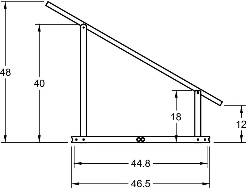
AnchorSpike hole-to-hole dimension: 44.8 inches
