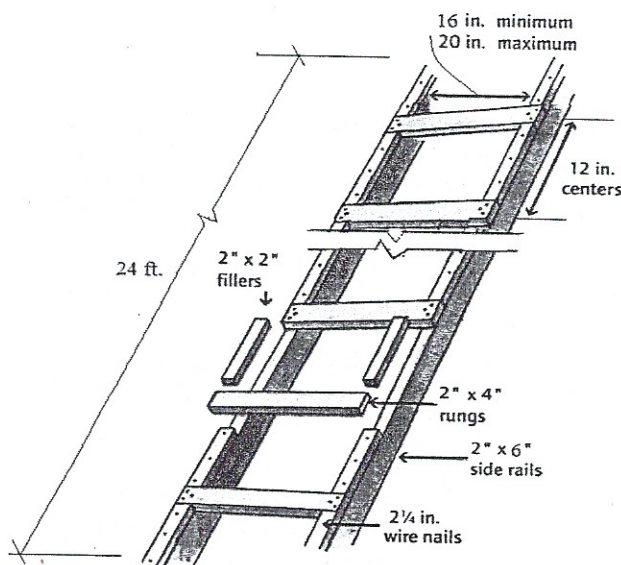
Figure 1: Single-Cleat Ladder
