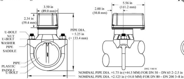
Fig. 6 Mounting Dimensions
