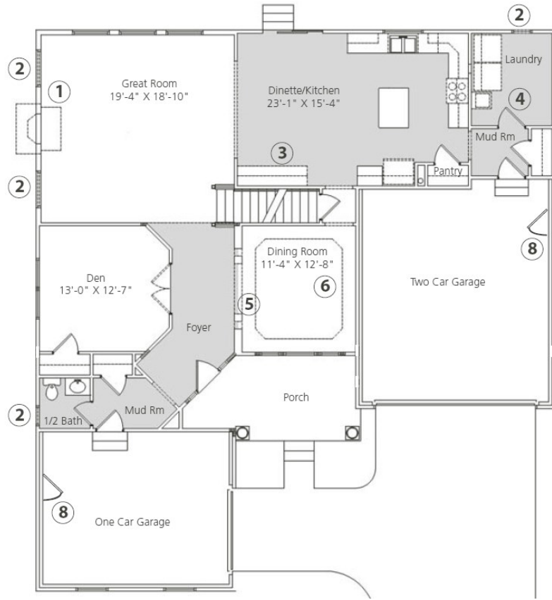
First Floor (Elevation "P")
