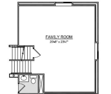
1st & 2nd Floor Plans Family Room / Lower Level Extension
