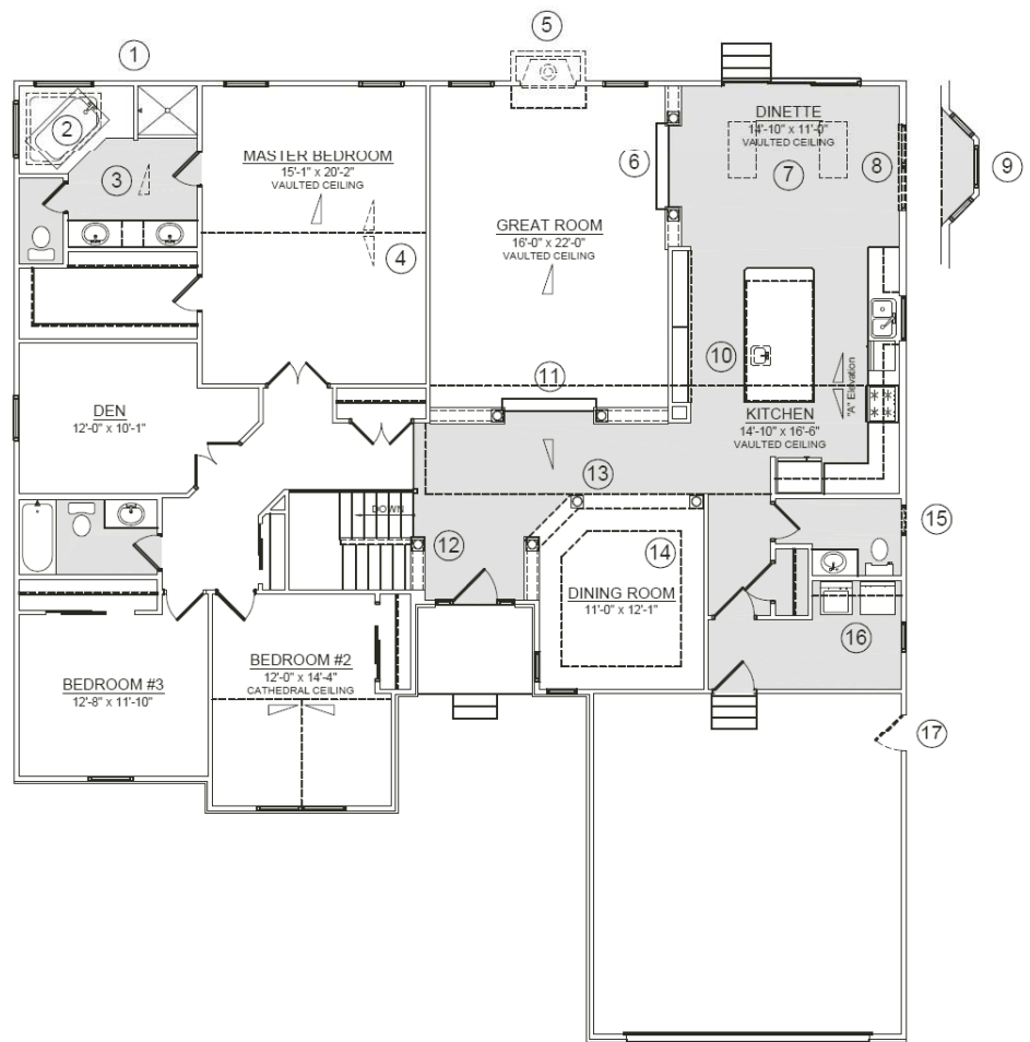
First Floor (Elevation "A")
