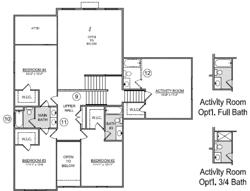
Second Floor (Elevation "A")
