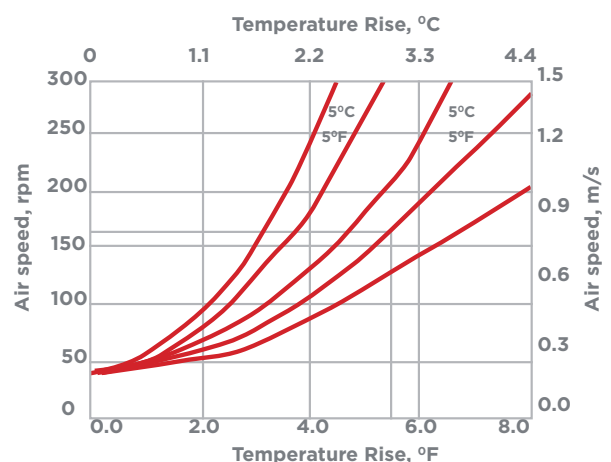
Air speed required to offset increased temperature.
