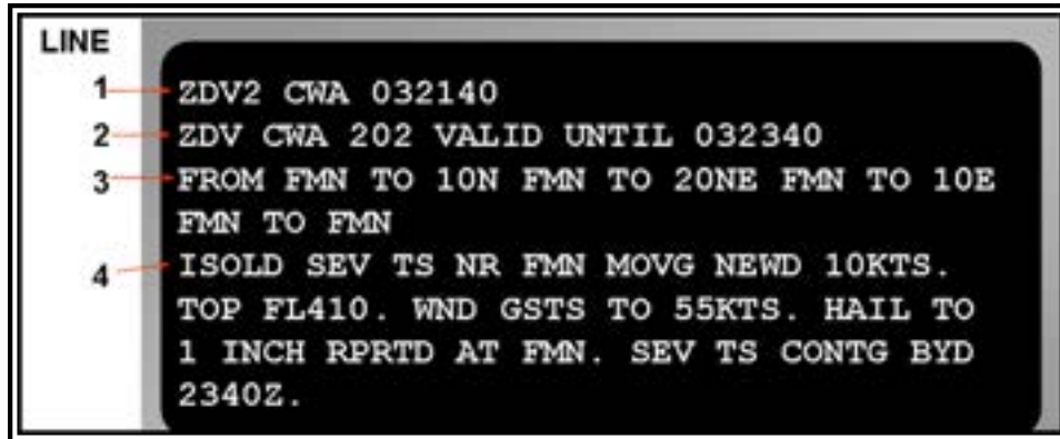
Figure 26-10. CWA—Example
