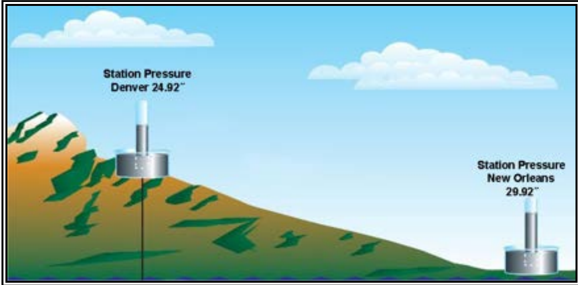
Figure 8-3. Station Pressure
