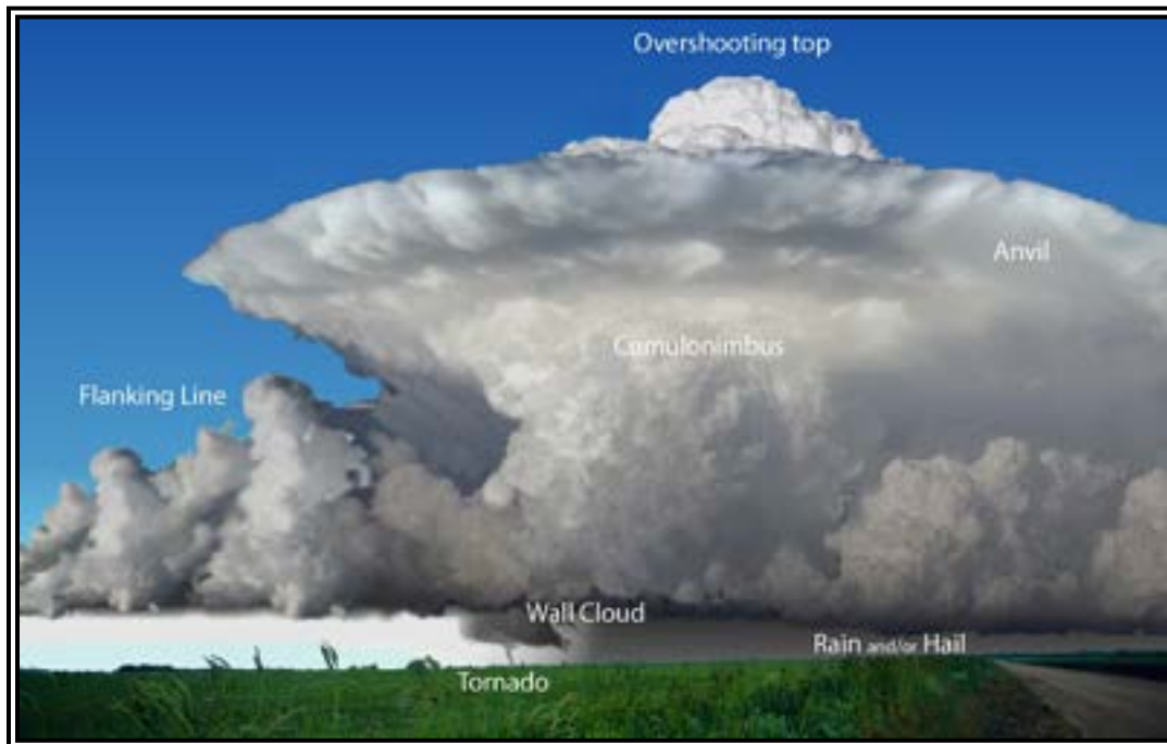
Figure 22-5. Supercell Thunderstorm
