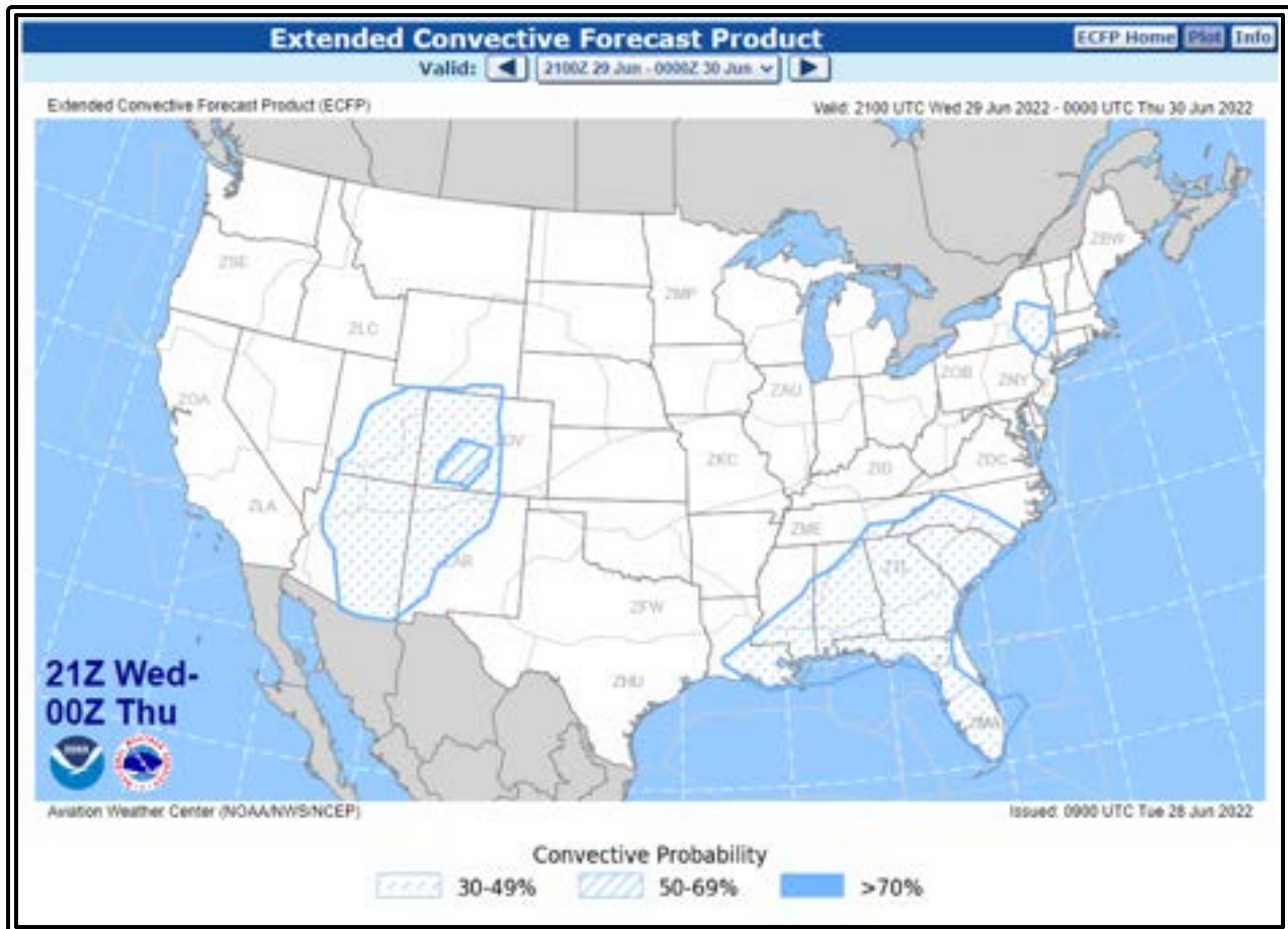
Figure 27-39. ECFP Example
