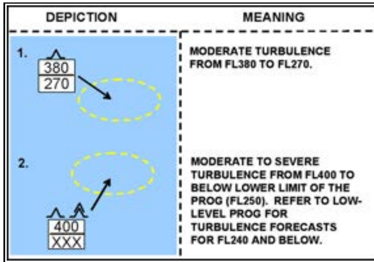
Figure 27-23. High-Level SIGWX Chart Turbulence—Examples
