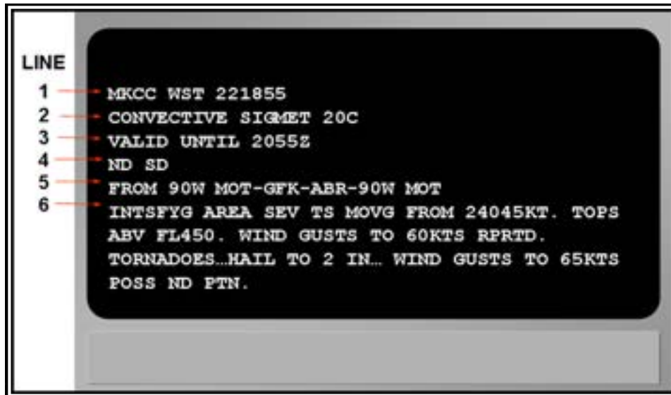
Figure 26-6. Convective SIGMET—Example
