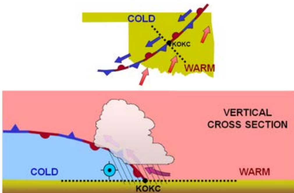
Figure 11-7. Stationary Front
