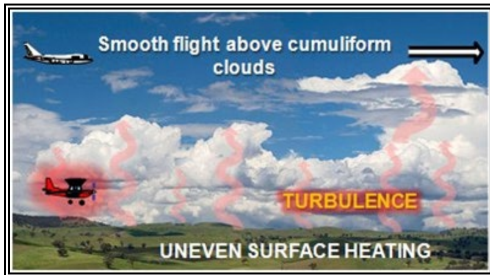
Figure 19-1. Convective Turbulence
