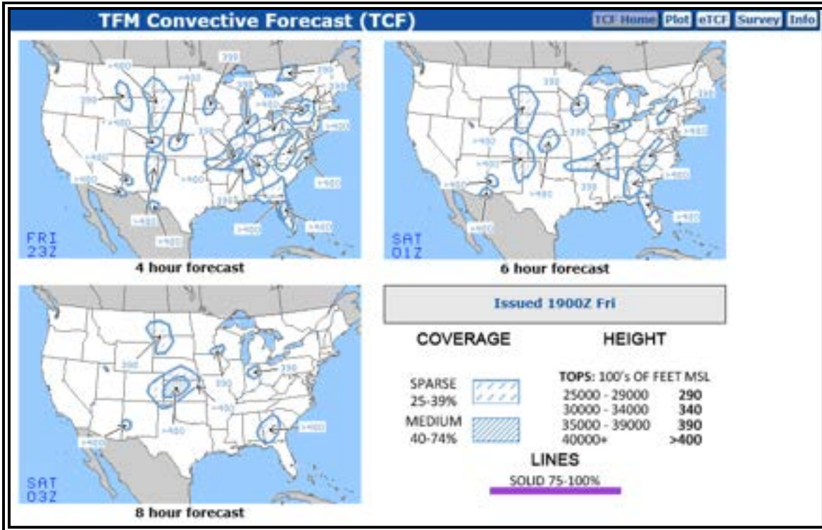
Figure 27-38. TCF Example
