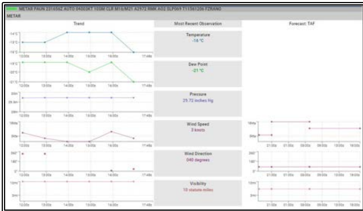
Figure 24-38. Weather Trends Example at Unalakleet (PAUN), Alaska
