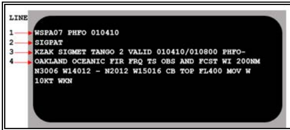
Figure 26-7. SIGMET Outside the CONUS—Example
