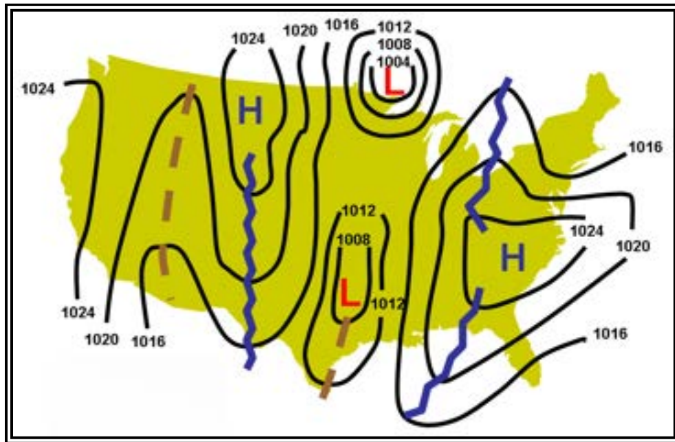
Figure 25-5. Schematic of Surface Chart Pressure Patterns
