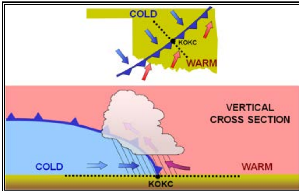
Figure 11-6. Cold Front
