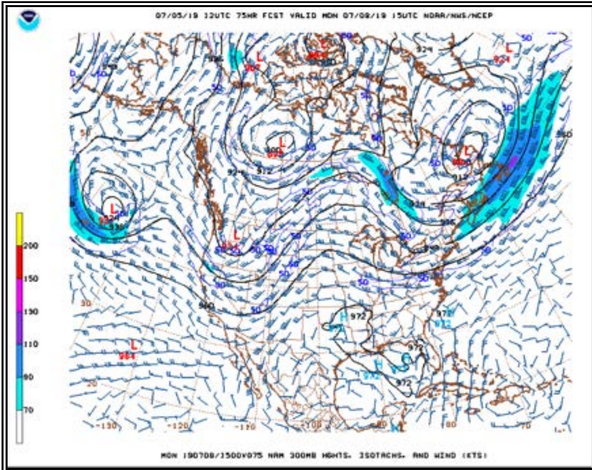
Contours of the height of the 300 mb surface are presented as solid lines. Windbarbs are used to show the direction and speed of the wind. Shading is done for wind speeds greater than 70 kt and generally represents the jet stream.
