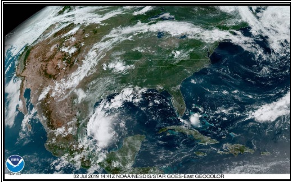
Figure 24-21. GeoColor Satellite Image—U.S. Example
