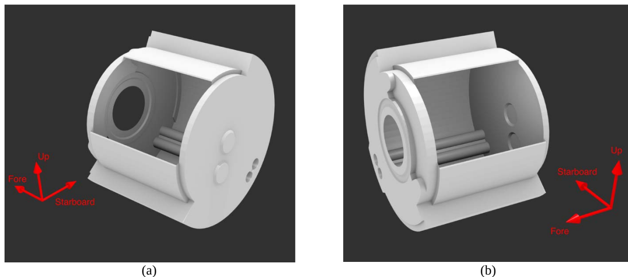
Figure 8. Isometric view of the SOFIA cavity.
