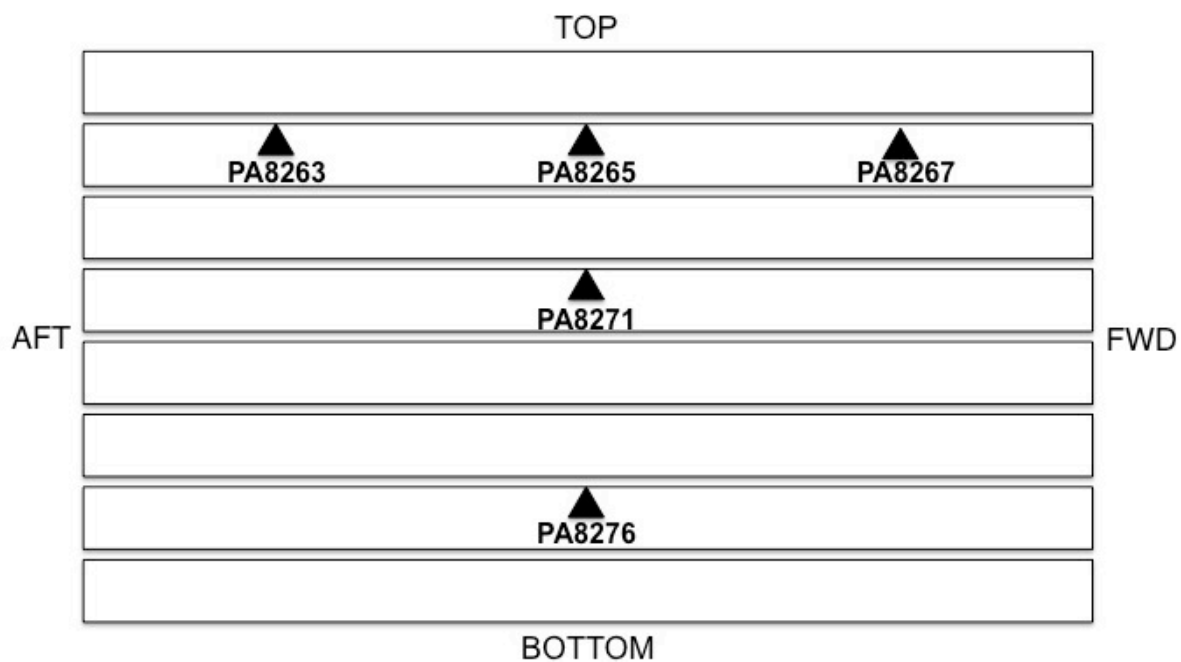
Figure 13. Internal lower flexible door sensor locations.
