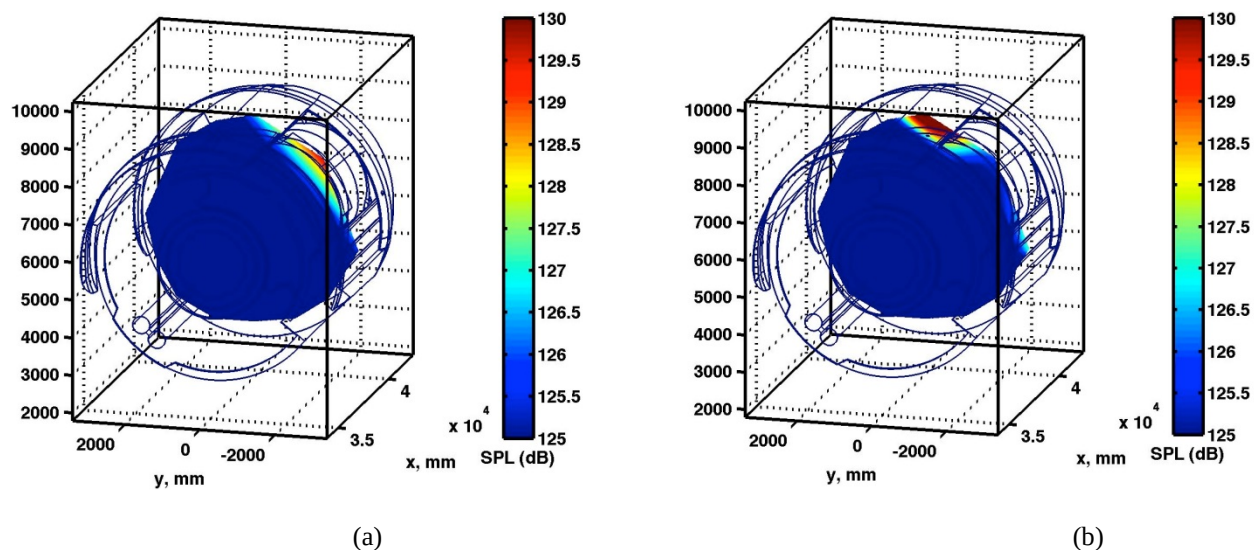
Figure 15. Cavity aft bulkhead hot spot at the nominal science observation flight condition. (a) Aperture assembly = 30° and (b) 57°.
