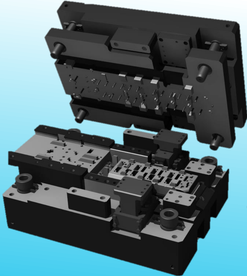
Sample 3D Die Design for Progressive die
