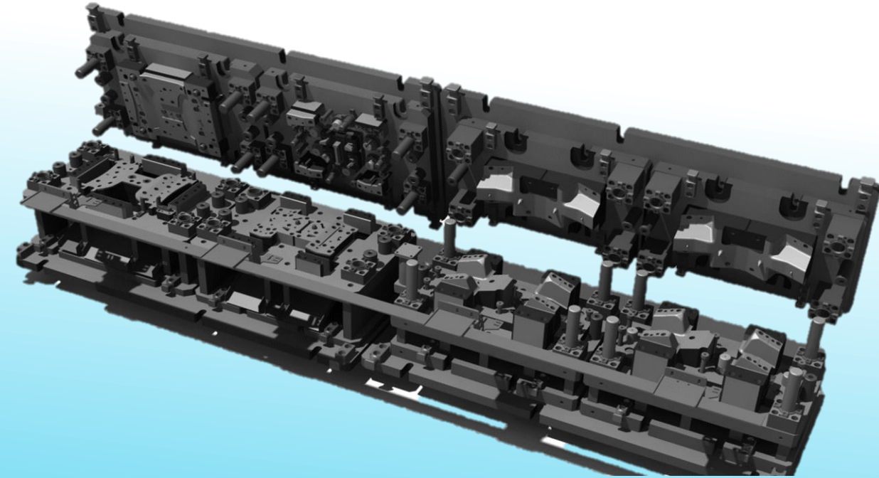
Sample 3D Die Design for Transfer line
