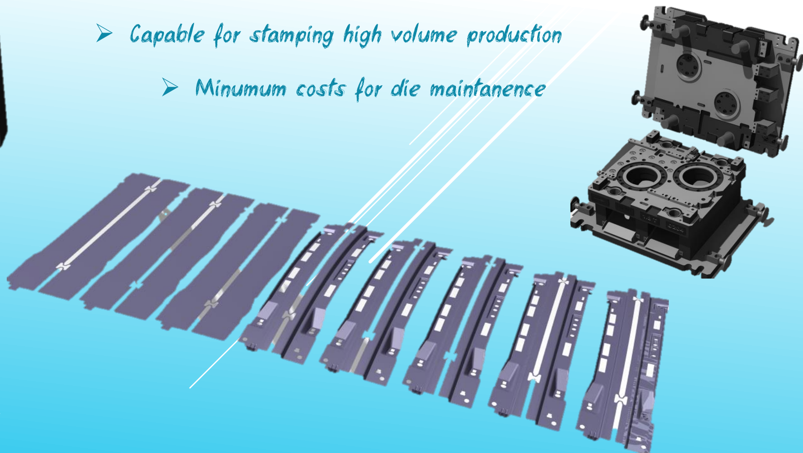
Sample 3D Die Design for Progressive die
