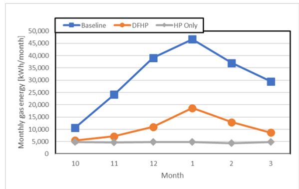
Figure 16 Monthly site energy consumption (Gas)
