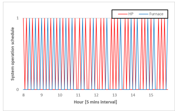
Figure 13 Heating system operation from 8 a.m. to 4 p.m.
