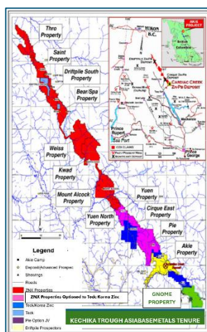
Gnome Project location in the Kechika Trough, British Columbia
