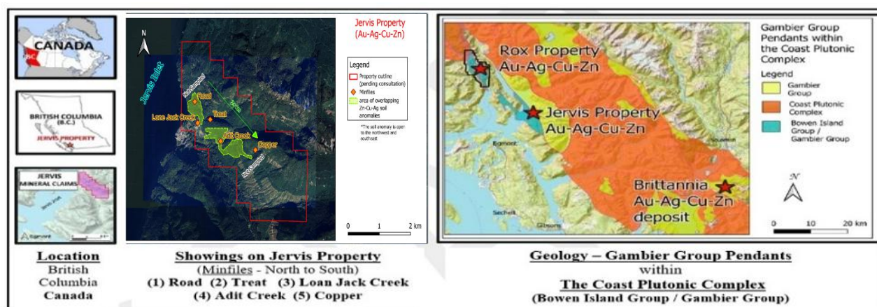
Jervis Project — location and geological setting along the VMS-prospective Gambier Group trend.
