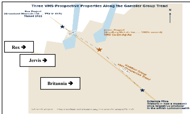
Britannia, Jervis, and Rox VMS-prospective properties along the Gambier Group trend.
