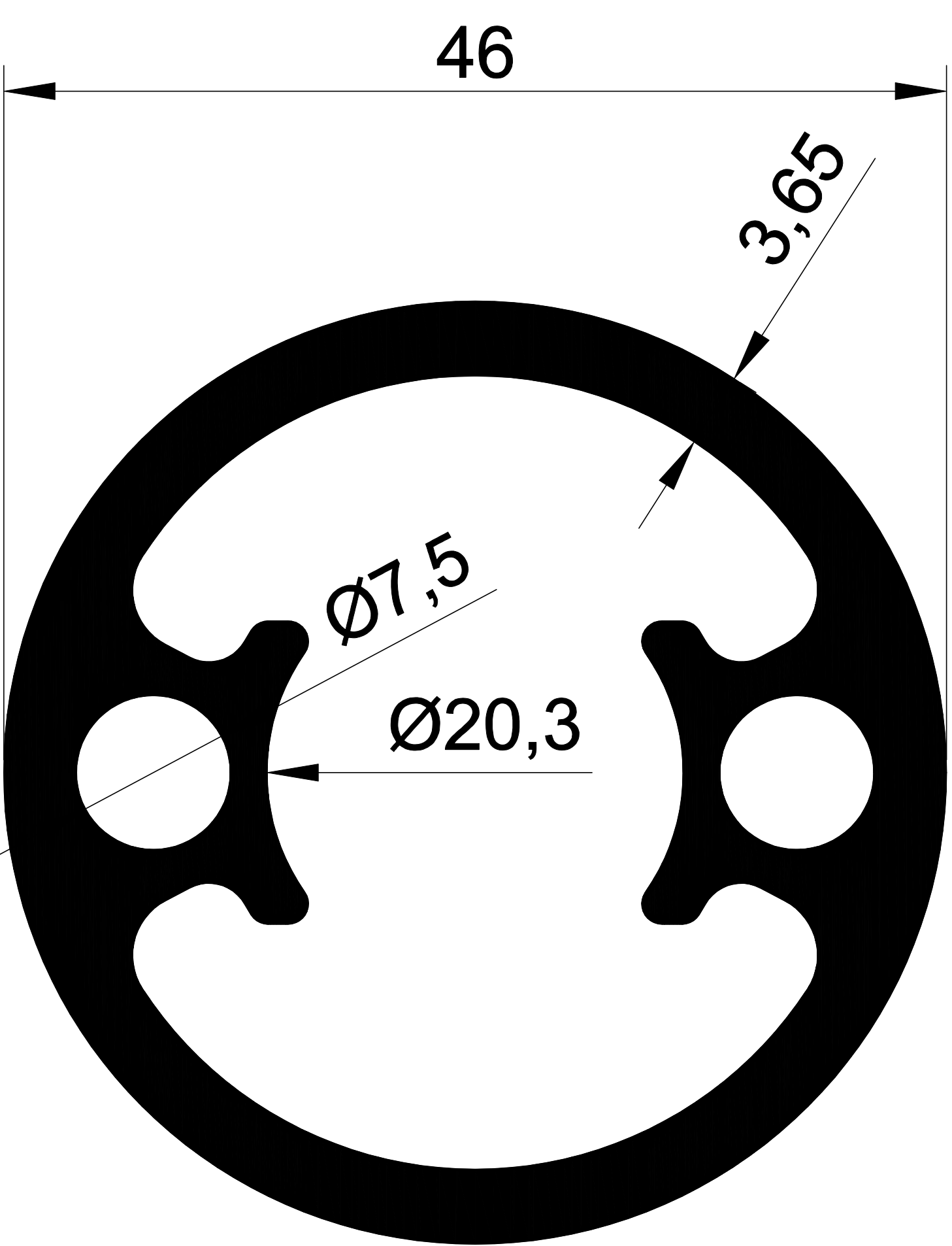
1029 1,780 Kg/m.
