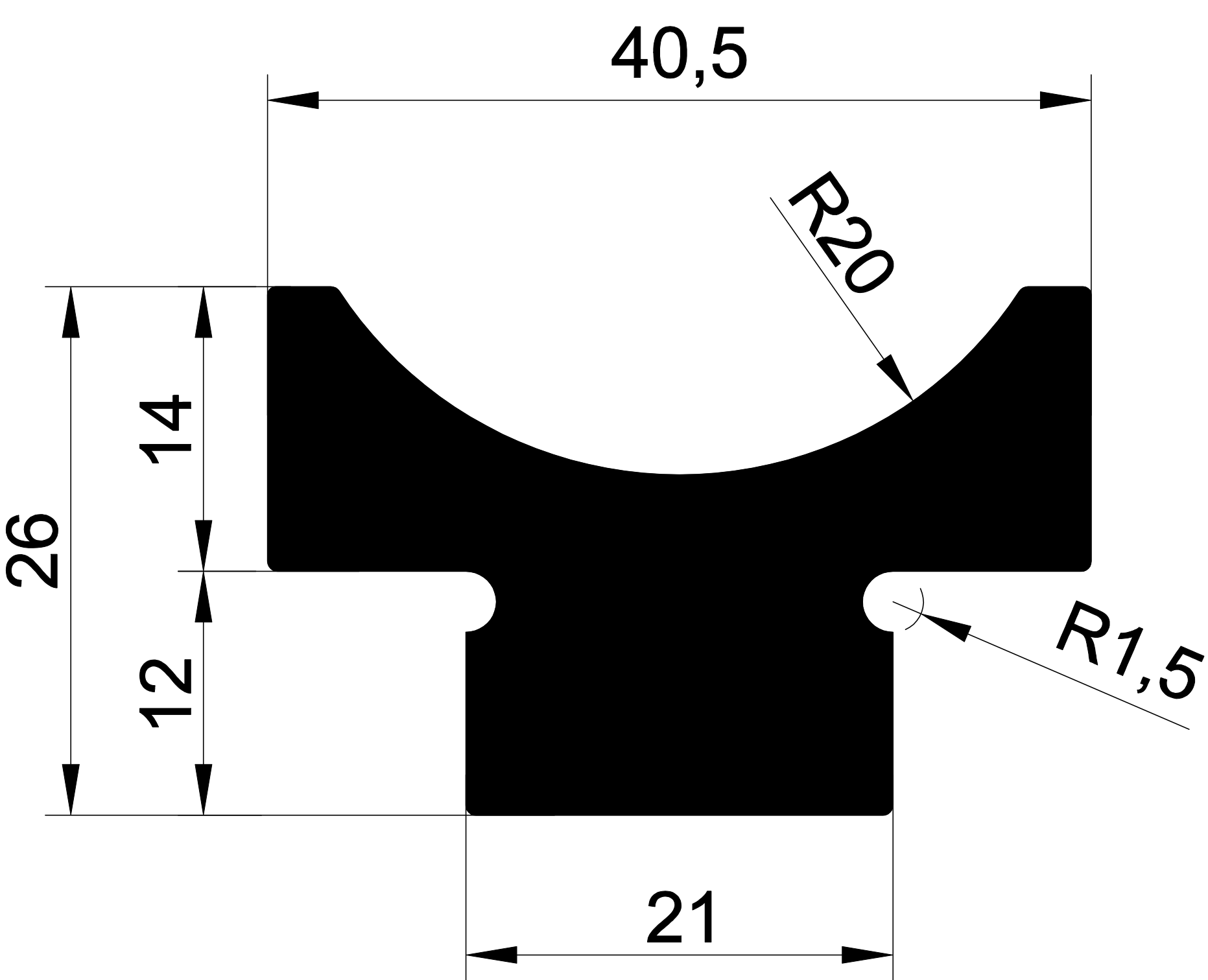
1026 1,602 Kg/m.
