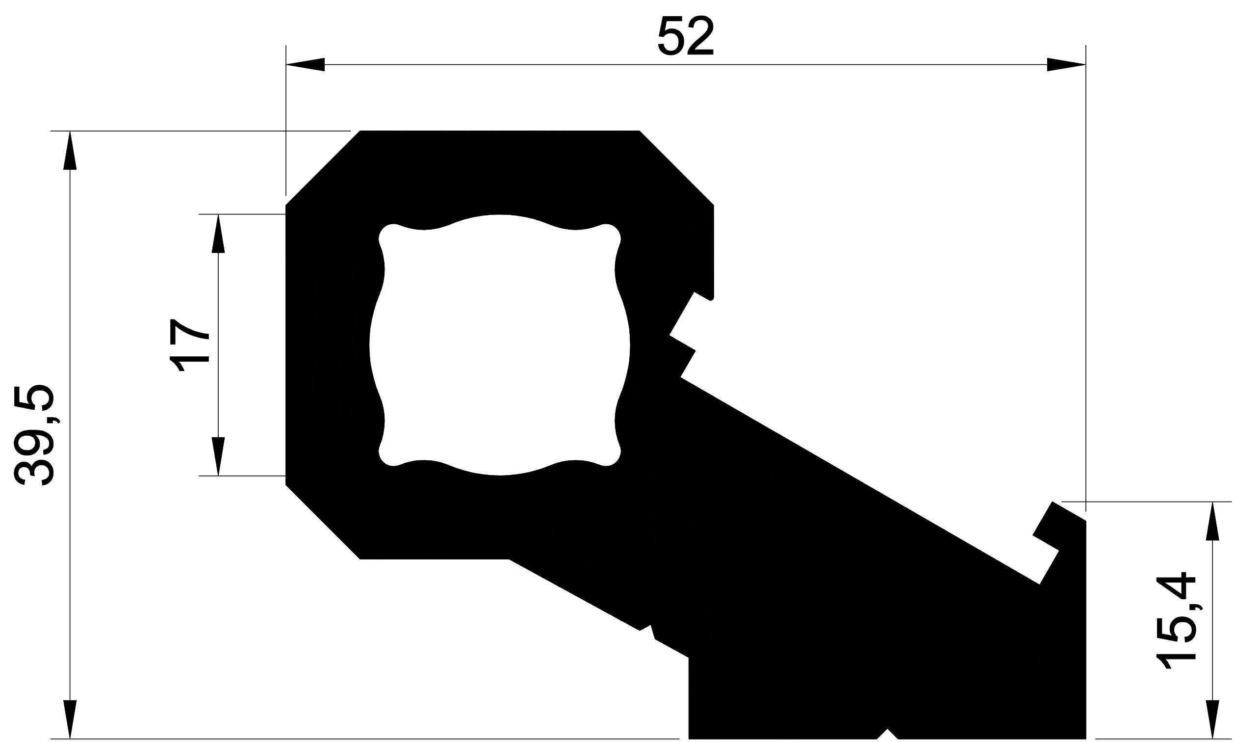
1236 2,480 Kg/m.
