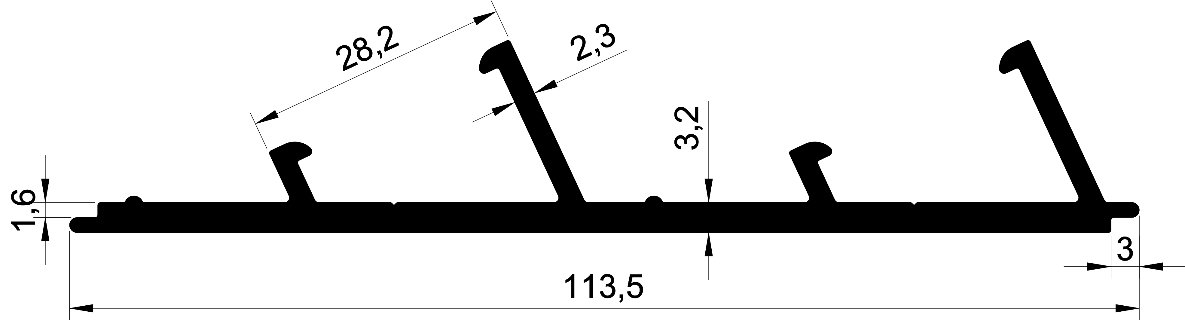
1432 1,311 Kg/m. MENFEZ KASA
