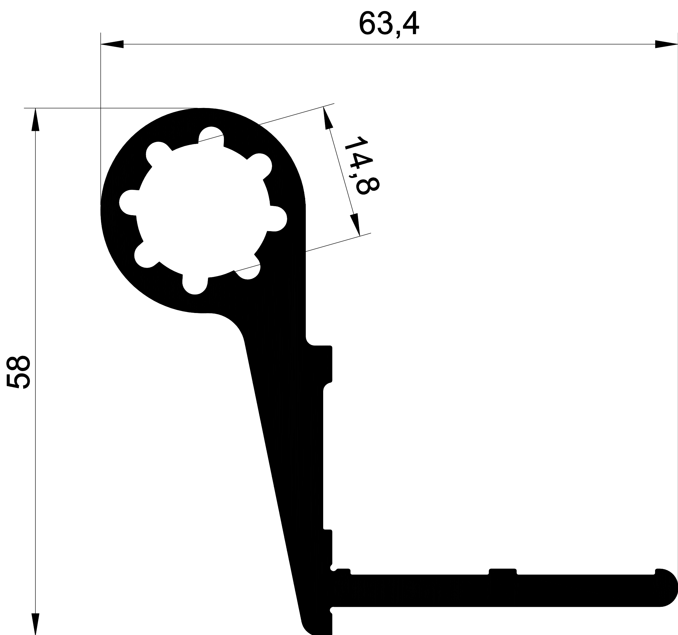
1011-B 1,521 Kg/m.
