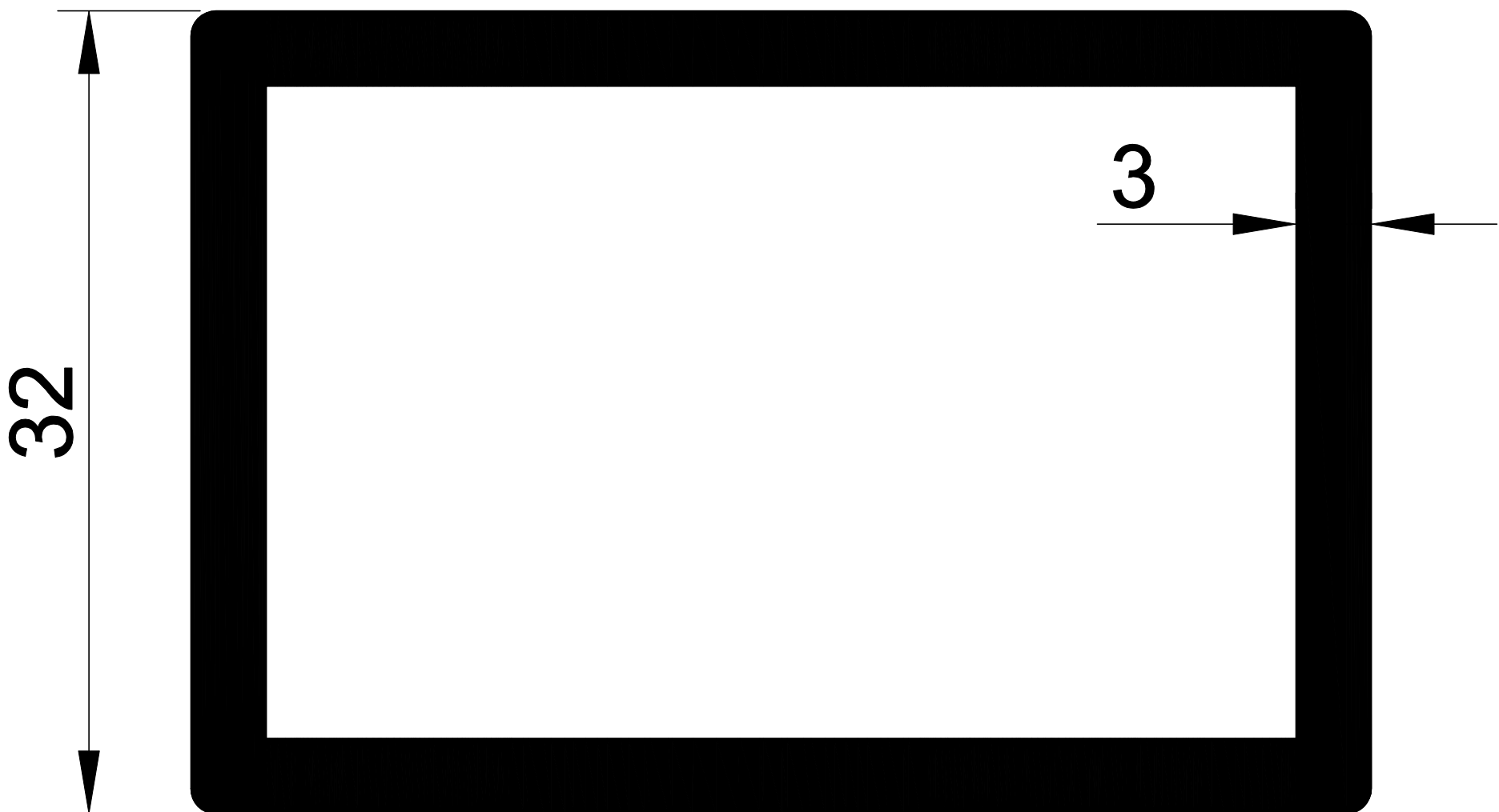
1277 1,184 Kg/m.
