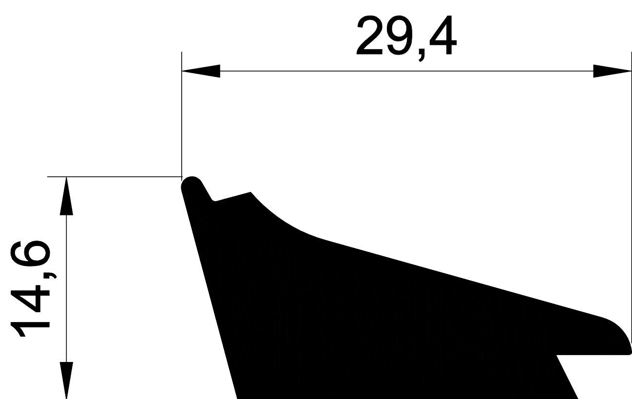
1219 1,976 Kg/m.
