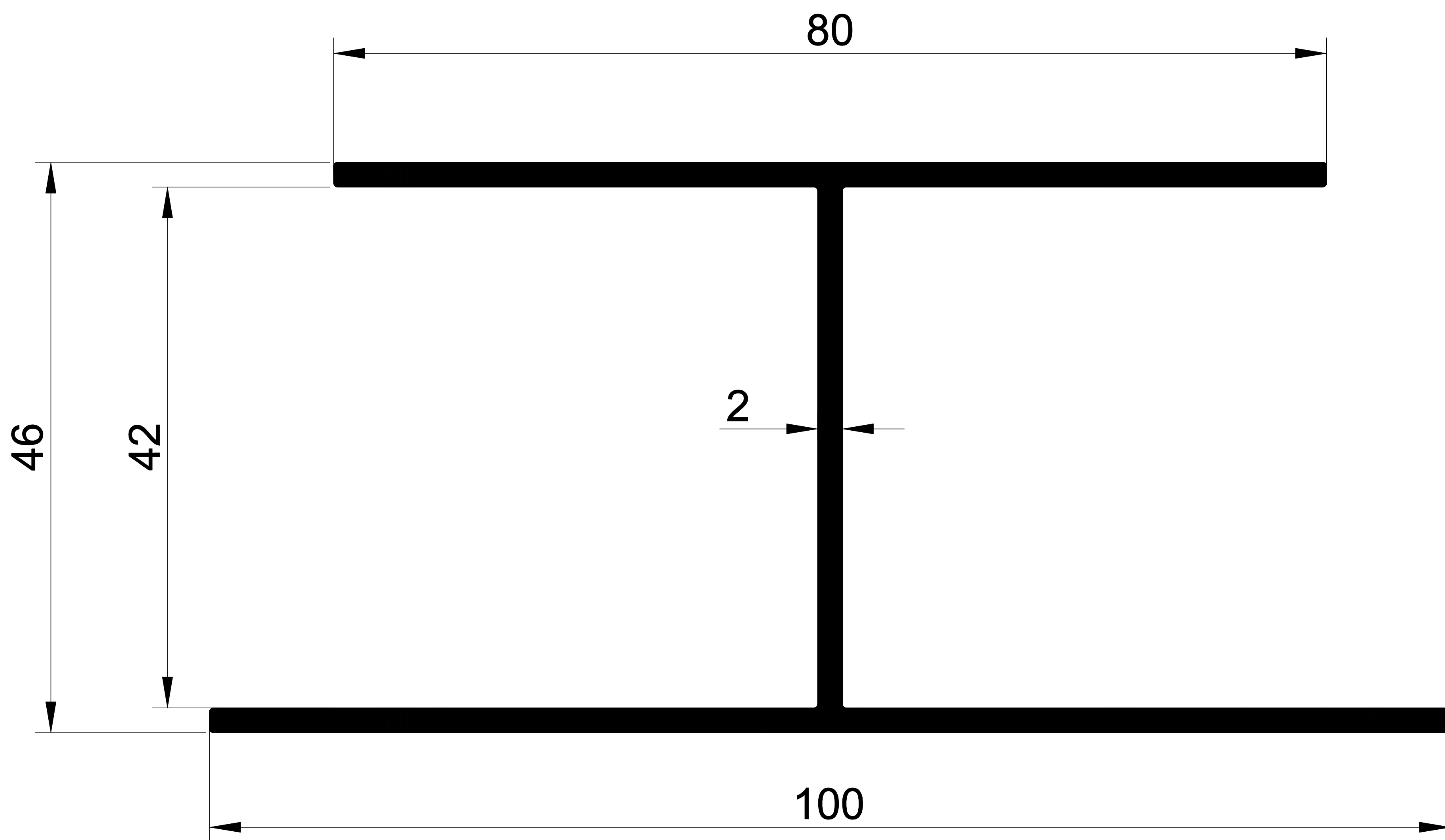
1447 1.203 Kg/m. PANEL H PROFİLİ
