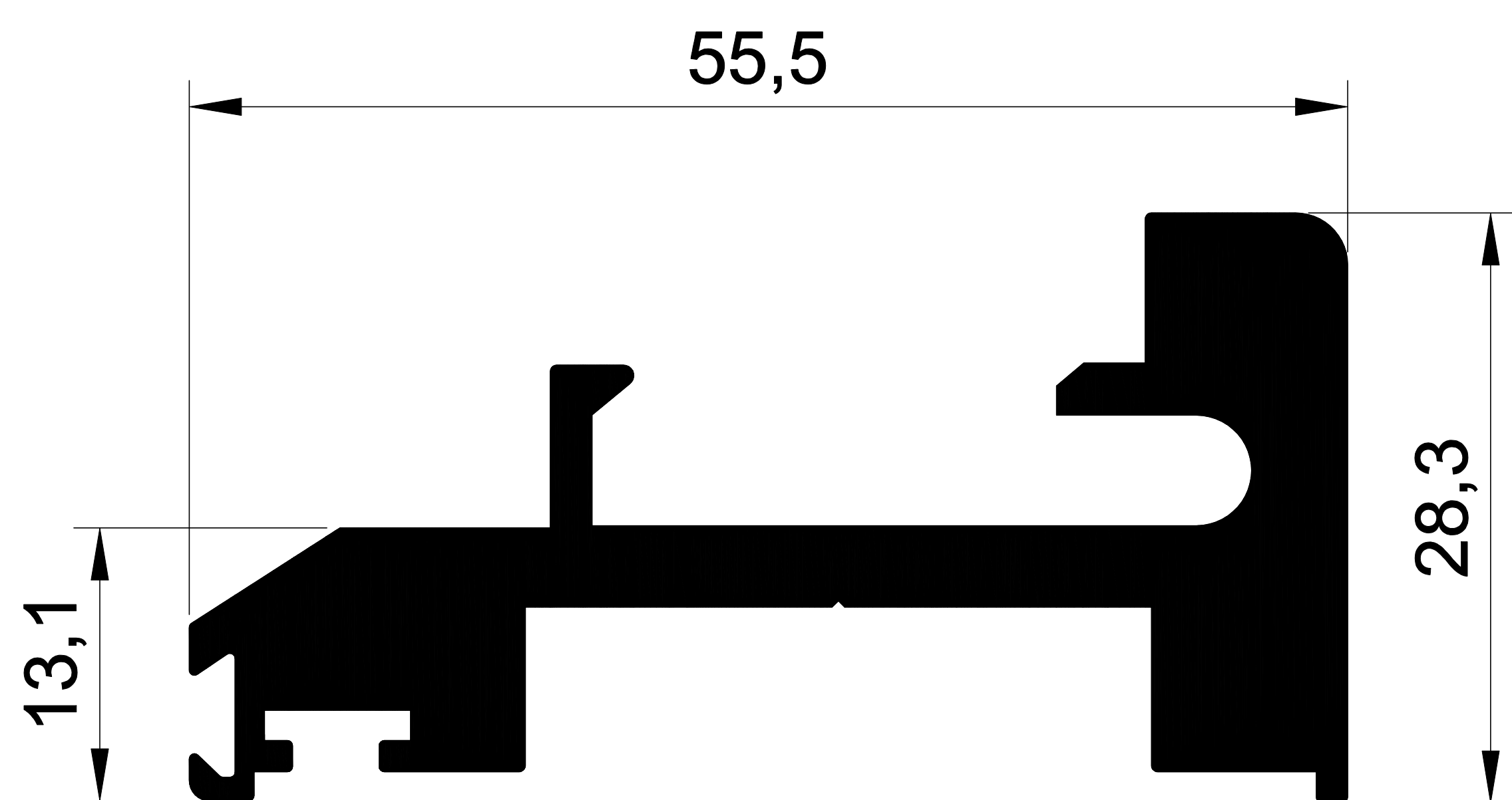
1209 1,428 Kg/m.
