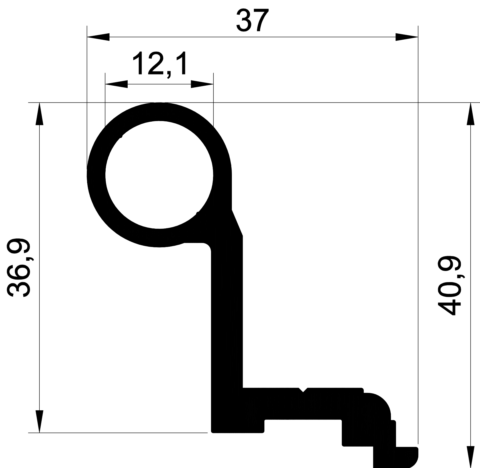
1260 0,721 Kg/m.
