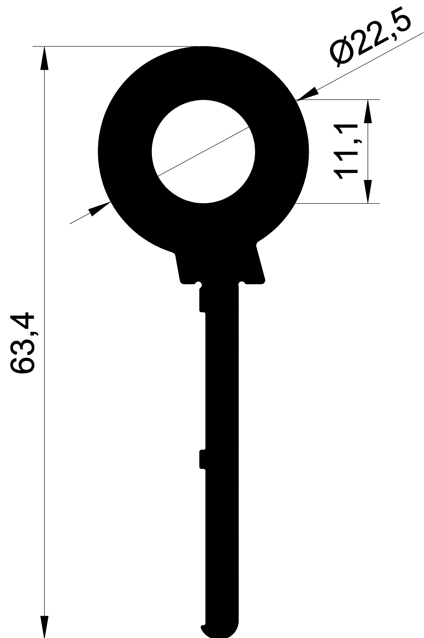
1010-B 1,261 Kg/m.
