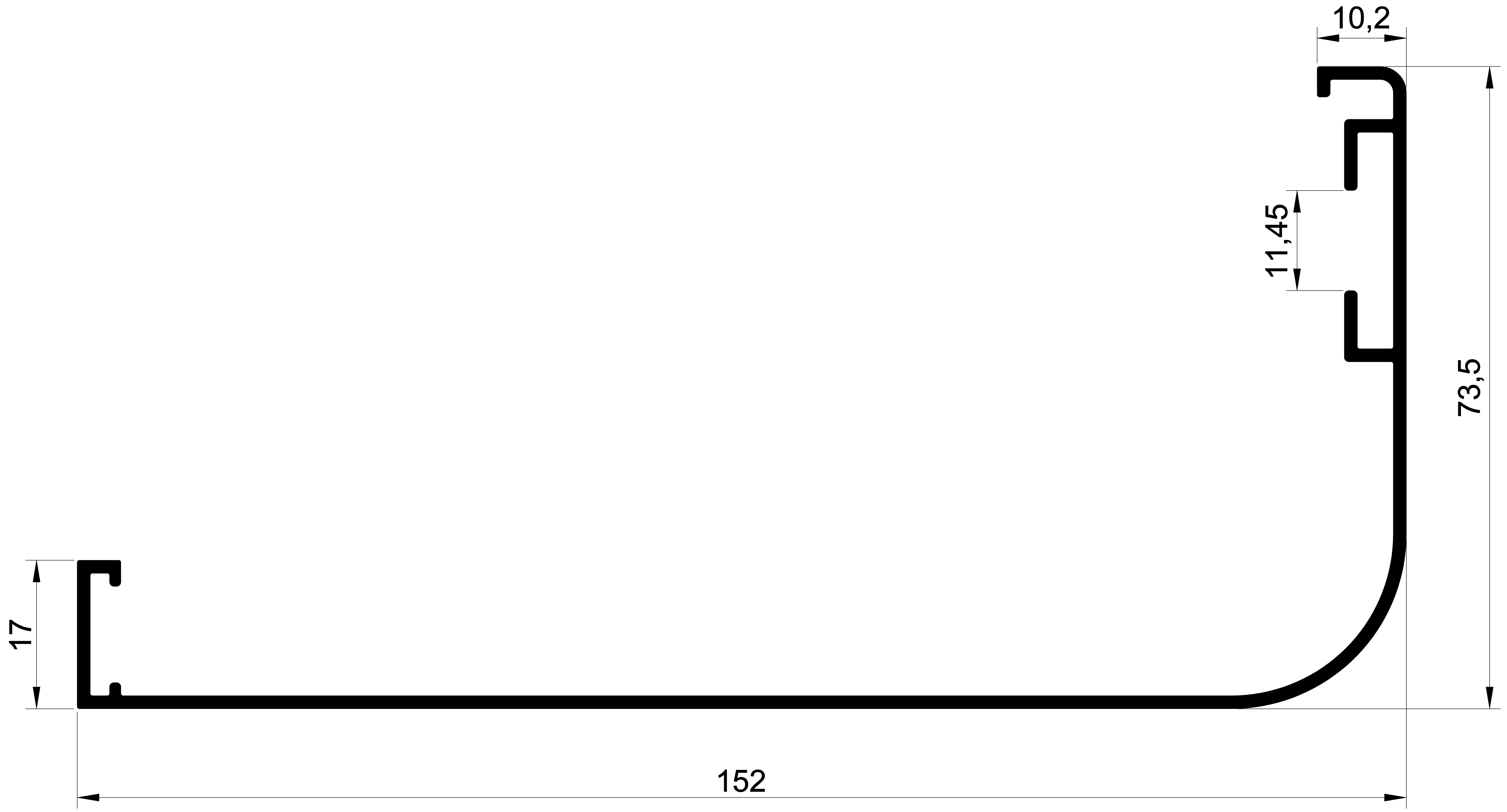
1425 1,102 Kg/m. MS-152'LİK PEERVAZ
