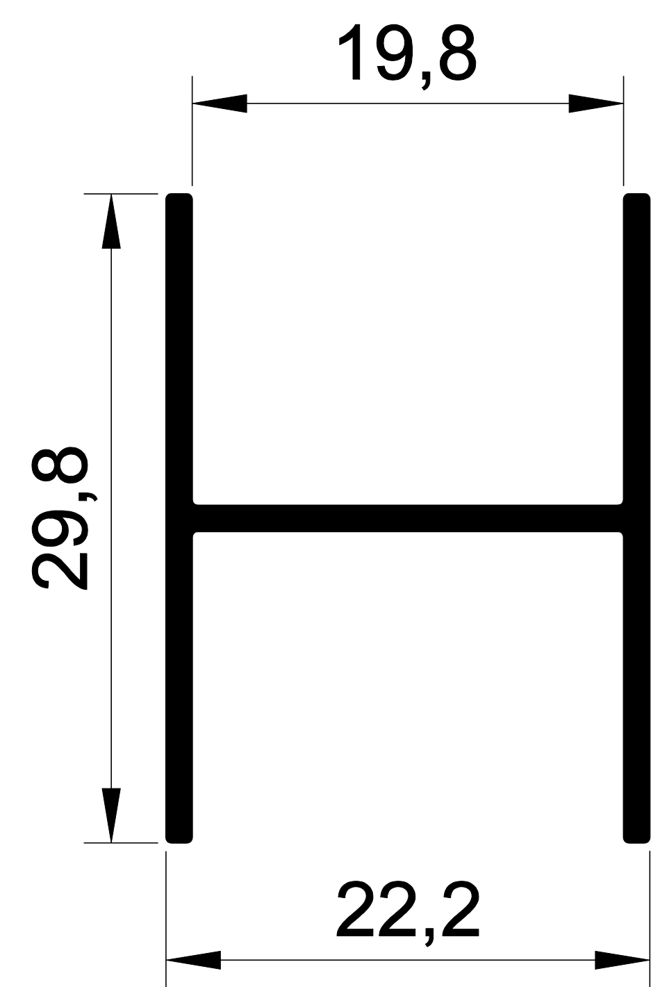
1411 0,257 Kg/m. MOBİLYA H PROFİLİ
