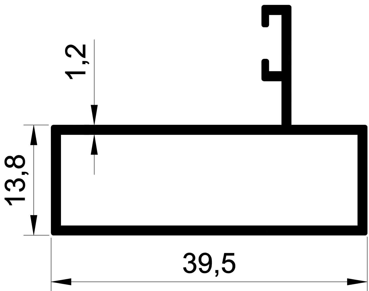
1145 0,404 Kg/m. GOLD DİKME
