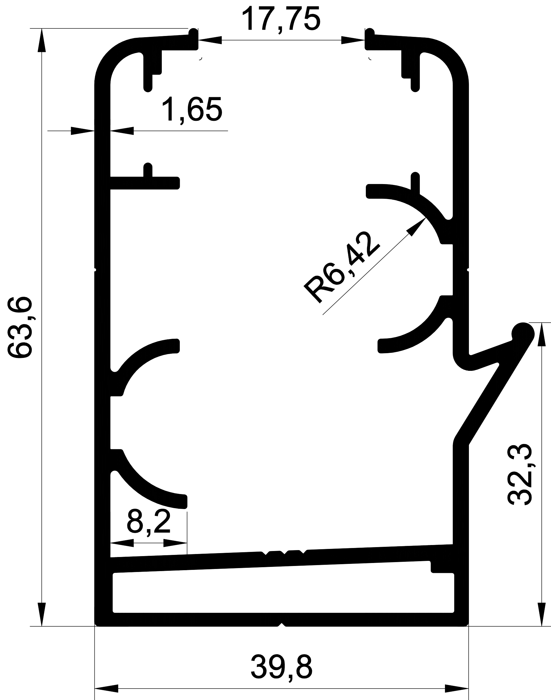
1456 1,222 Kg/m. GOLD ORTADAN DAMLALIKLI KASA-1.65 mm
