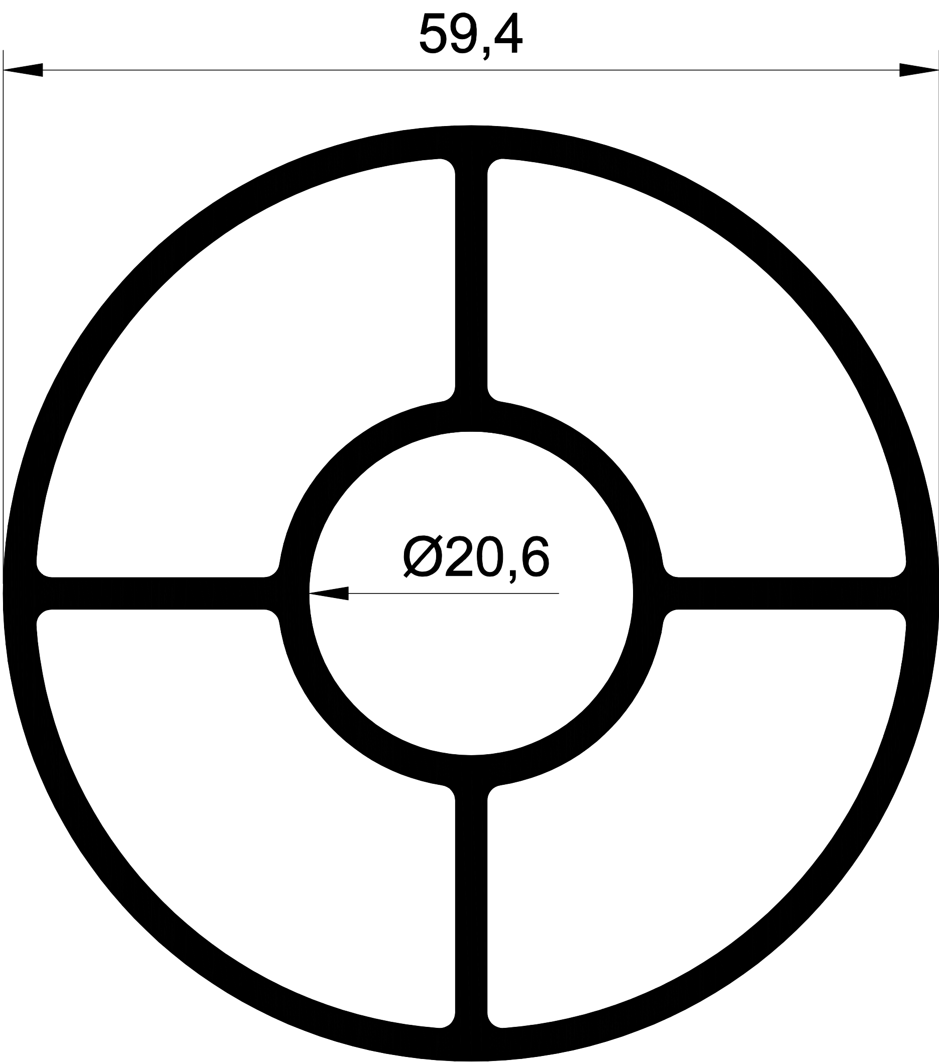
1256 1,705 Kg/m.
