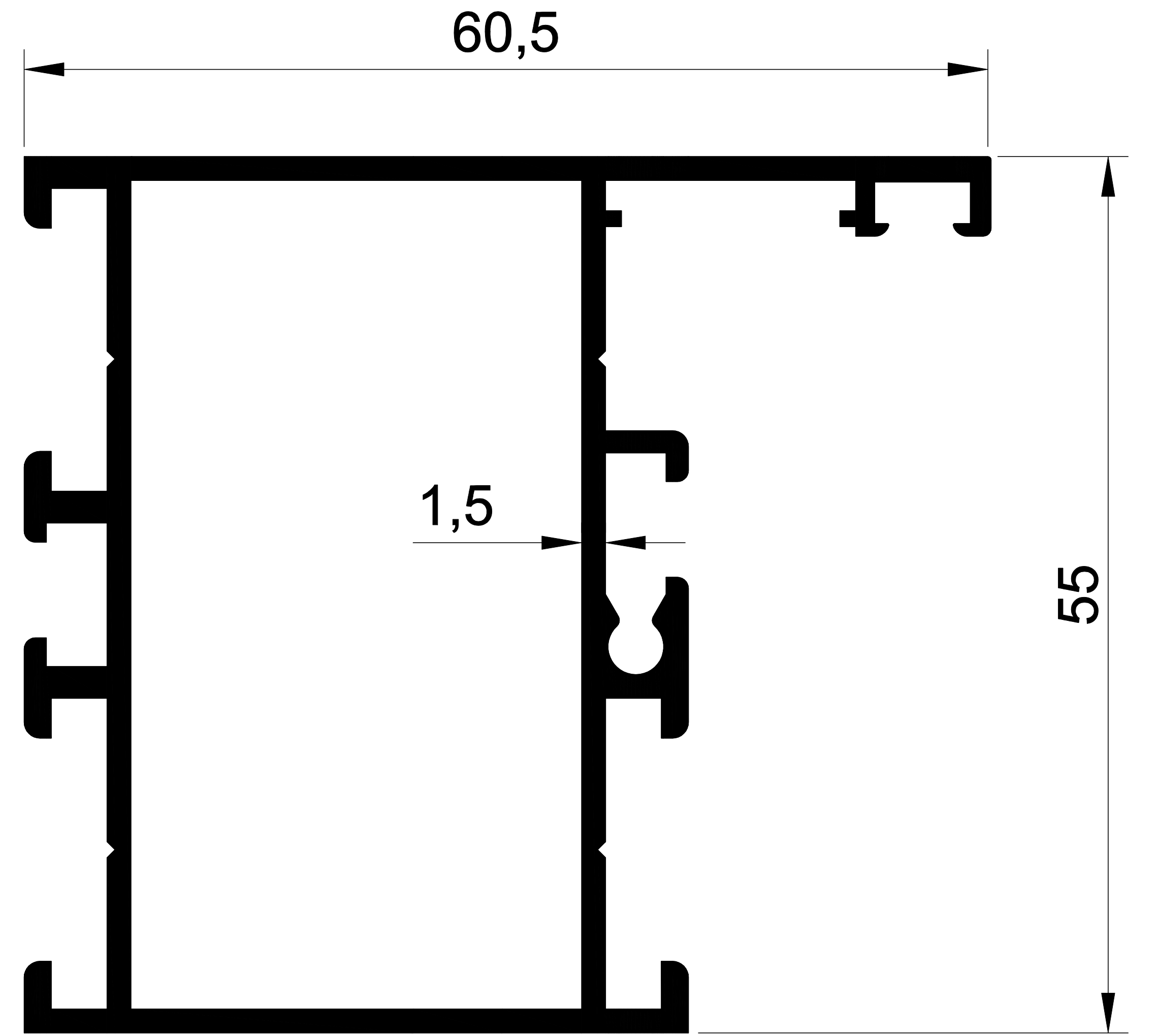
1200 1,098 Kg/m. SİSTEM KASA
