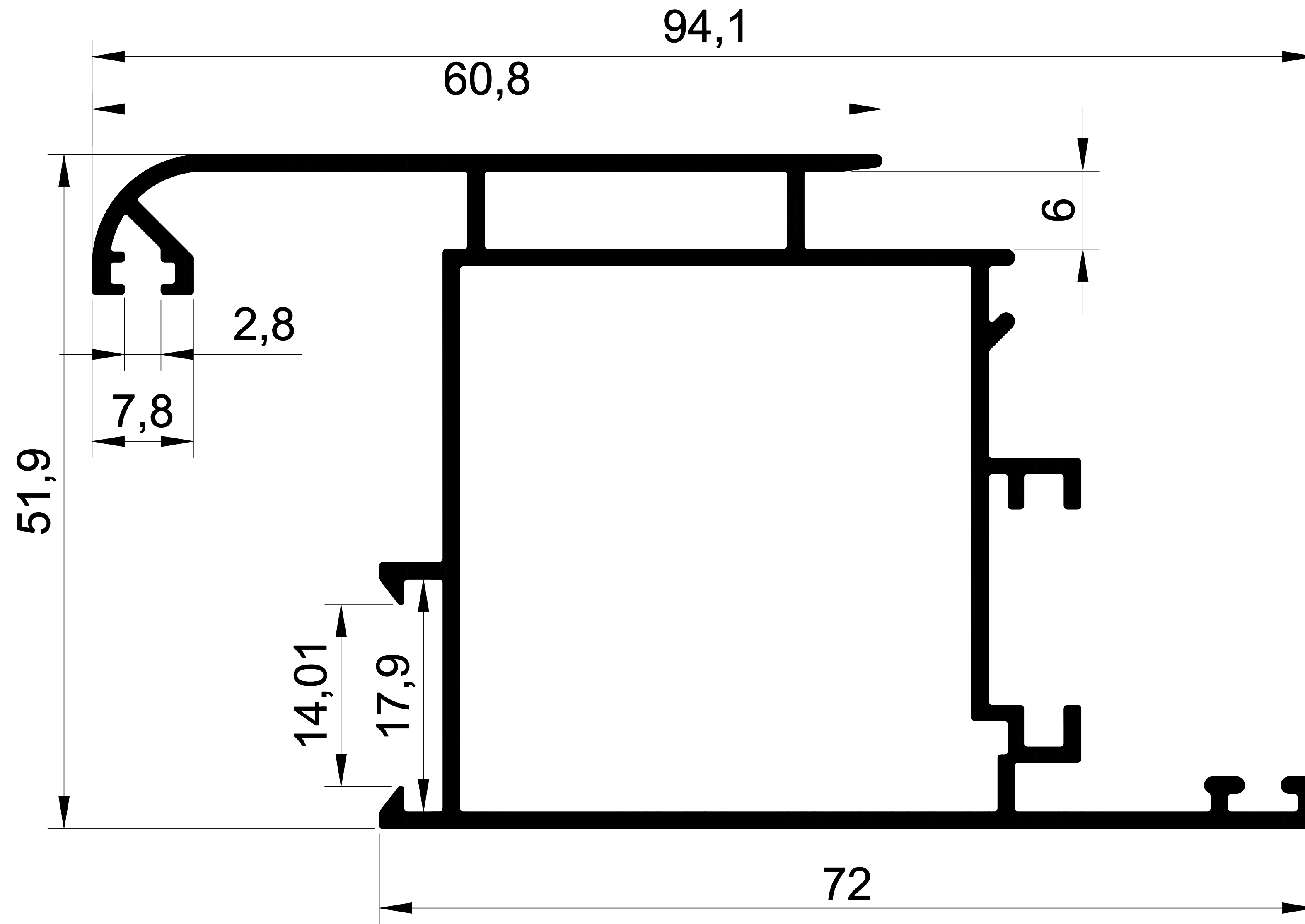
1371 1,164 Kg/m. OVAL KANAT
