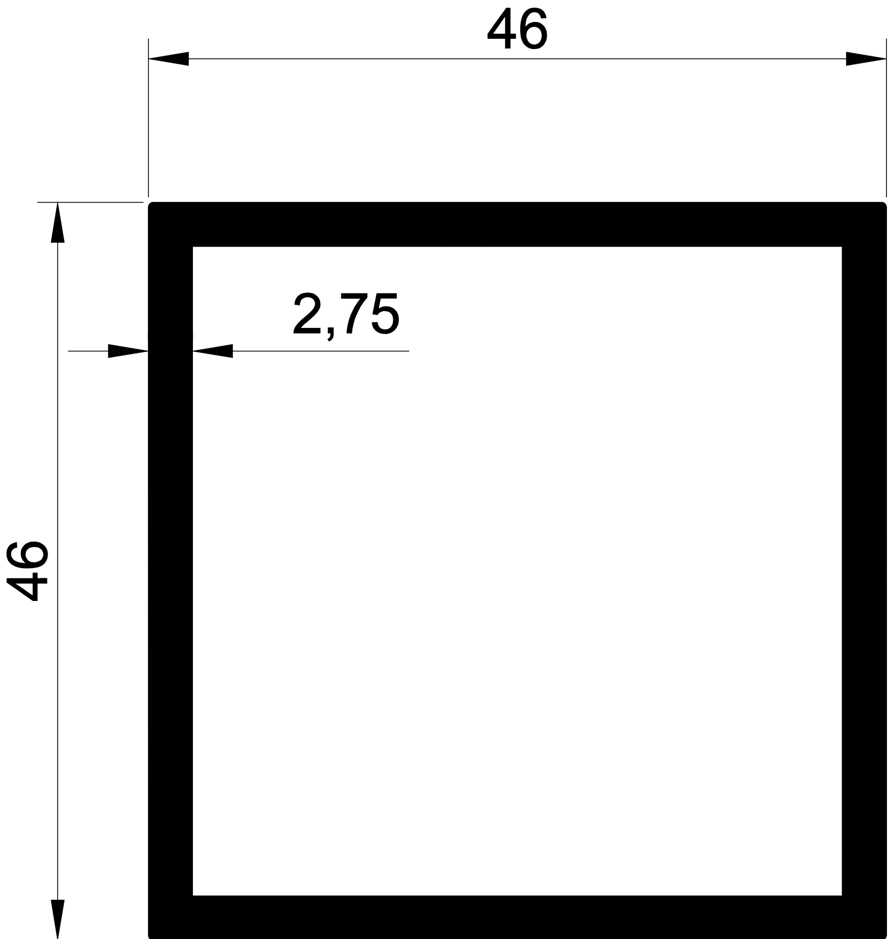
1049-B 1,289 Kg/m.
