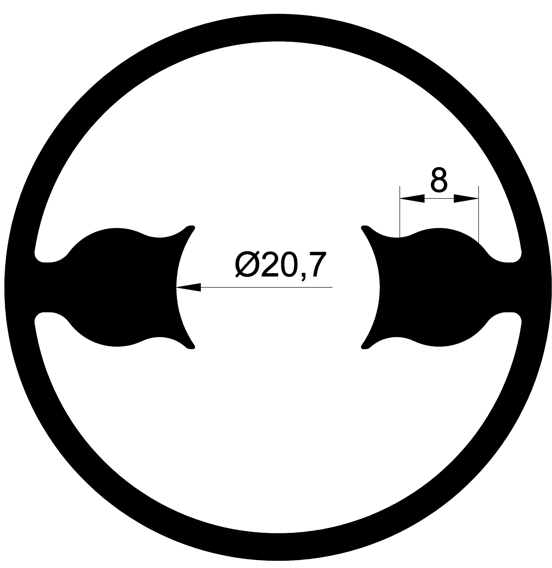
1017-B 1,743 Kg/m.
