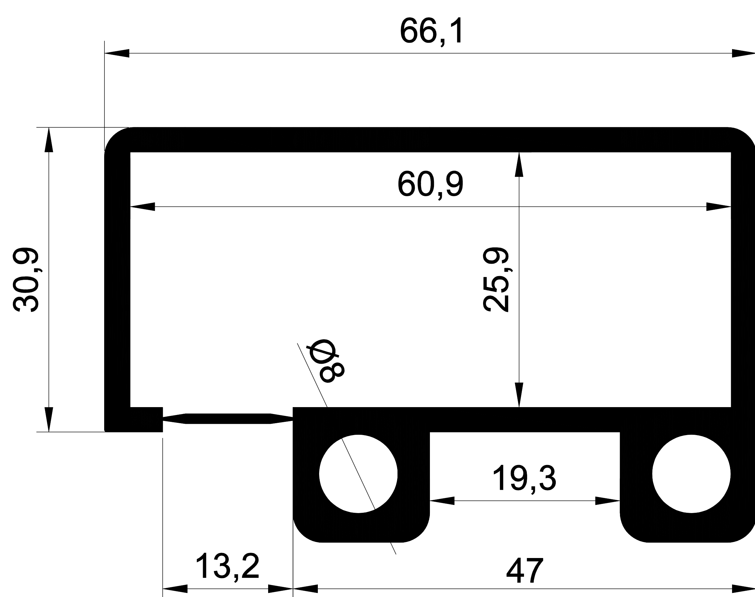
1283 1,740 Kg/m.
