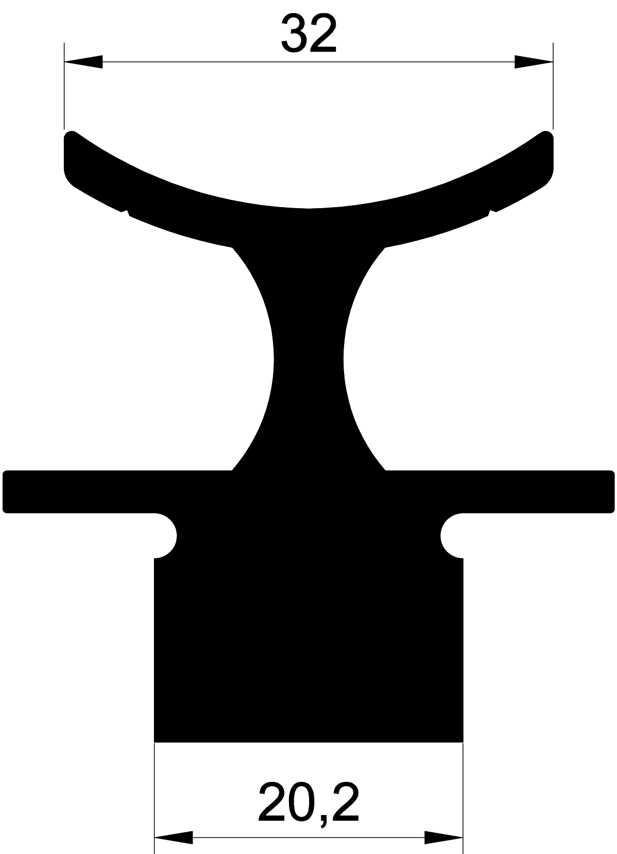
1172 1,615 Kg/m.
