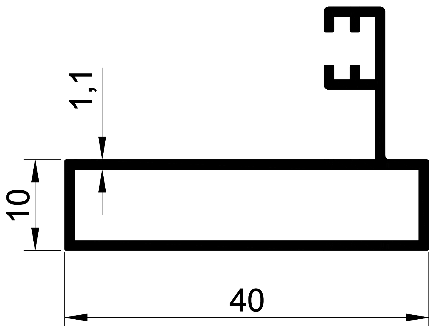
1341 0,388 Kg/m. 10 mm GOLD DİKME
