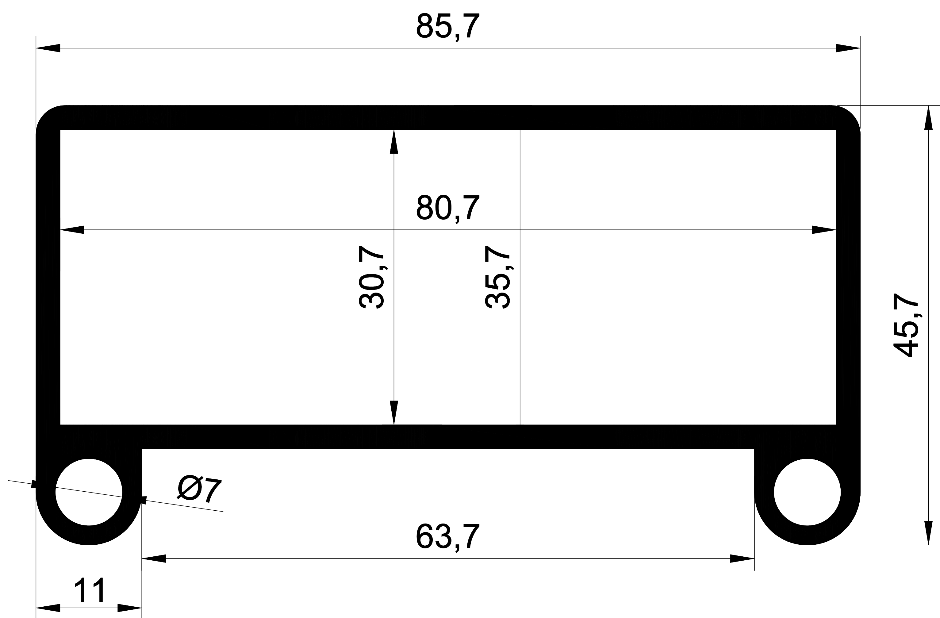
1045 1,883 Kg/m.
