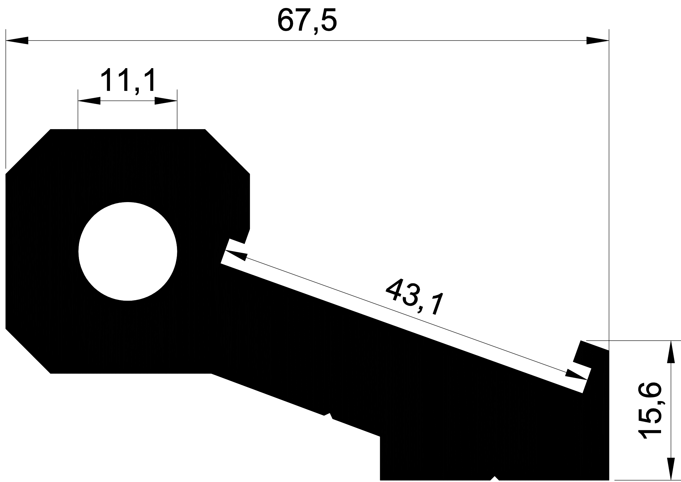
1238 3,111 Kg/m.
