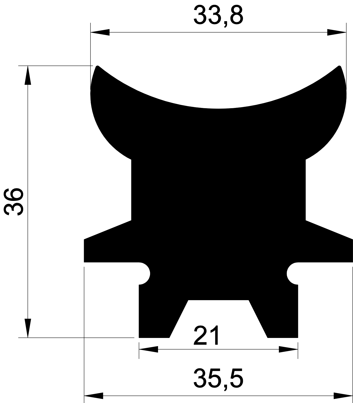
1012 2,122 Kg/m.
