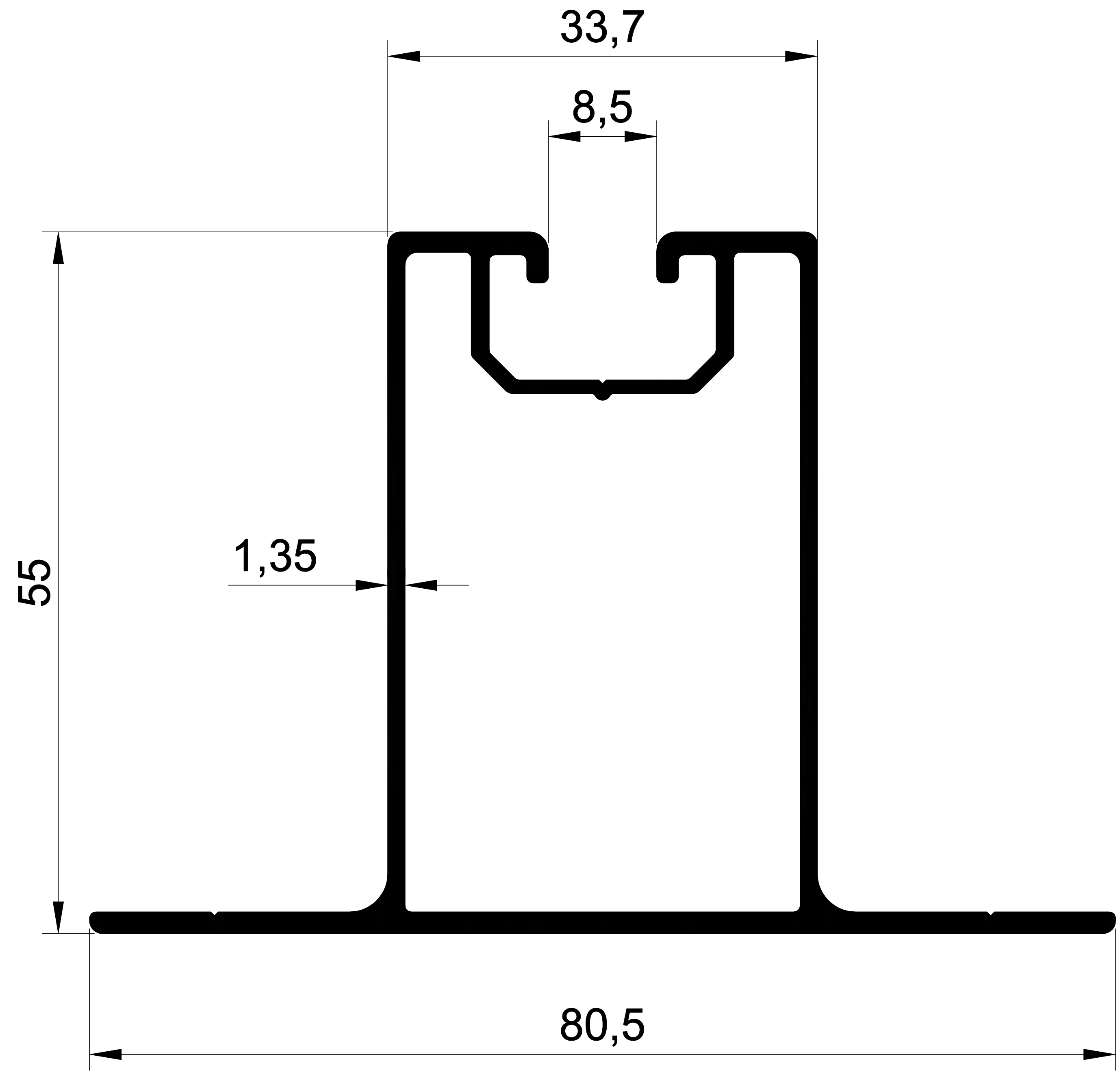
1214 1,016 Kg/m.
