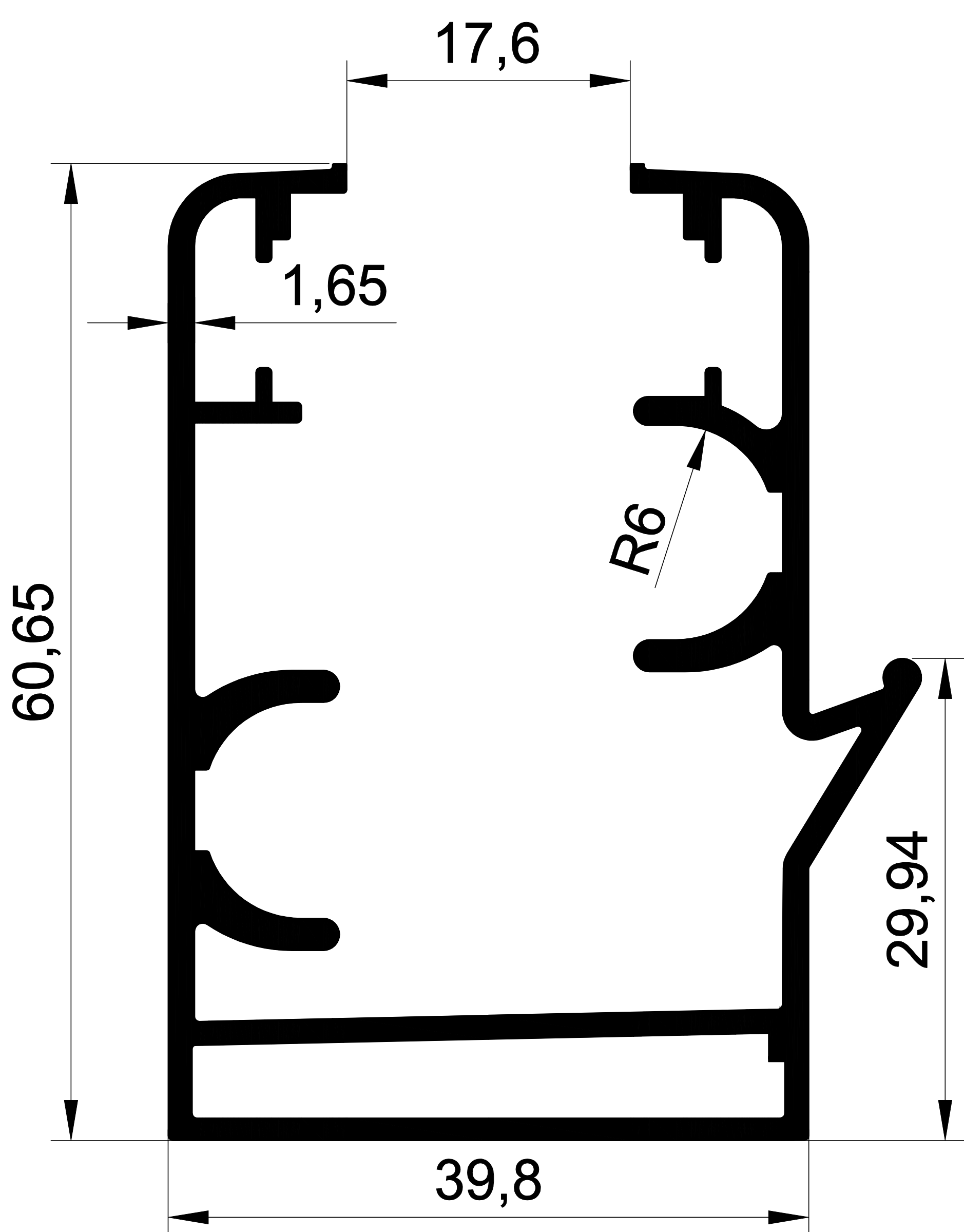
1457 1,262 Kg/m. FIRTINA ORTADAN DAMLALIKLI KASA-1.6 mm
