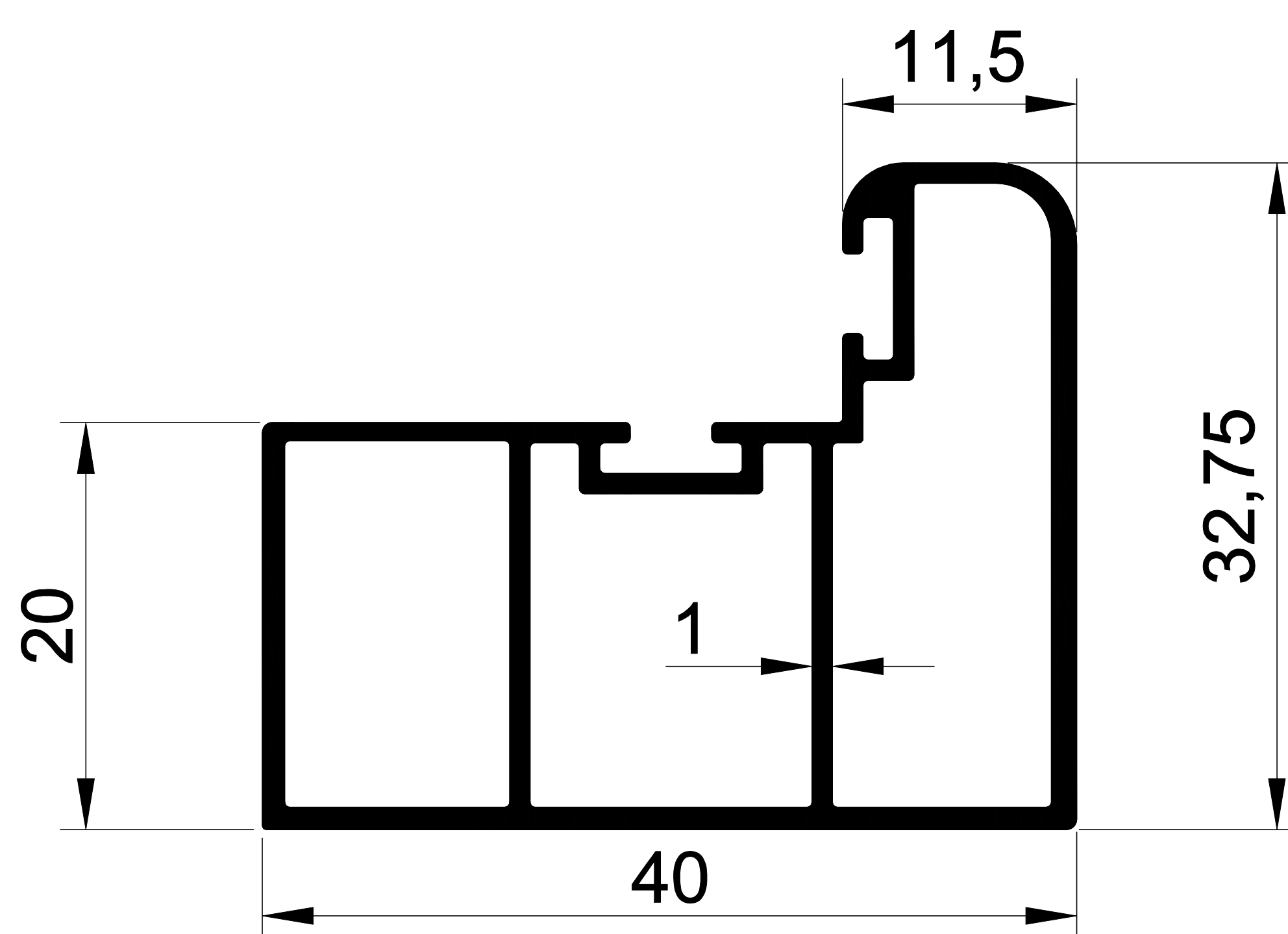
1184 0,533 Kg/m. BKS DİKME
