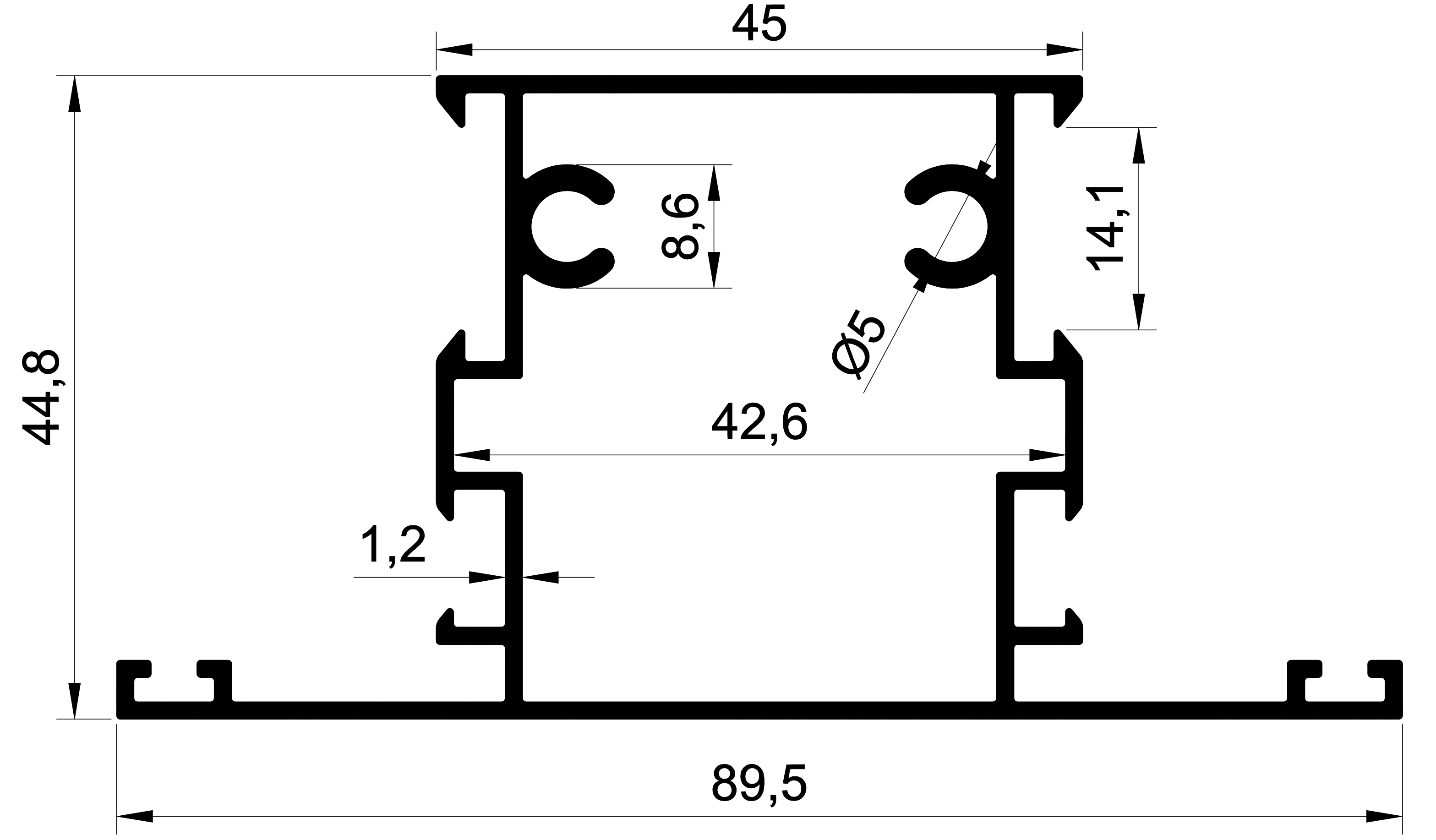
1372 1,054 Kg/m. OVAL ORTA
