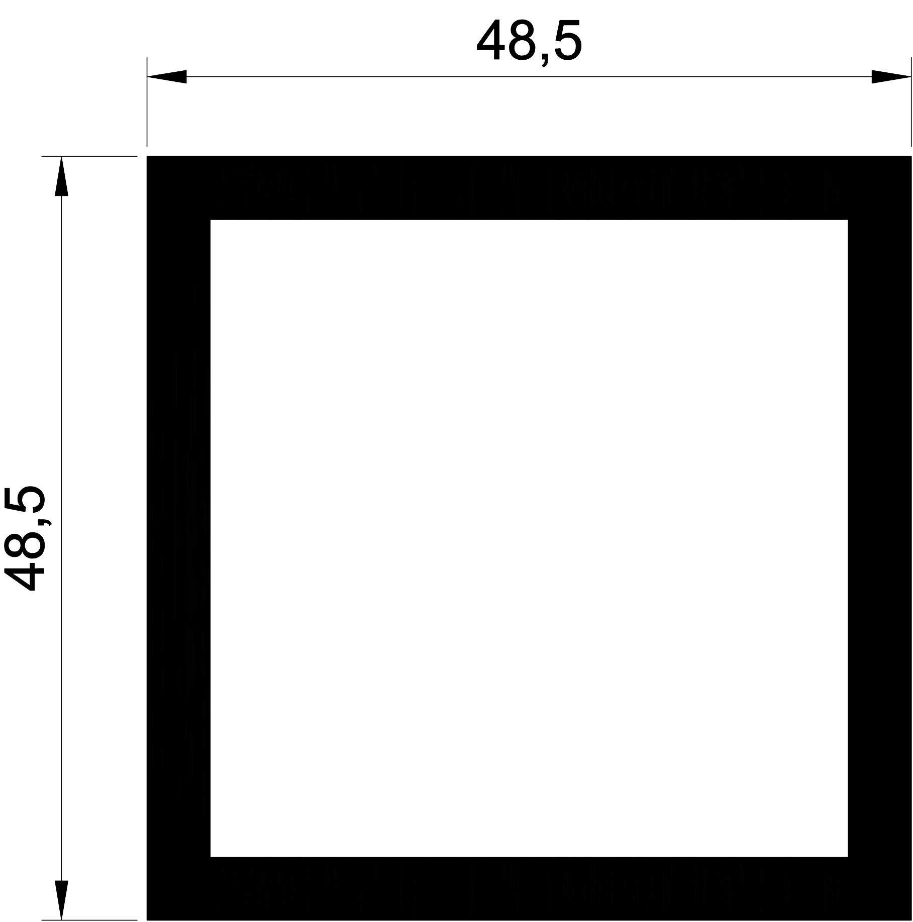
1049 1,929 Kg/m.
