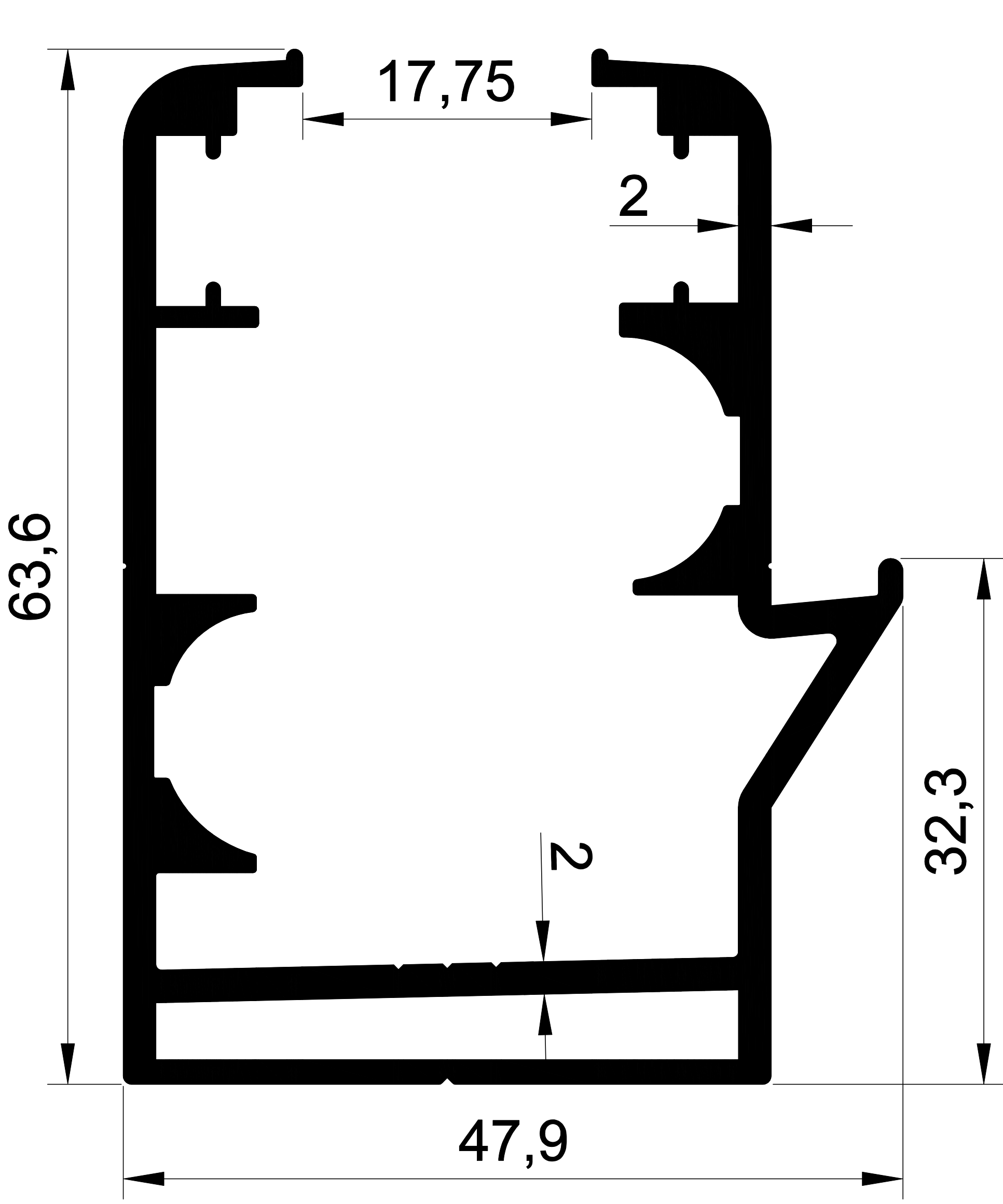
1303 1,453 Kg/m. GOLD ORTADAN DAMLALIKLI KASA
