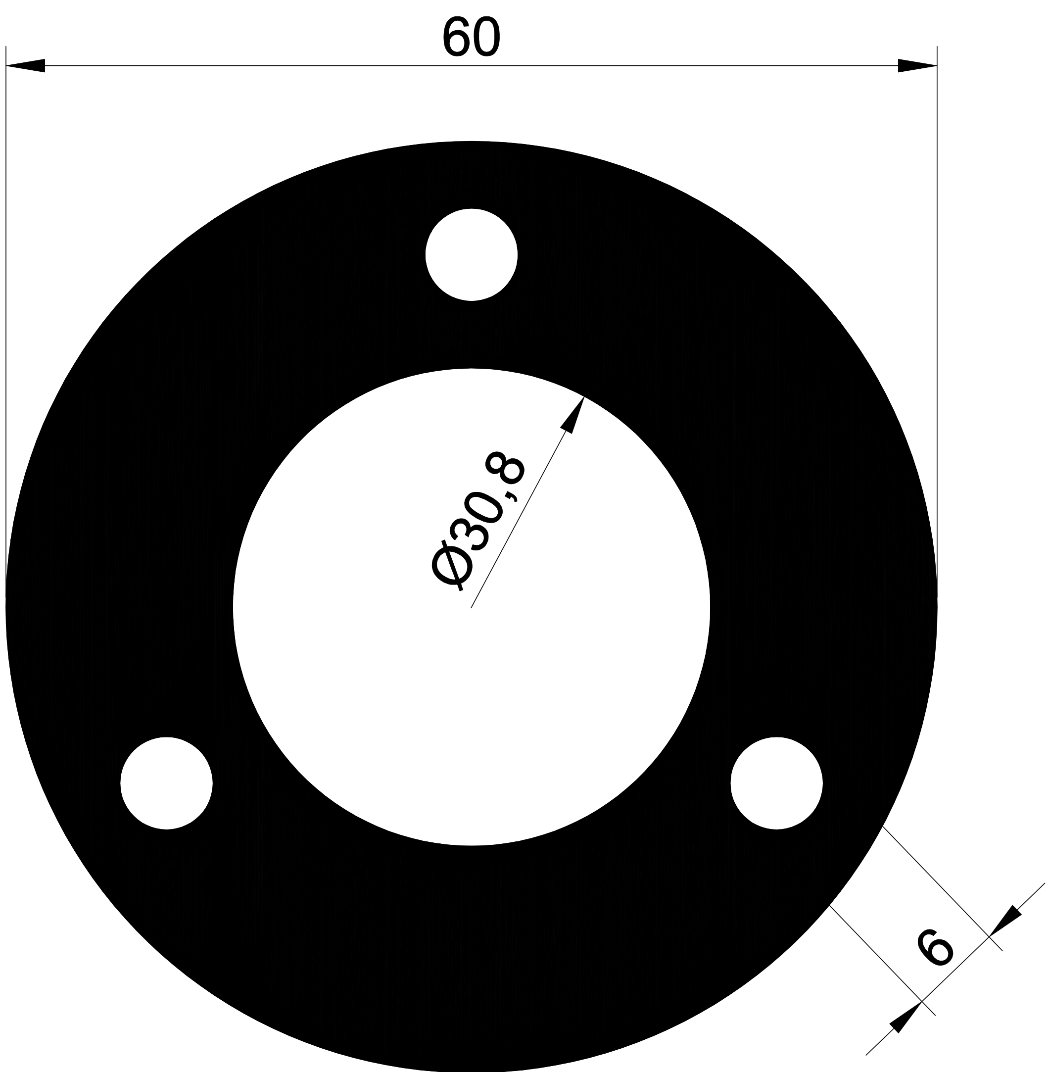
1075 5,414 Kg/m.
