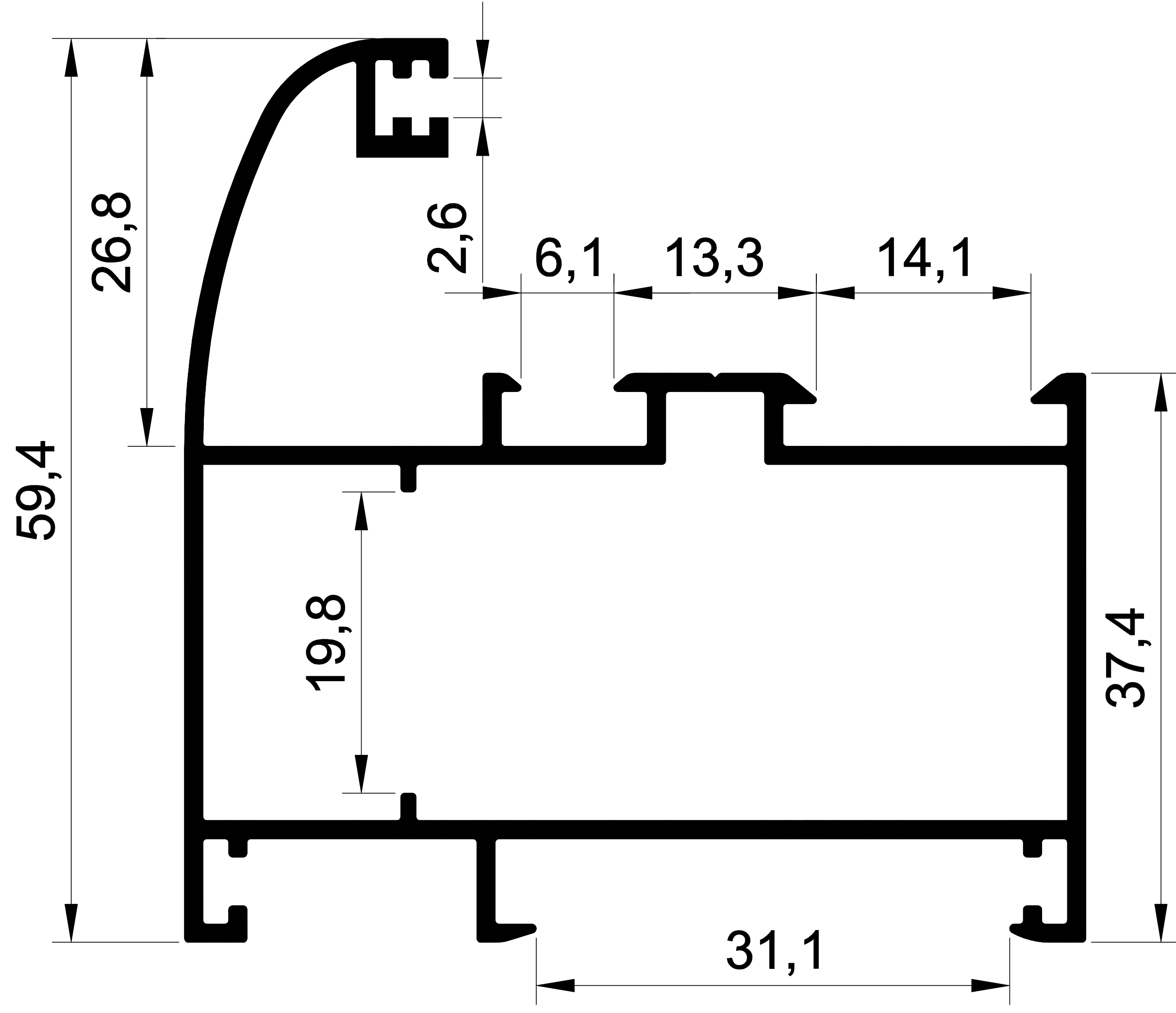
1369 0,917 Kg/m. OVAL KASA
