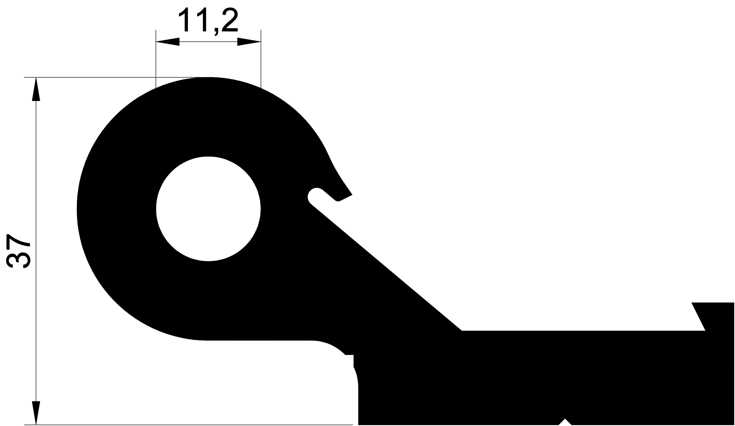
1235 2,824 Kg/m.
