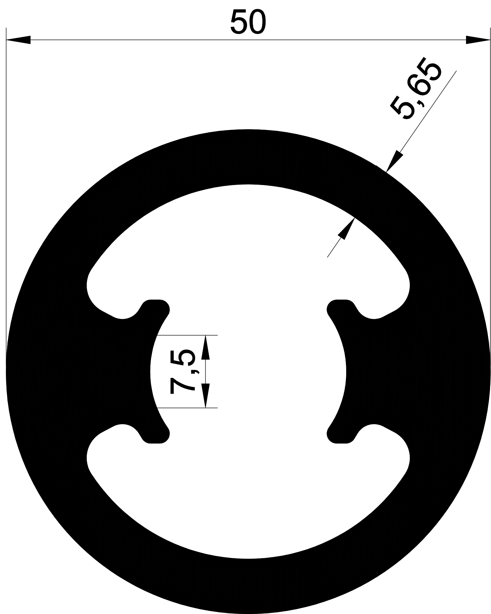
1029-B 2,593 Kg/m.
