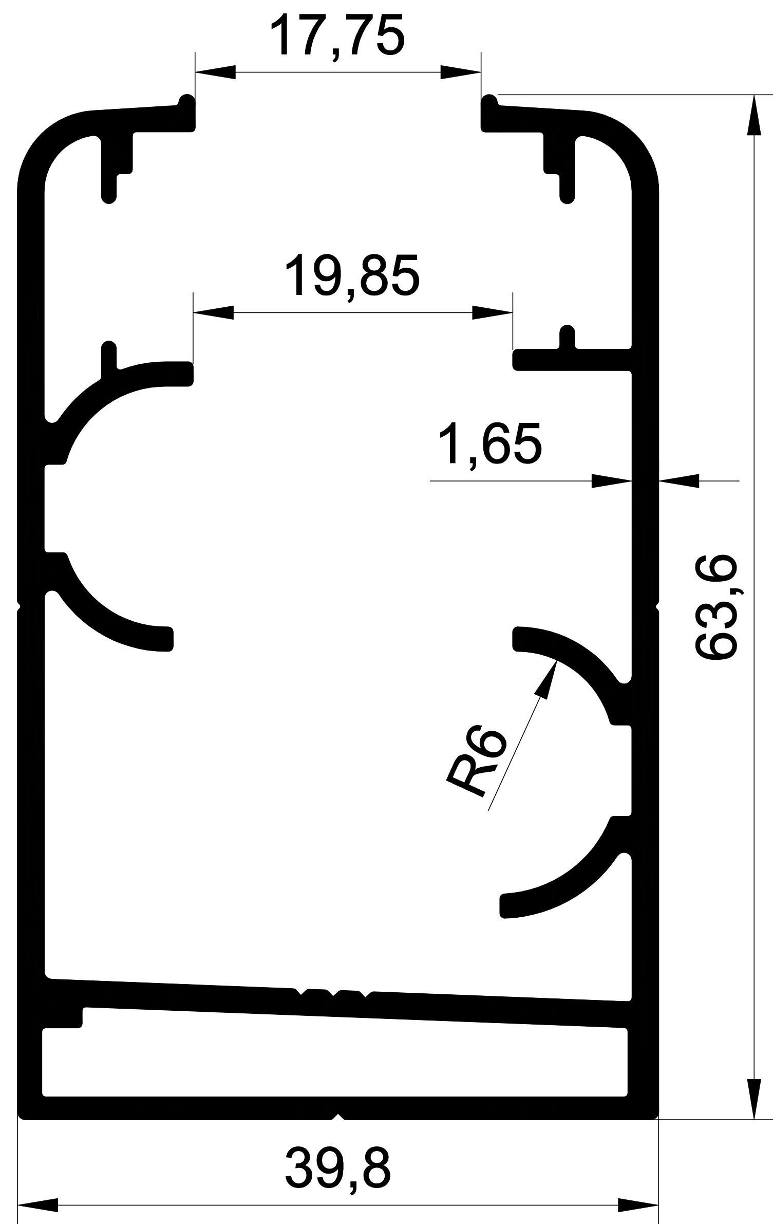
1250-C 1,172 Kg/m. GOLD KASA-1,65 mm
