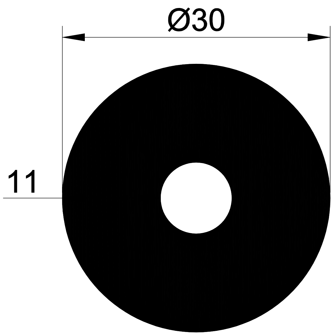
1005 1,778 Kg/m.
