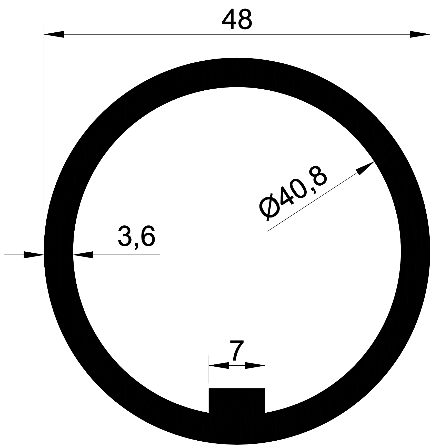
1018 1,423 Kg/m.
