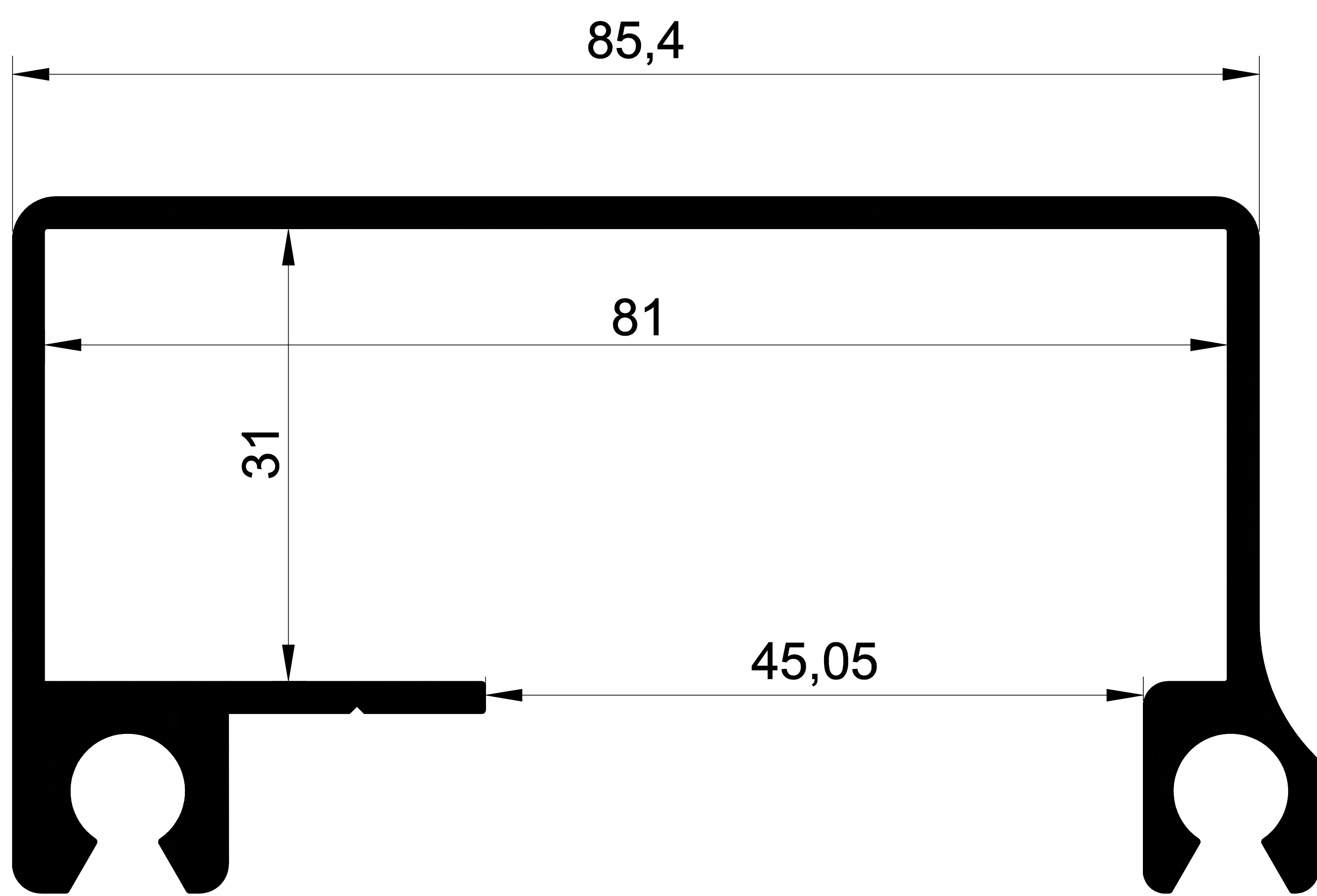
1301 1,612 Kg/m.
