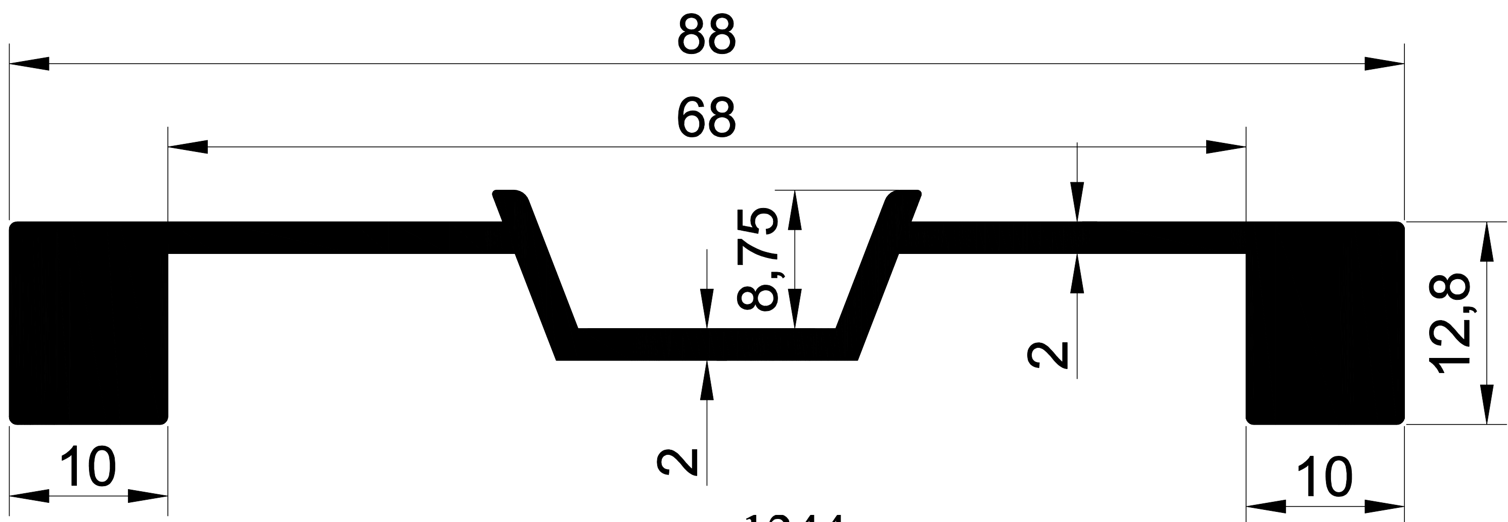
1244 1,135 Kg/m.
