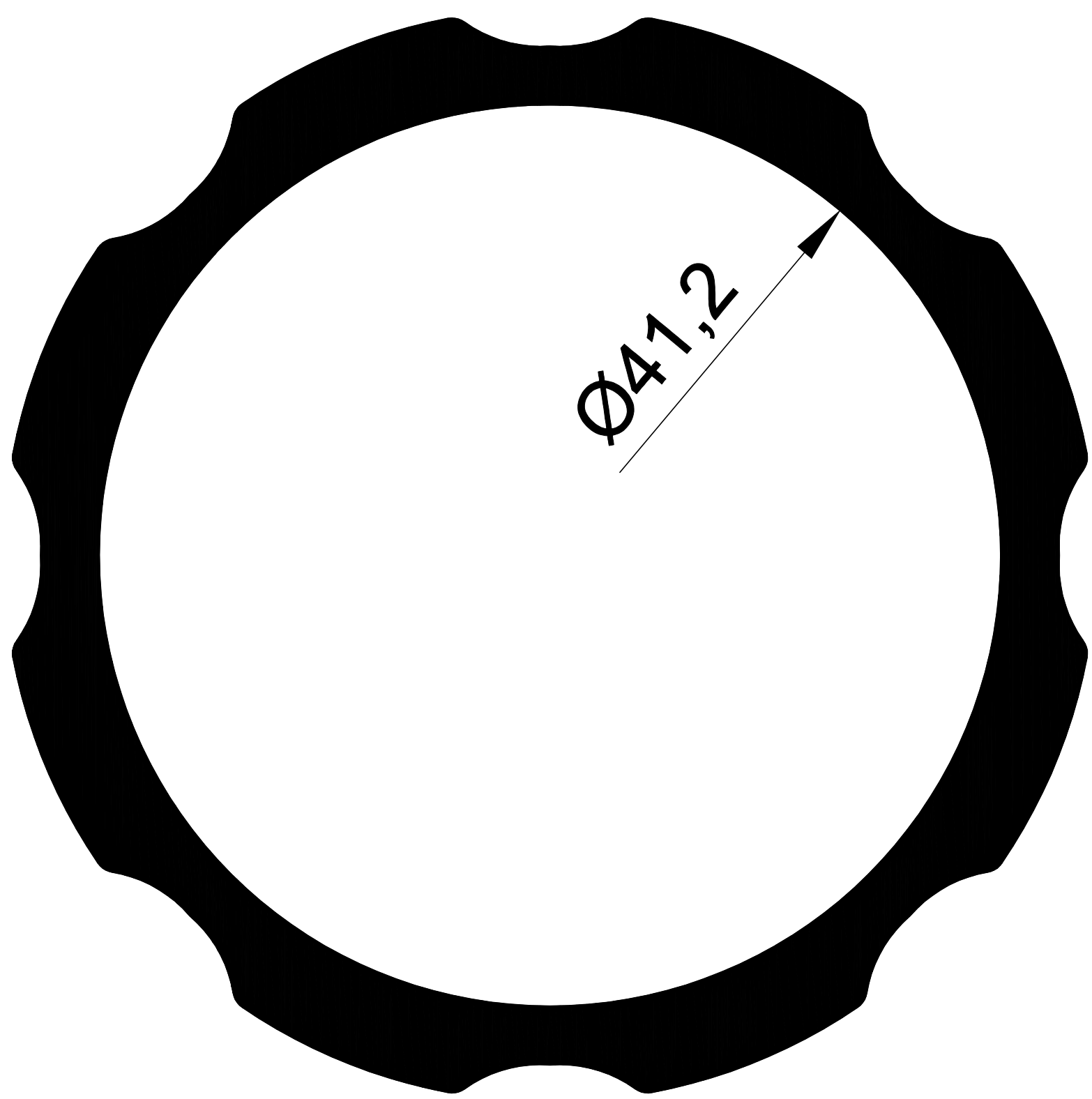
1213 1,485 Kg/m.
