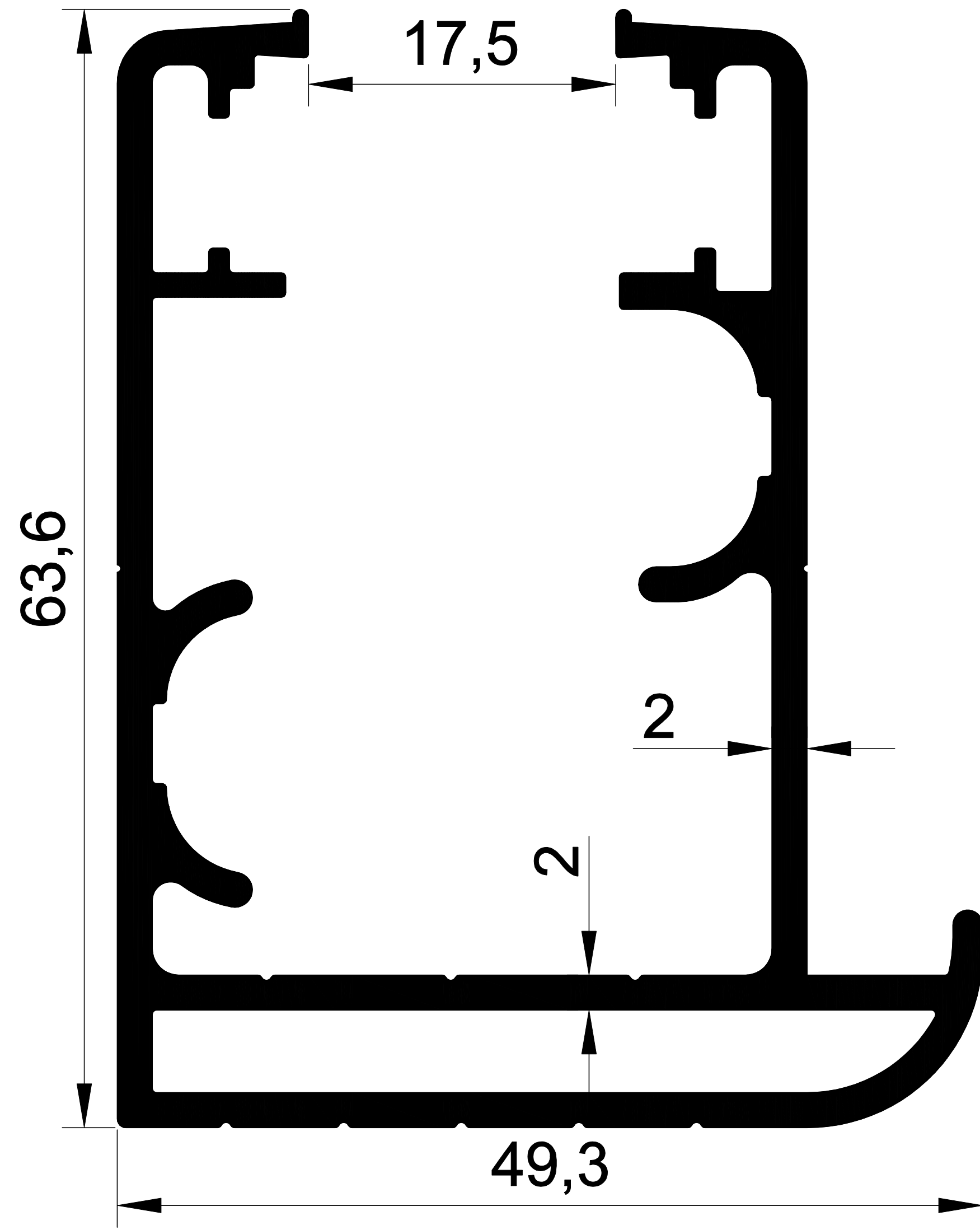
1270 1,523 Kg/m. GOLD ALTTAN DAMLALIKLI KASA
