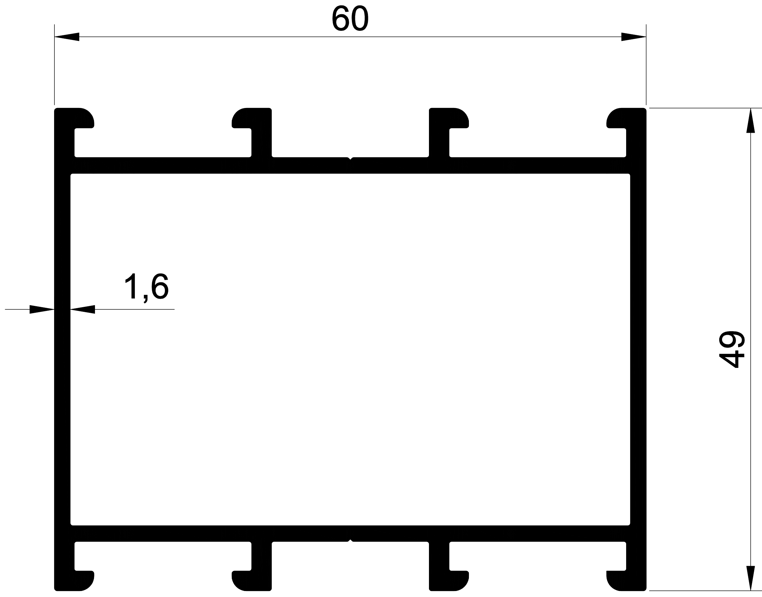
1407 1,123 Kg/m. 1.6 MM C-60 KASA
