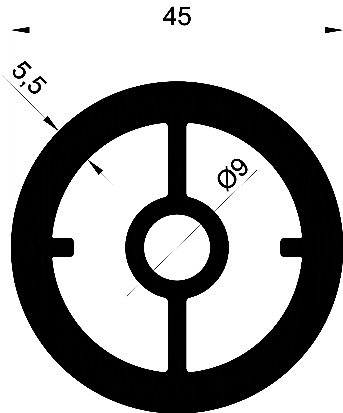
1022 2,271 Kg/m.
