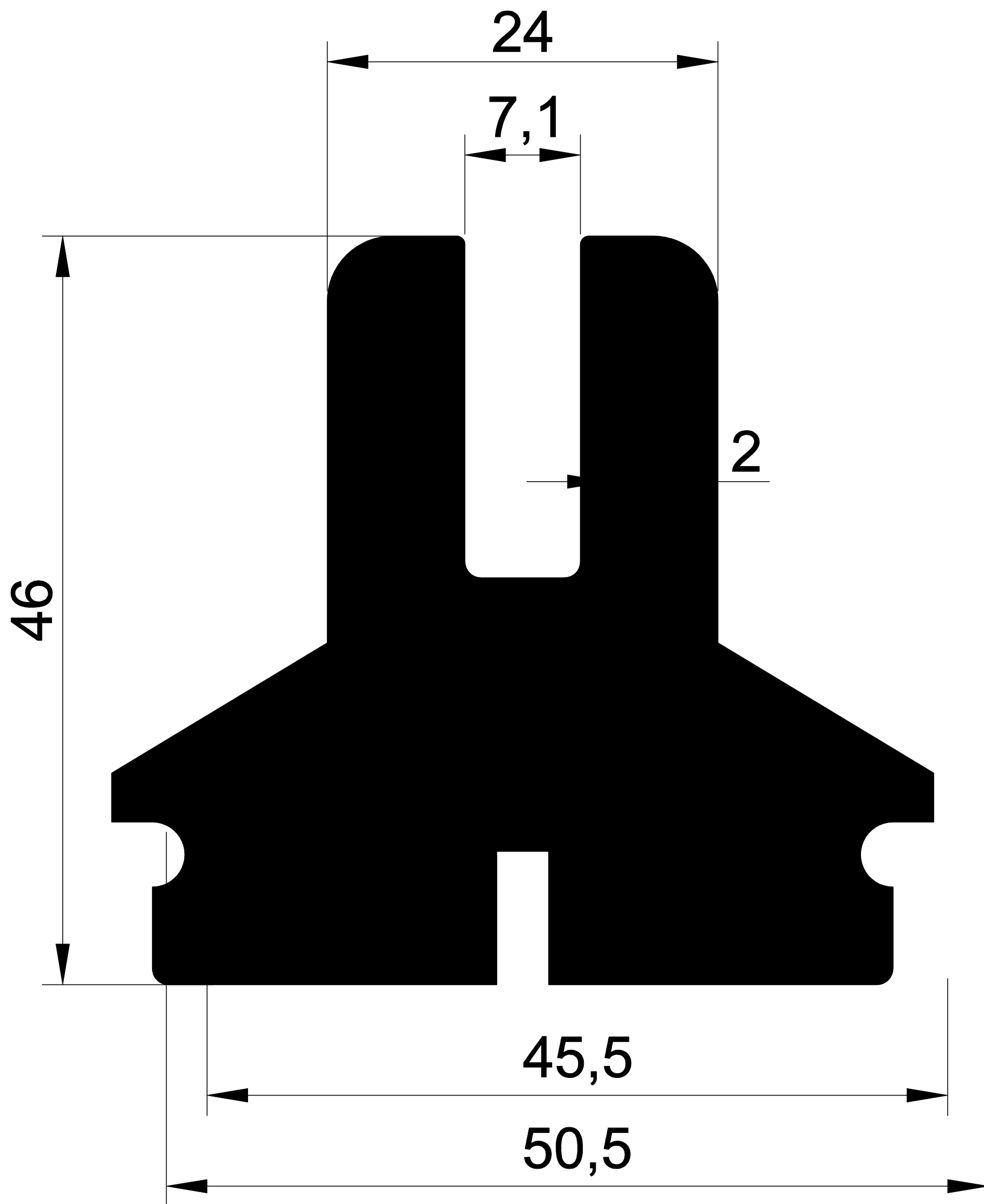
1122 3,550 Kg/m.
