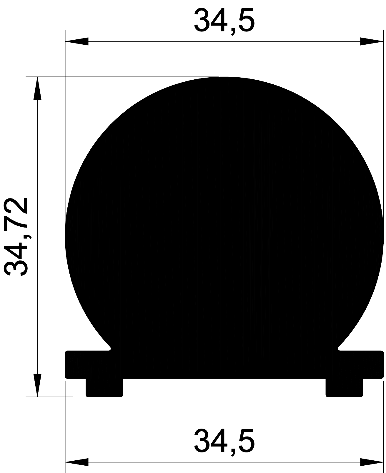
1297 2,645 Kg/m.
