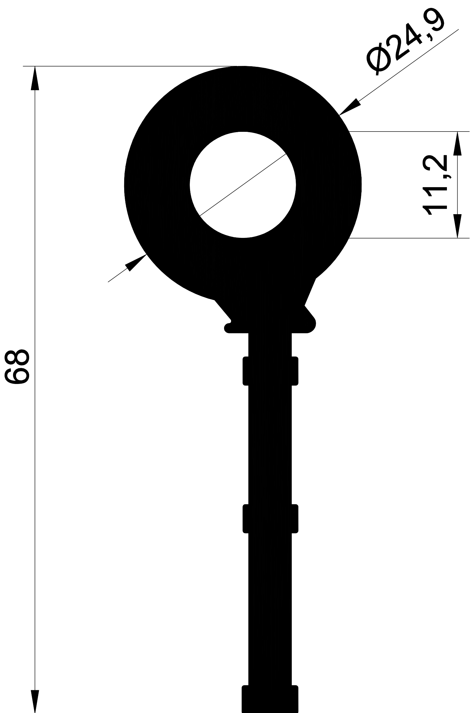
1010 1,661 Kg/m.
