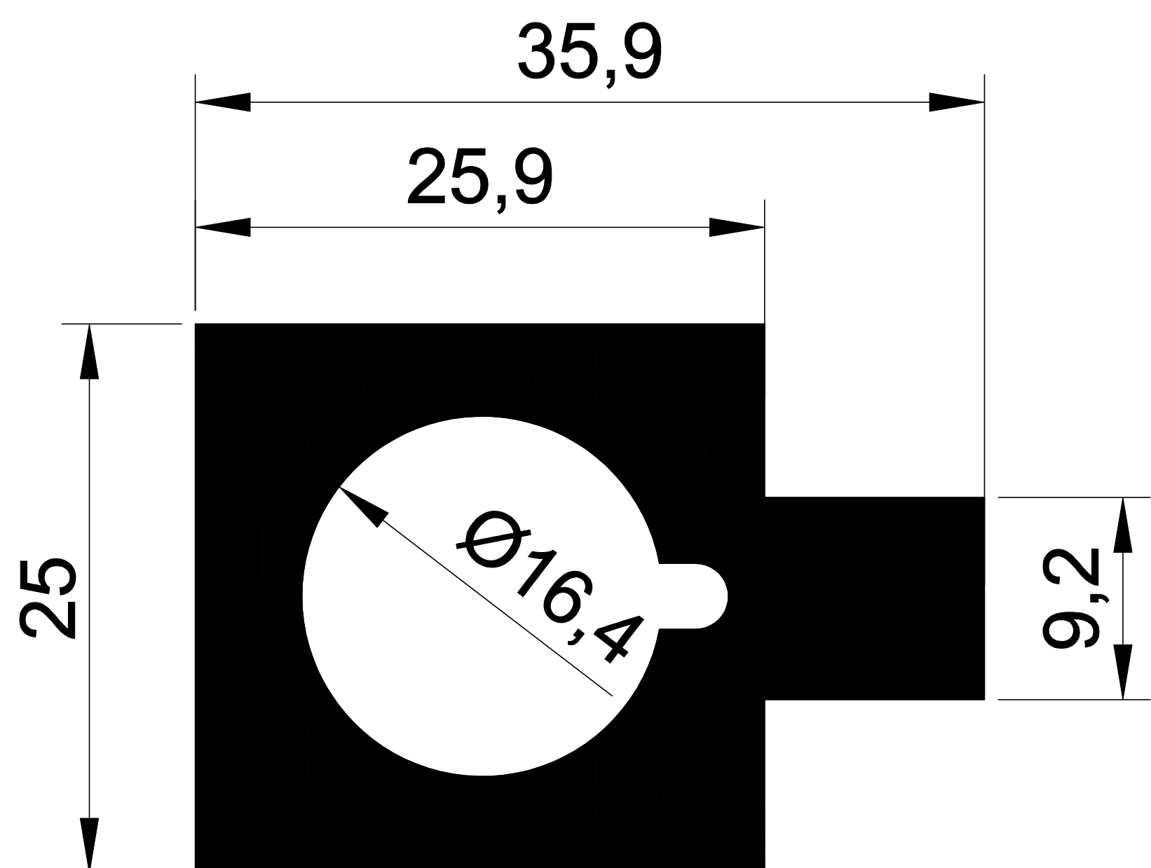
1220 1,412 Kg/m.
