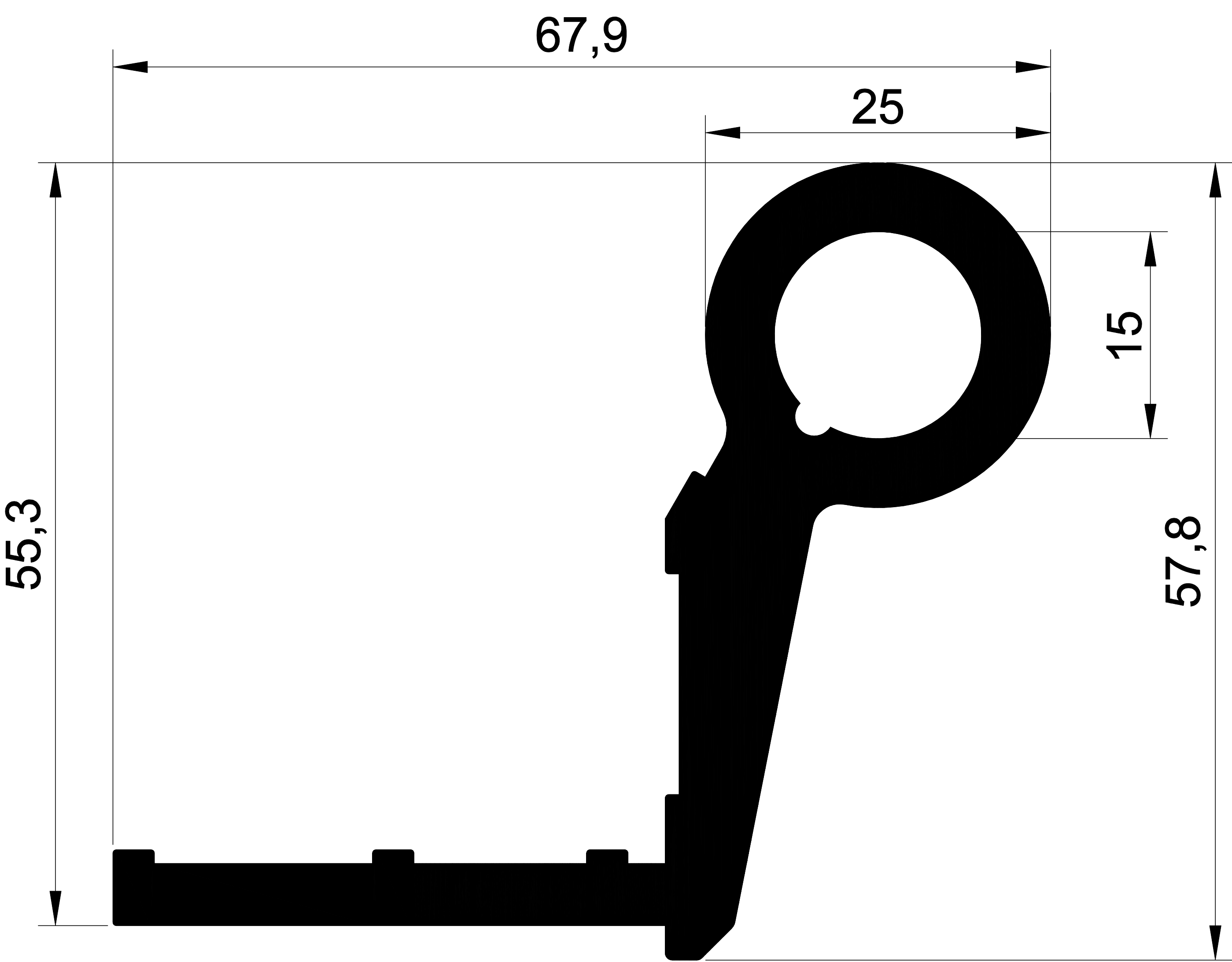
1011 2,073 Kg/m.
