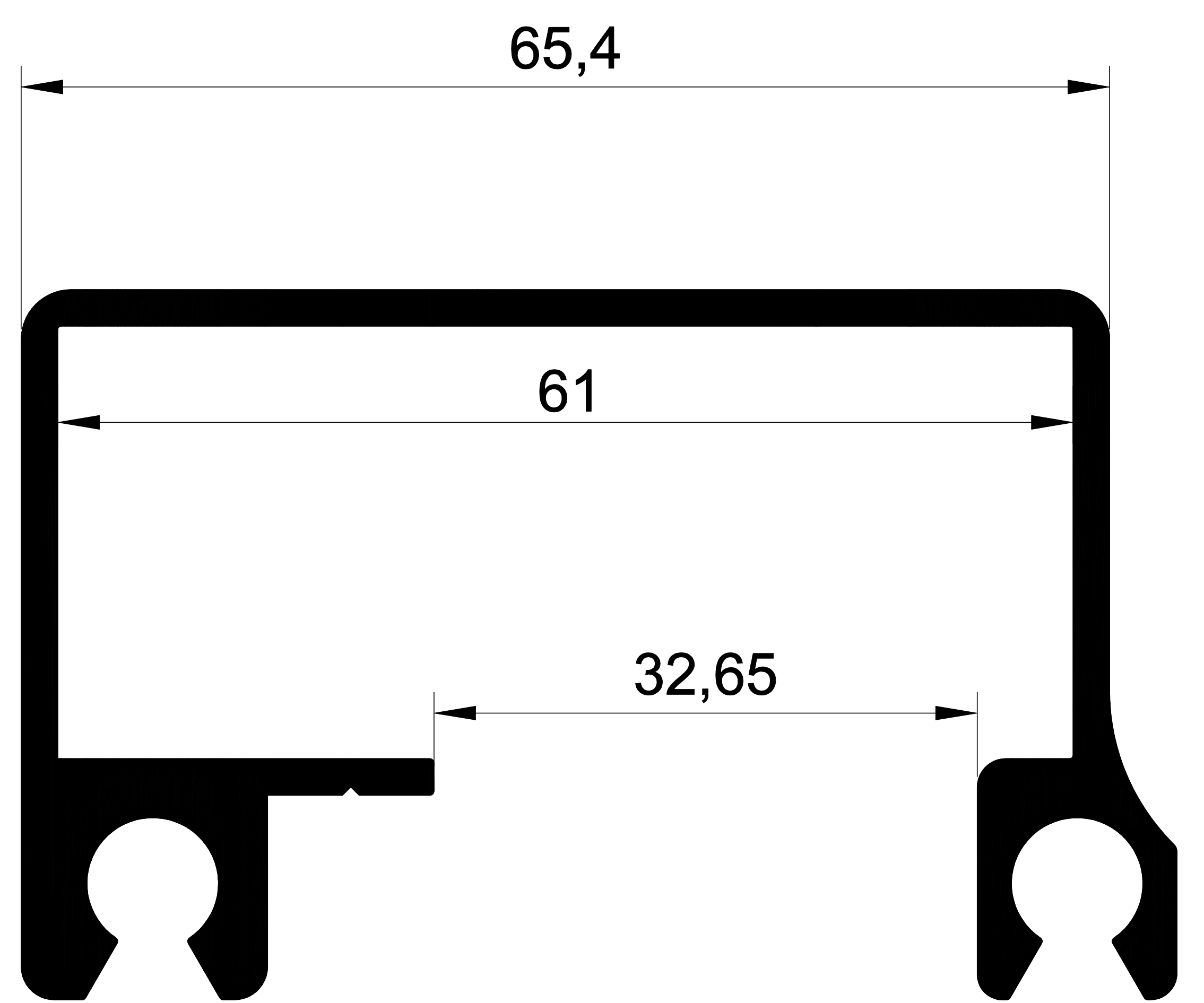
1302 1,387 Kg/m.
