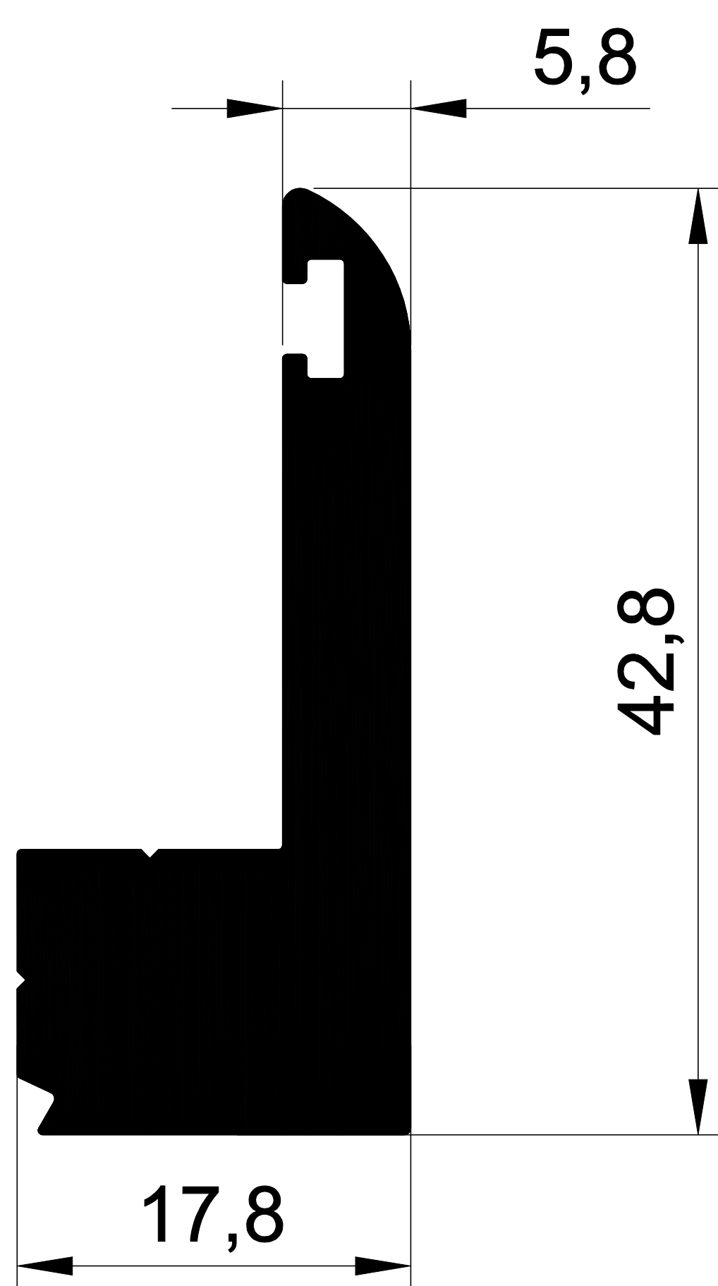
1248 1,022 Kg/m.
