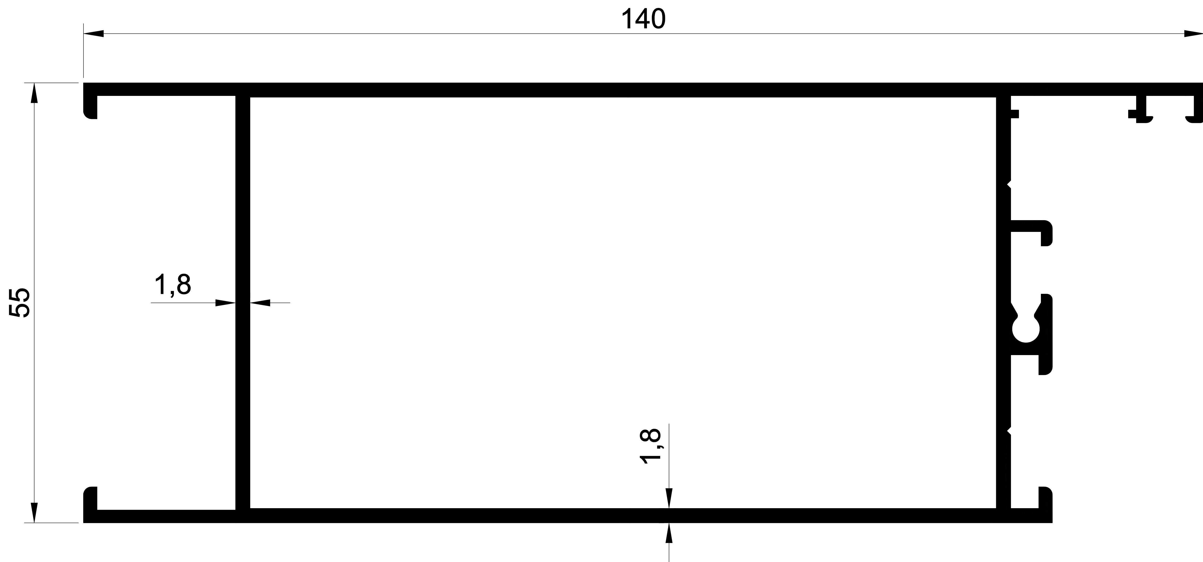
1205 1,902 Kg/m. SİSTEM ETEK
