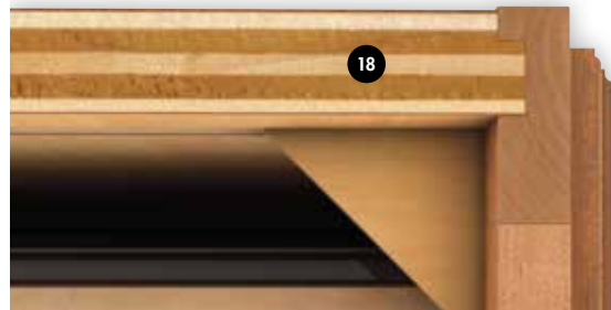
3/4" Furniture Ends Construction
