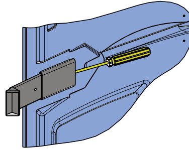
2 INSERT SLIDE LATCH INTO DOOR PULL USE SCREWDRIVER TO ASSIST IN SLIDING THE LATCH COMPLETELY INTO THE DOOR PULL
