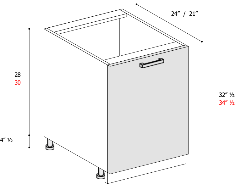
Overall dimensions of base units H.34" 1/2 with handle
