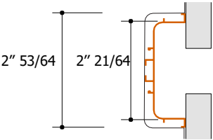
Single vertical groove for tall units
