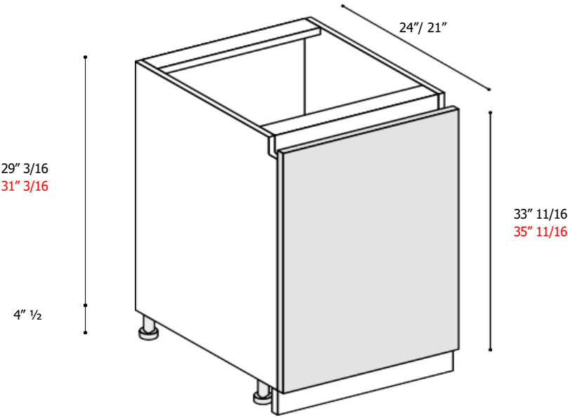
Overall dimensions of base units H.35" 11/16 with groove
