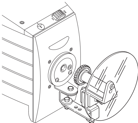
Anti-snarling unit
