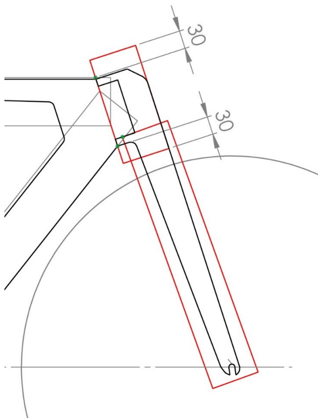
Figure 32: Illustration of the position of the boxes for offset fork
