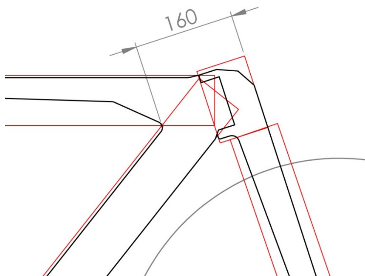
Figure 18: Illustration of the limit case
