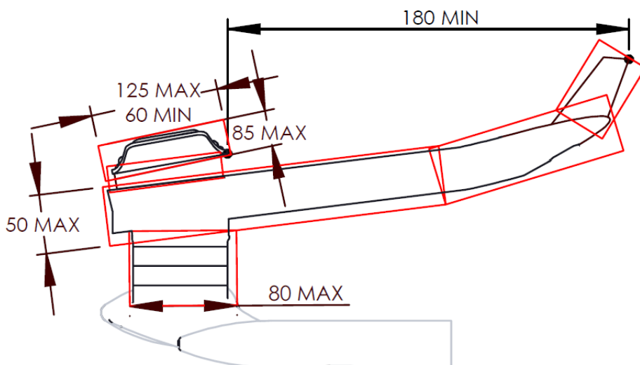
Figure 45 Illustration (C) of templates formed by red boxes for each element
