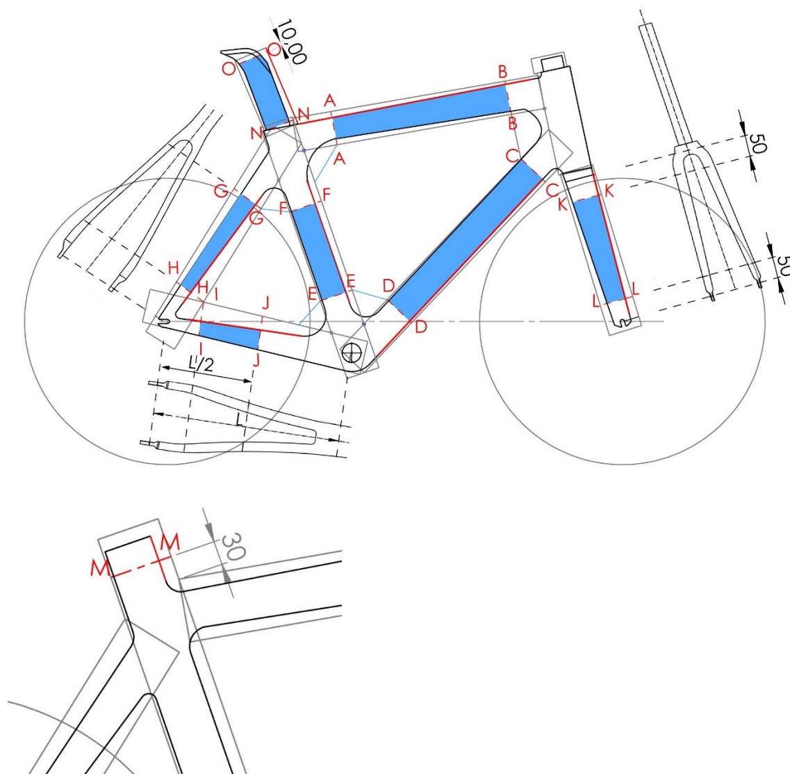
Figure 25: Illustrations of the areas of the frameset subject to the rule of minimum and maximum dimension
