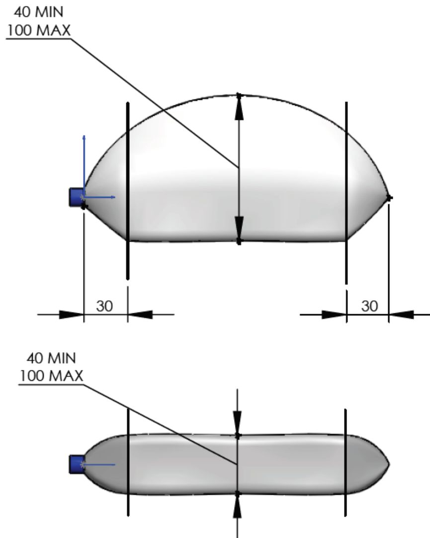
Figure 66: Illustration of the areas of a bottle where the dimensions are subject to regulations
