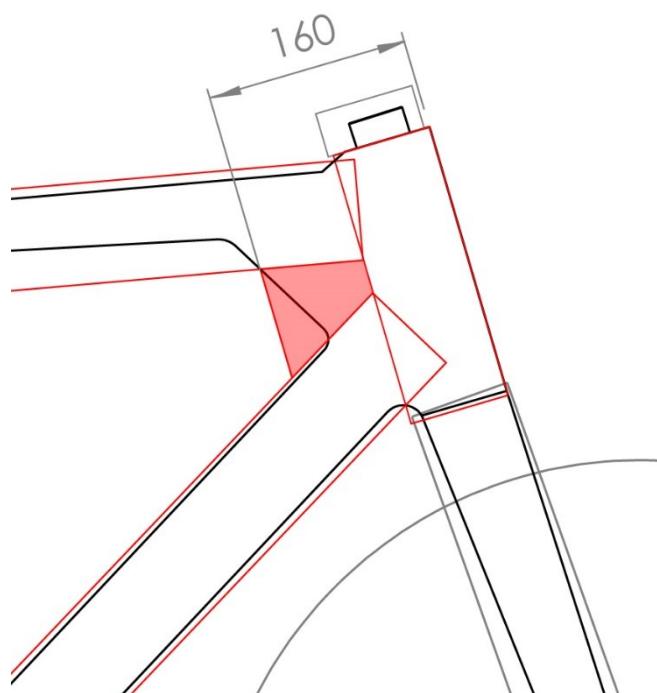
Figure 19: Illustration of the compensatory joint zone
