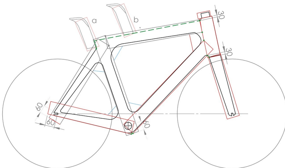
Figure 23: Illustration of the positioning of the seat post box
