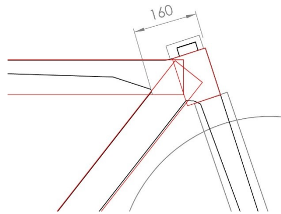
Figure 17: Illustration of the maximum distance of 160 mm for a small frame size (B)
