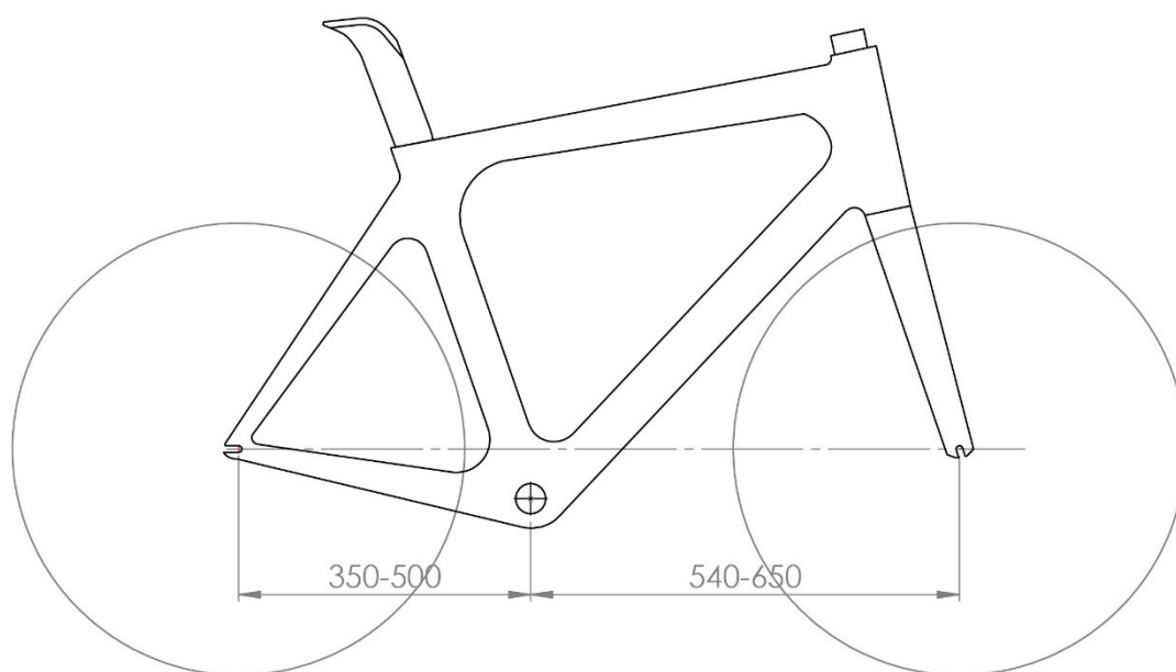
Figure 8: Illustration of the minimum and maximum distances between the bottom bracket and front and rear wheel axles
