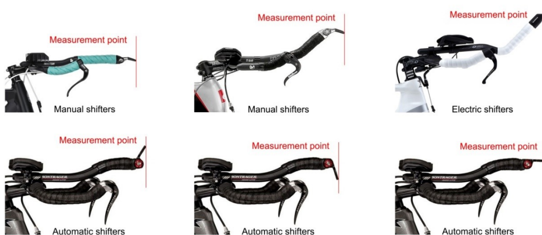
Figure 54 Points of measurement for the horizontal distance from the bottom bracket axle
