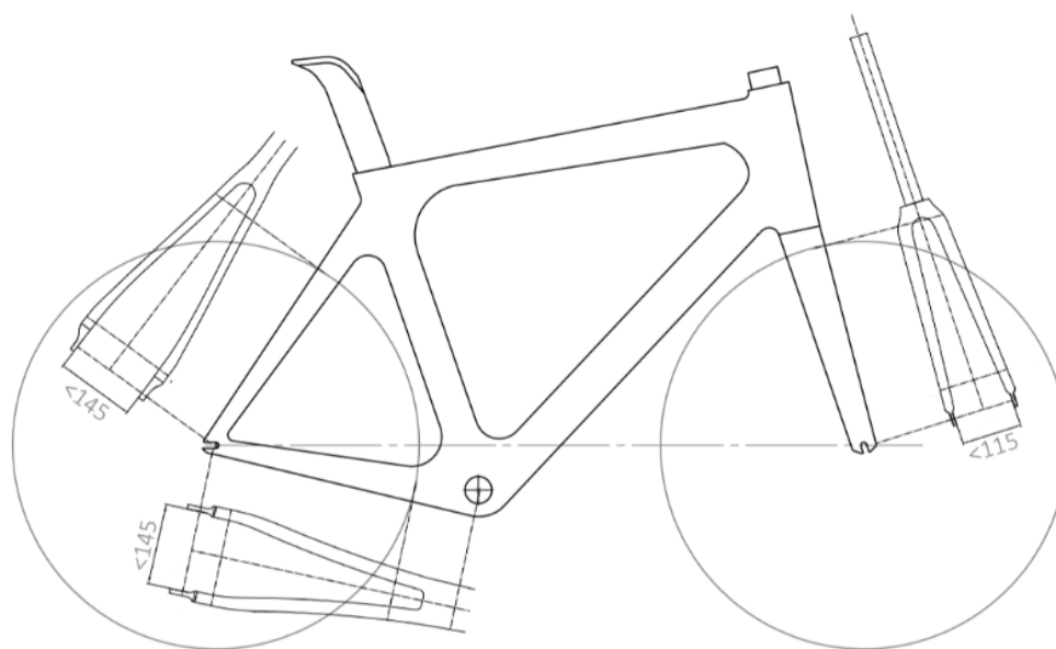
Figure 9: Road and Cyclo-cross - Illustration of the maximum distances between the internal extremities of the two legs of the front forks and the two sides of the rear triangle
