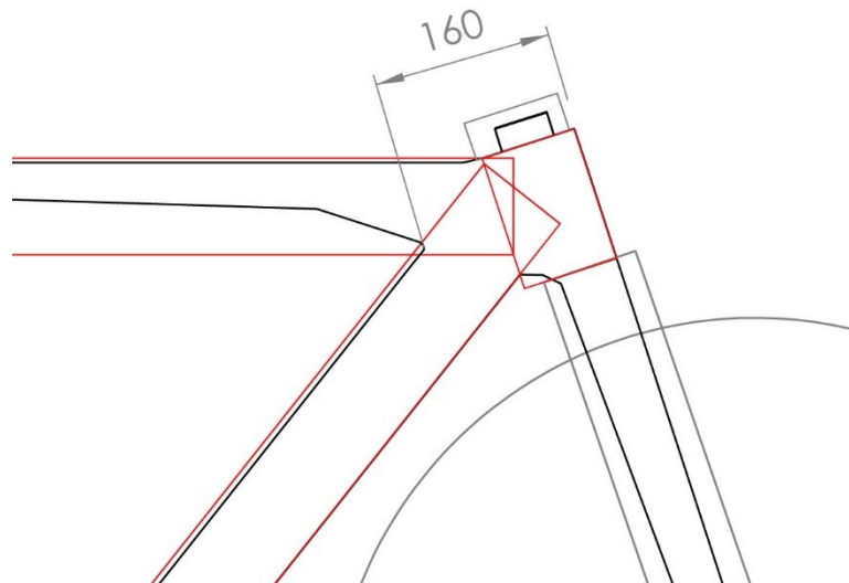
Figure 15: Illustration of the 160 mm rule
