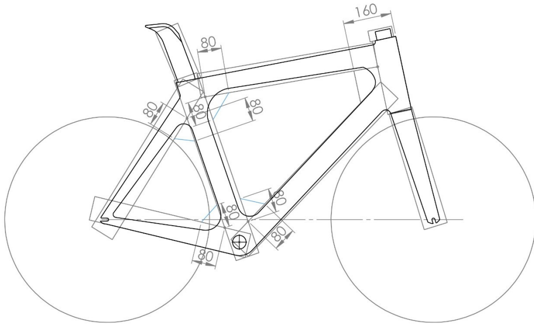
Figure 14: General illustration of compensation triangles and boxes
