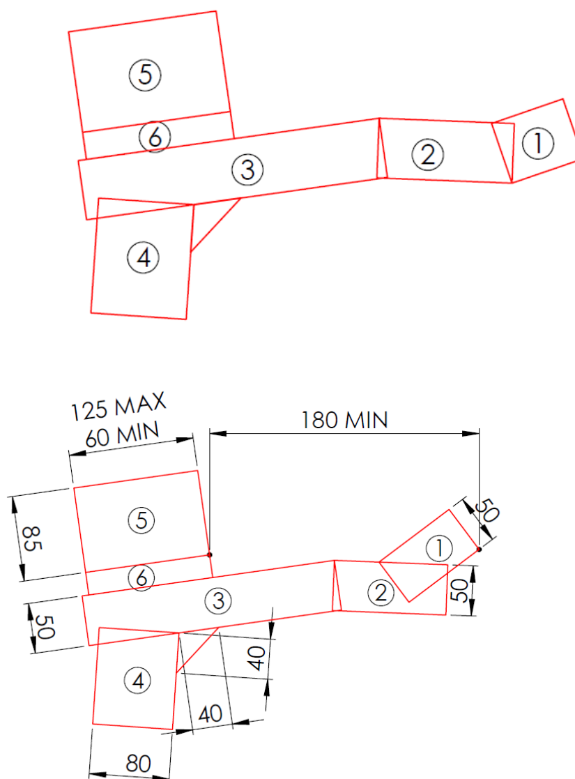
Figure 44 Illustrations (A), (B) of templates formed by red boxes for each element
