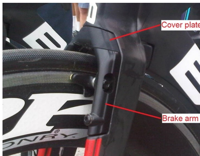
Figure 59: Brake integrated with the fork and fitted with a cover
