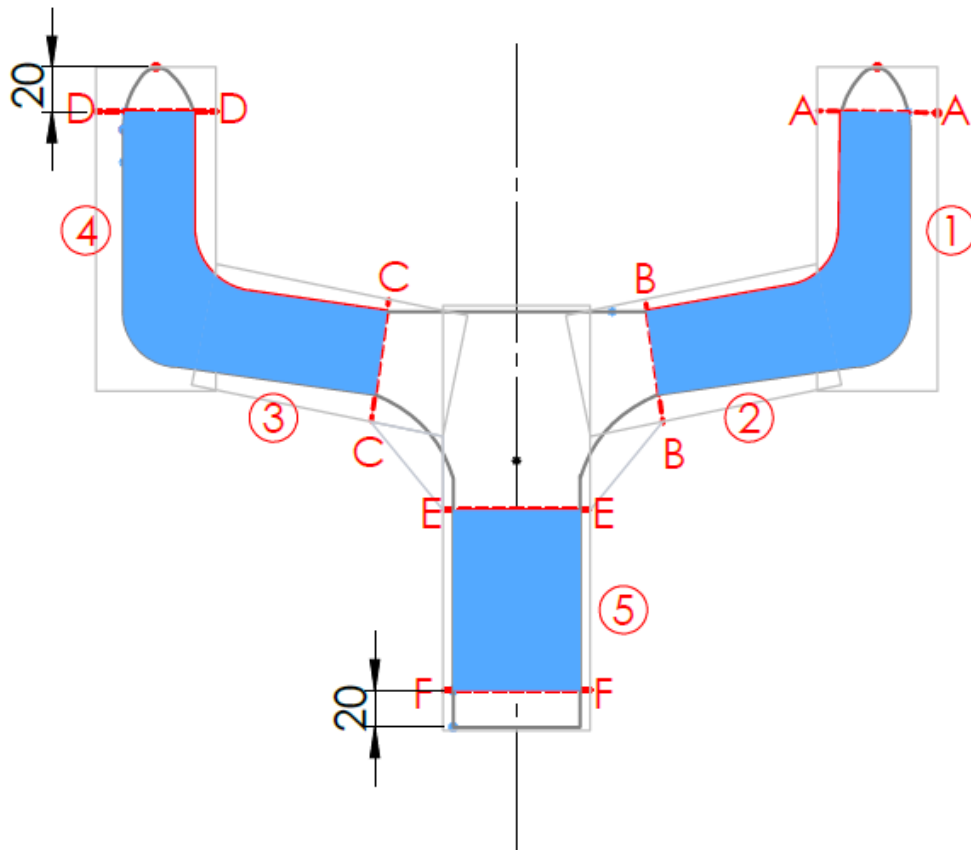
Figure 43 Illustration of minimum and maximum dimensions requirements
