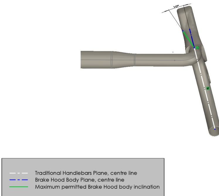
Figure 36 Illustration of the maximum permitted Brake Hood body inclination in combination with a flared traditional handlebars
