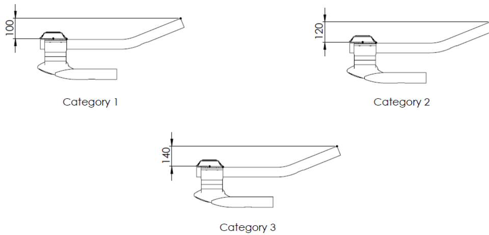
Figure 51 Examples of the vertical limits per each height category (as per provisions of article 1.3.023)
