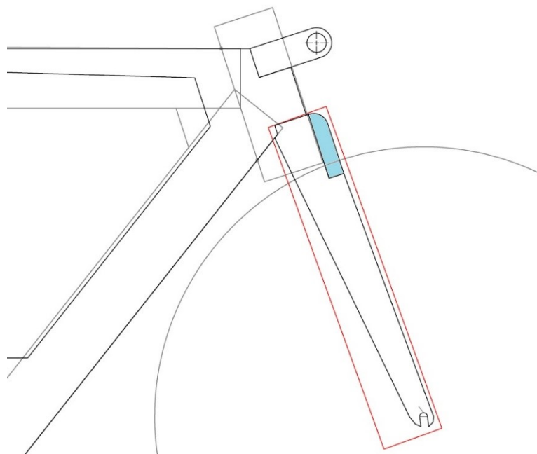
Figure 60: Illustration of a cover that fits over the brake only
