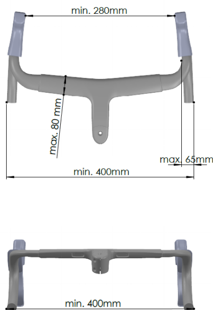
Figure 37 Road & Cyclo-cross, Illustration of the handlebar that must comply with the minimum overall width of 400 mm
