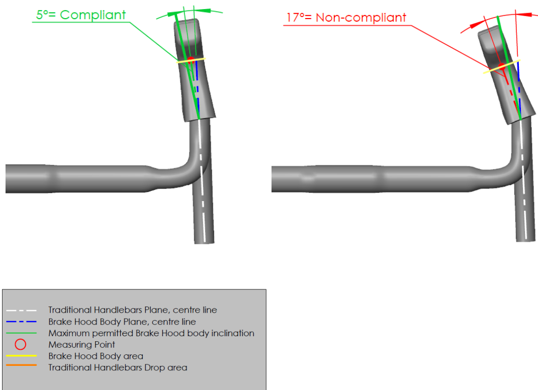
Figure 35: Illustration of the maximum permitted Brake Hood body inclination
