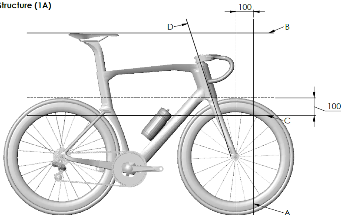
Figure 34: Illustration of the box, marked out by lines A, B, C and D, within which the handlebars must be fully contained.
