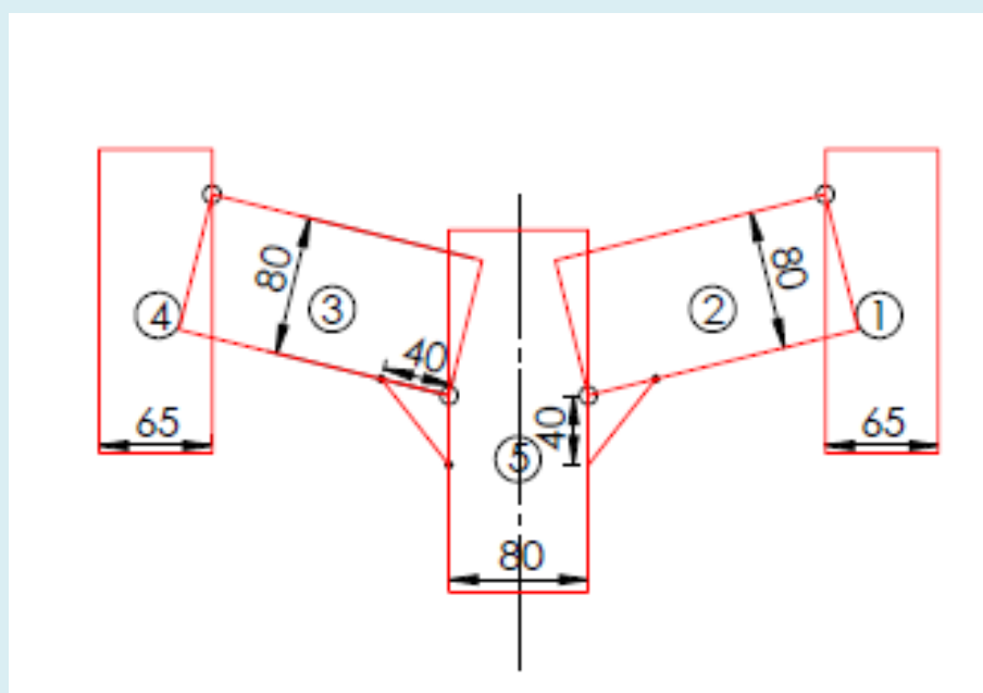
Structure (1.0) Road, Cyclo-cross
