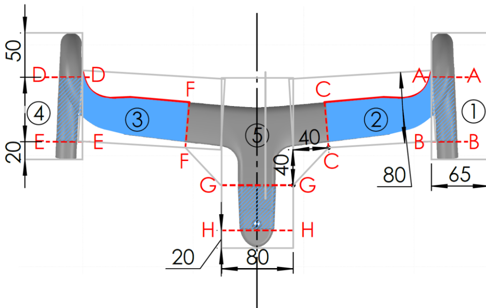
Figure 39 Road, Cyclo-cross, Illustration of minimum and maximum dimensions requirements
