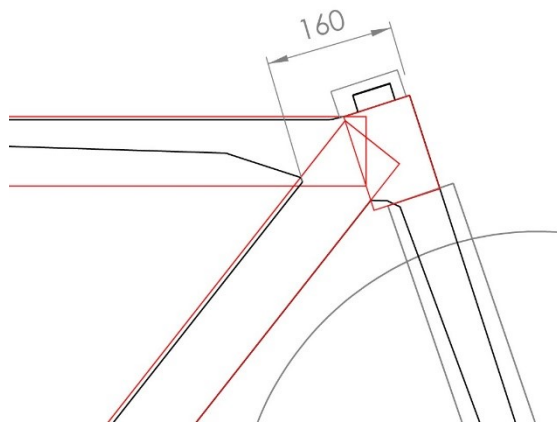
Figure 16: Illustration of the maximum distance of 160 mm for a small frame size (A)
