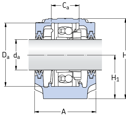
Four-lip seals L design
