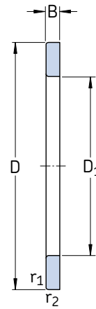
Housing washer
