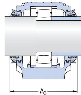
Taconite seals ND design
