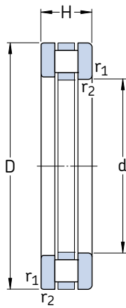
Complete bearing
