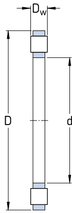
Cylindrical roller and cage thrust assembly
