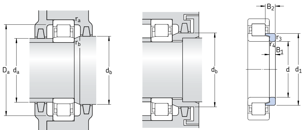
Angle ring
