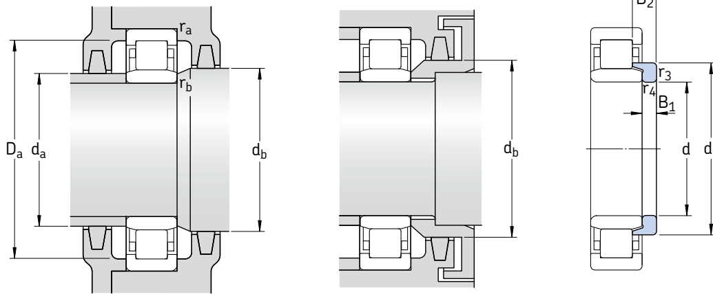
Angle ring
