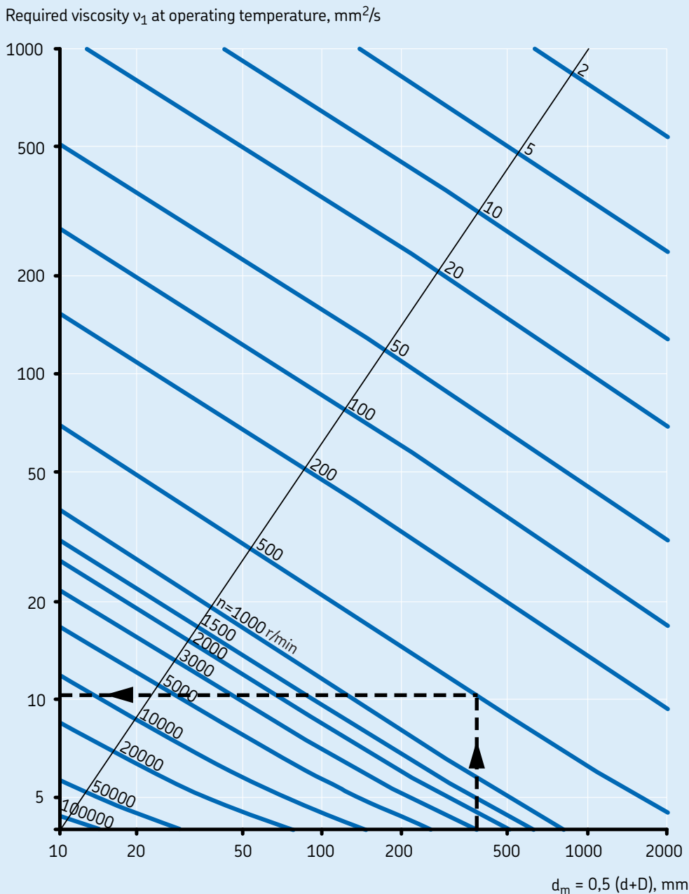
Estimation of the minimum kinematic viscosity v_1 at operating temperature
