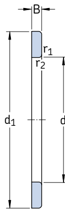
Shaft washer
