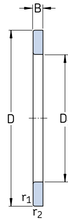
Housing washer
