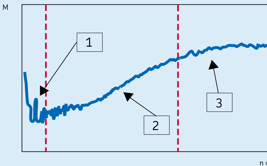
Bearing frictional moment as a function of the speed and viscosity
