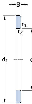
Shaft washer
