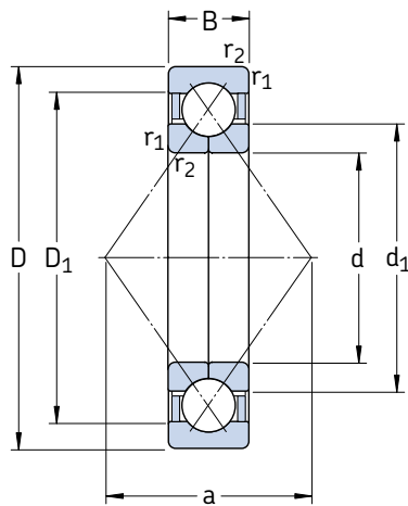
Basic design
