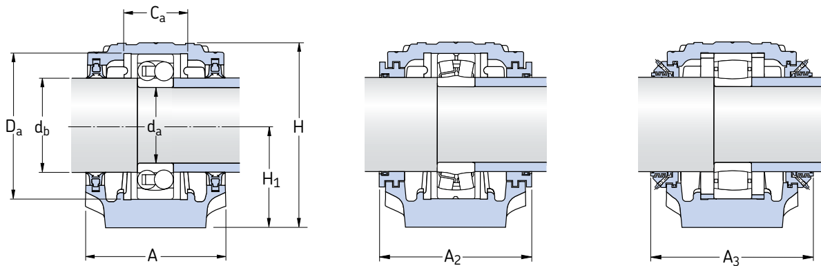
Double-lip seals G design
