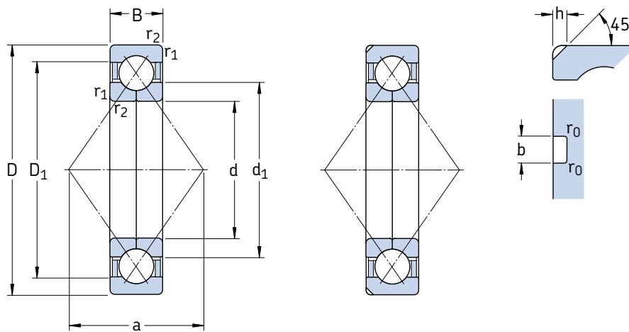
Basic design
