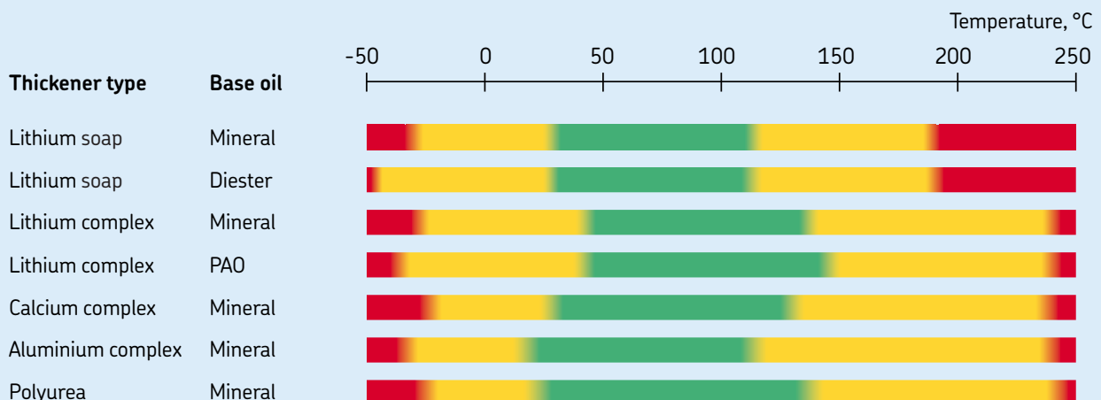
The SKF traffic light concept – standard greases
