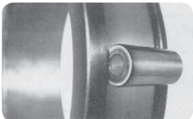
Seizing damage usually appears on the rollers. (fig. 9)
