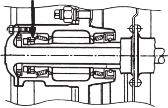
Double adjusting nut
