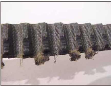
Figure 10 - Extreme belt edge wear
