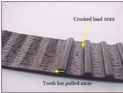
Figure 15 - Extreme land crushing and wear from excessive sprocket runout
