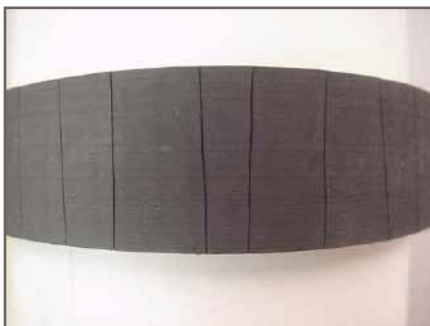
Figure 17 - Cracking from high temperature operation, rubber
