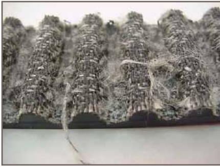
Figure 12 - Extreme tooth wear from worn sprockets
