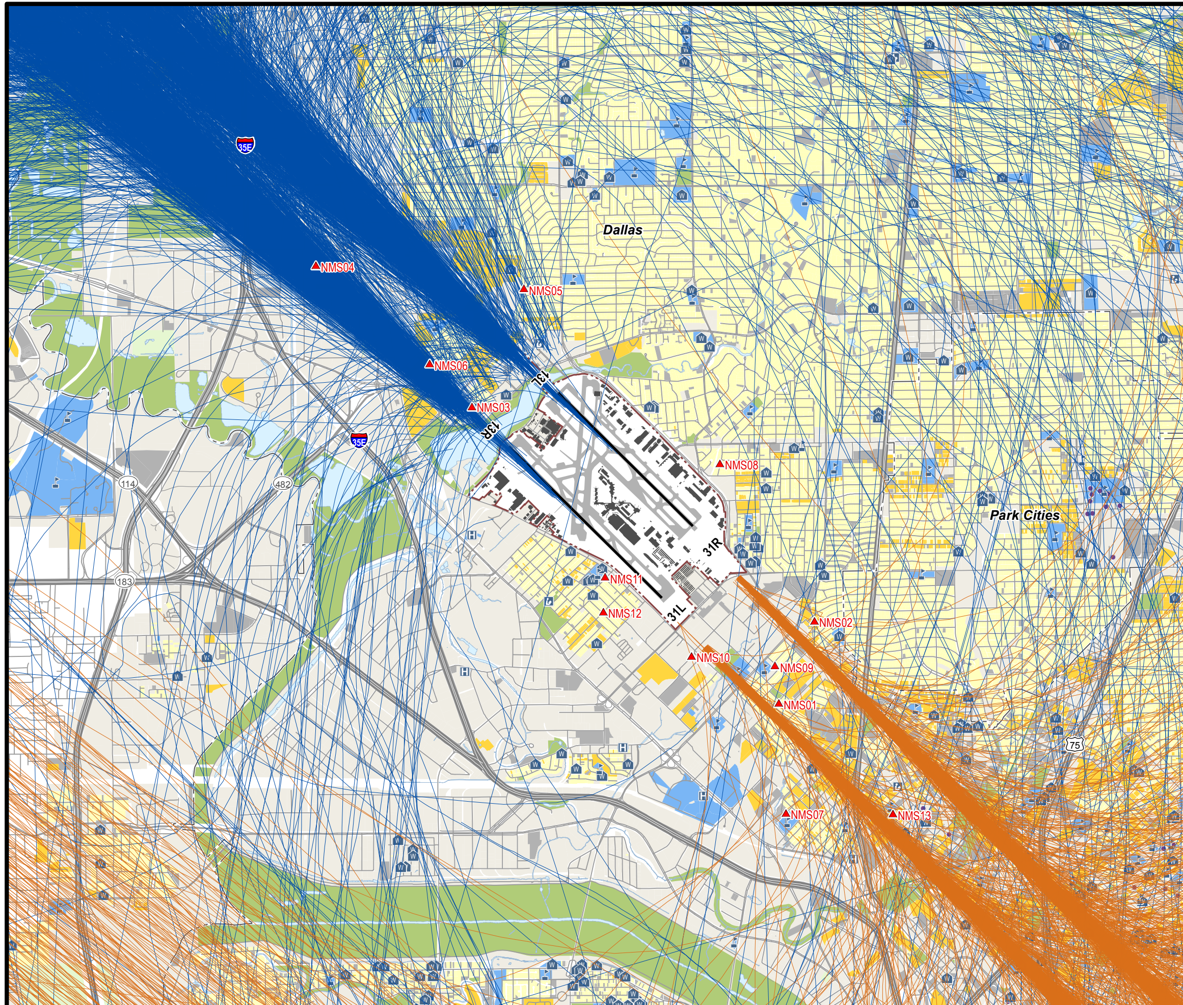
Figure 13 Sample of Modeled North Flow Flight Tracks
