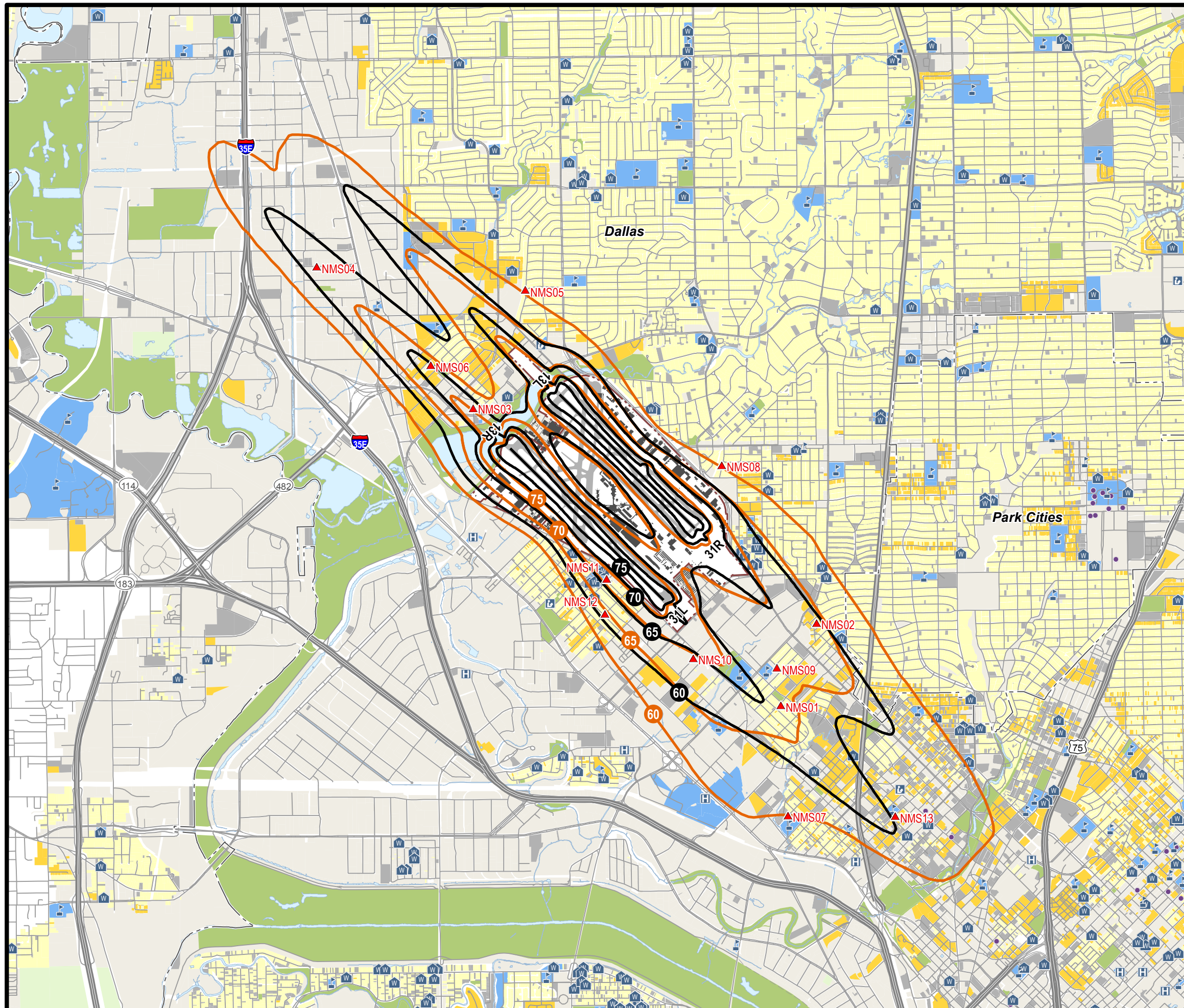
Figure 17 2013 DNL Contours compared to 2006 DNL Contours
