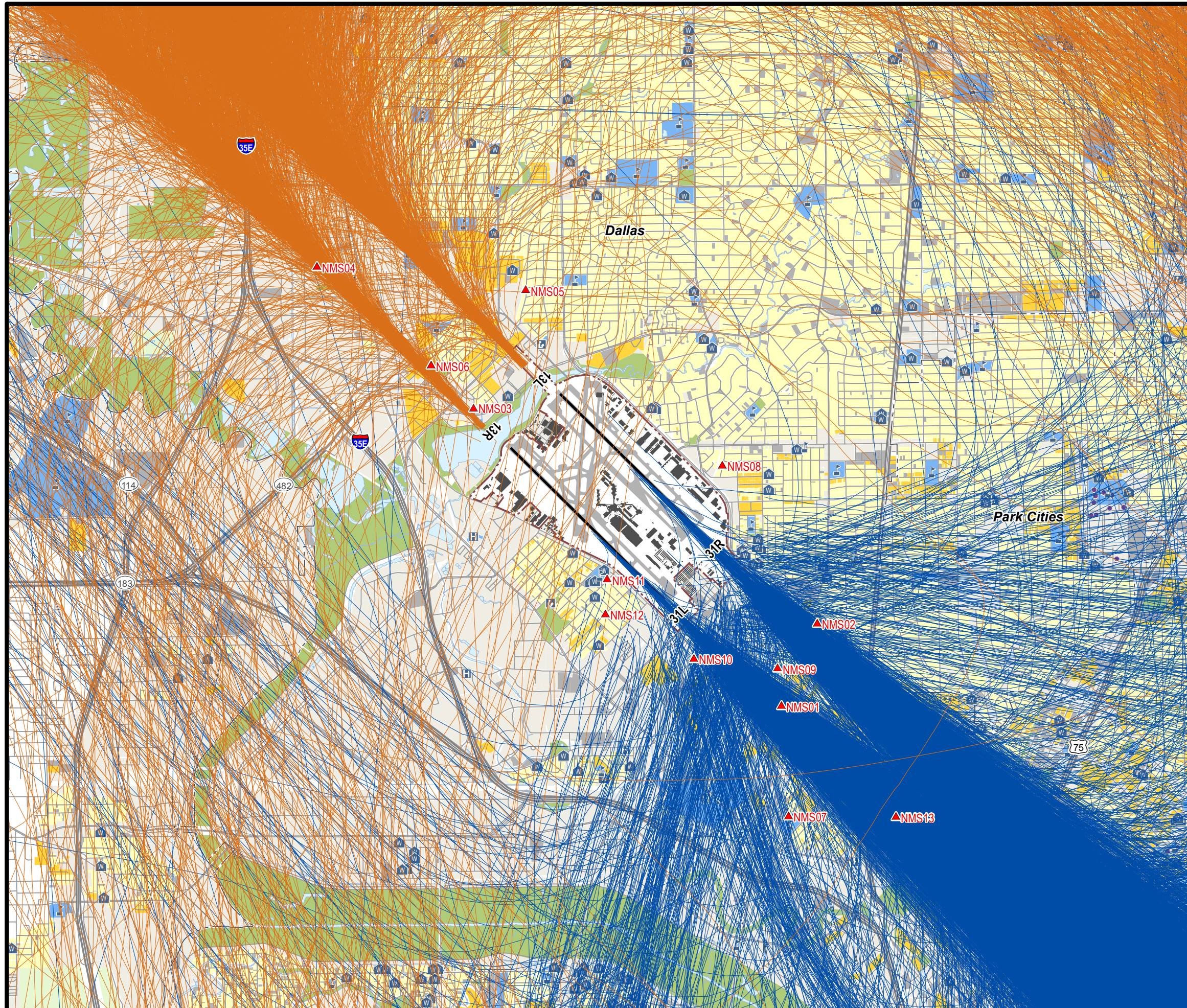
Figure 14 Sample of Modeled South Flow Flight Tracks
