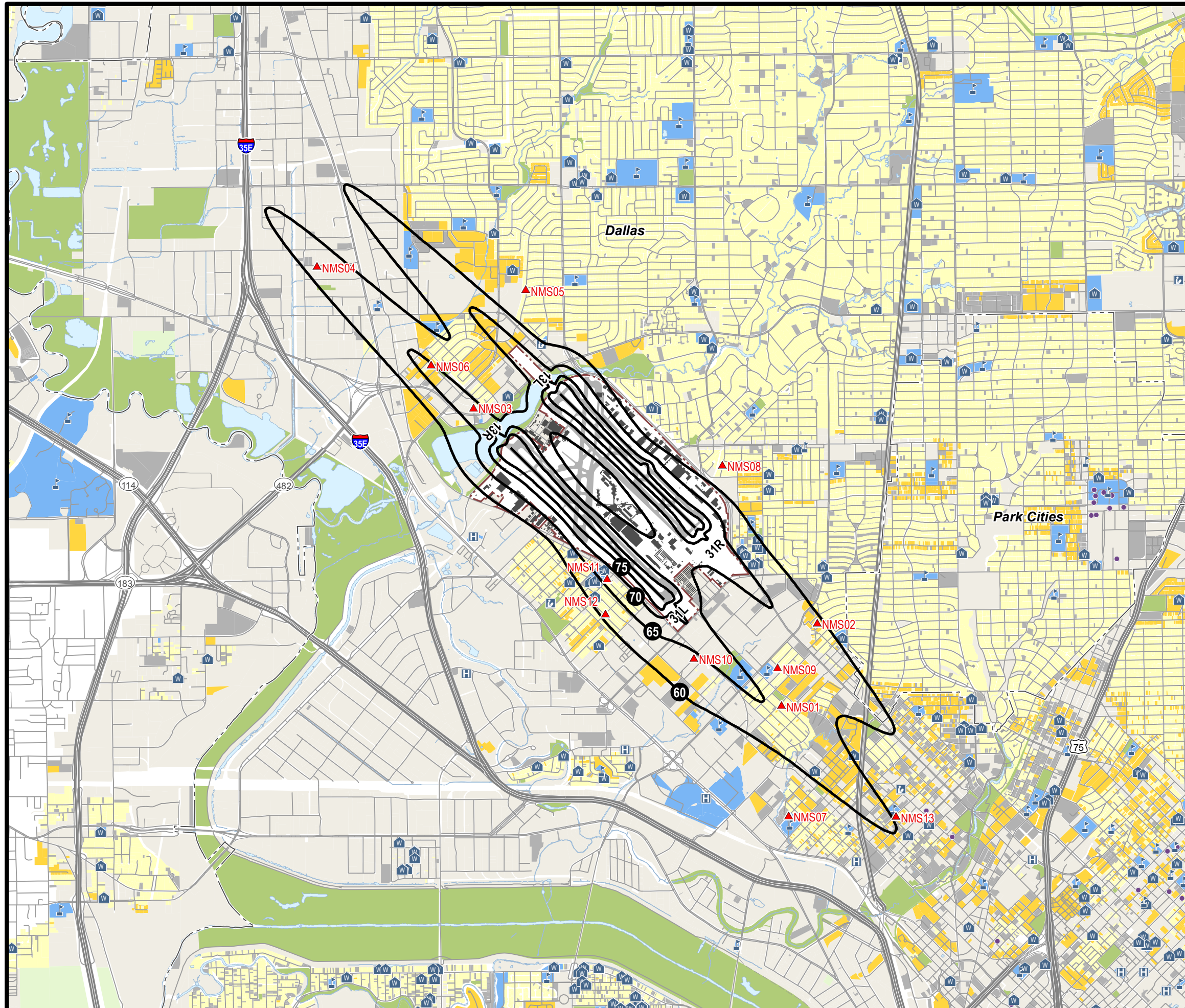
Figure 16 2013 DNL Contours
