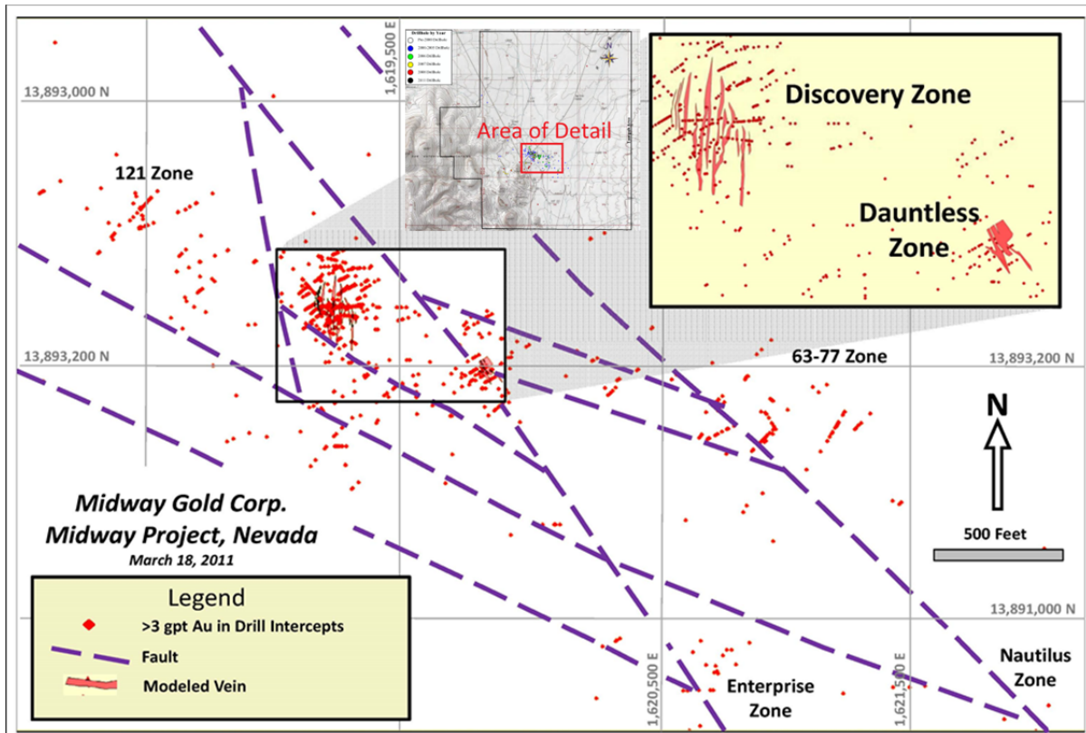
Figure 7-6 Tonopah High Grade Gold Intercept Distribution (Plan View)
