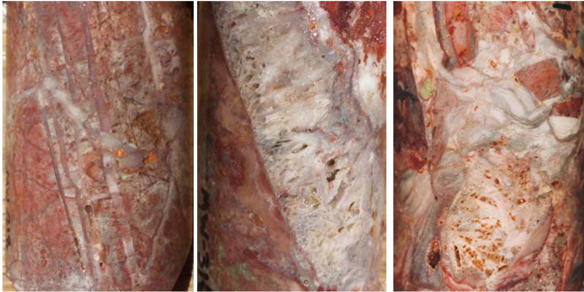
Figure 7-7 Core Photos of Tonopah Vein Structures
