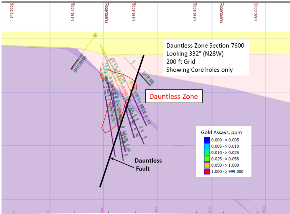
Figure 7-11: Cross Section showing Dauntless Zone Mineralization (Section 7600 from Figure 7-4) (Podratz & LeLacheur, 2014)
