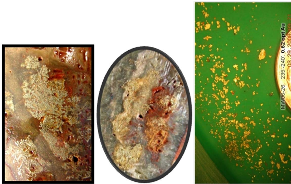
Figure 7-8 Visible Gold from Tonopah Project
