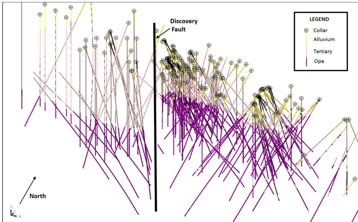
Figure 7-5 Oblique Cross Section of the Discovery Zone showing offset of Trv/Opa contact in drilling (Podratz & LeLacheur, 2014)
