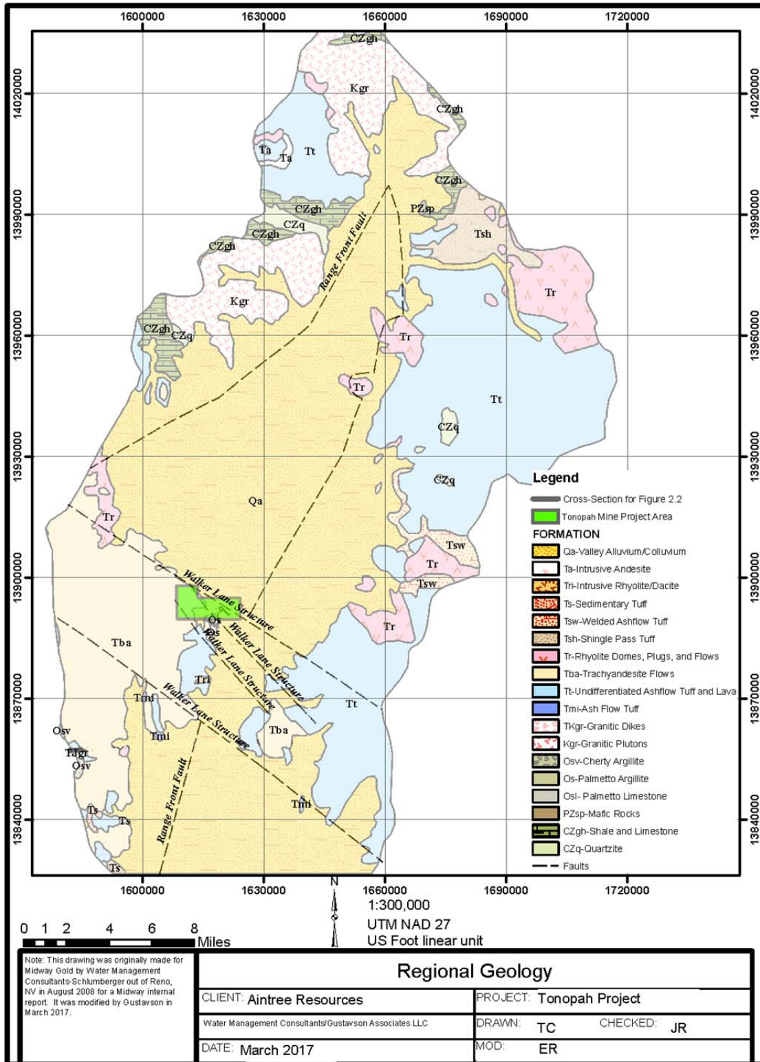
Figure 7-1 Regional Geology
