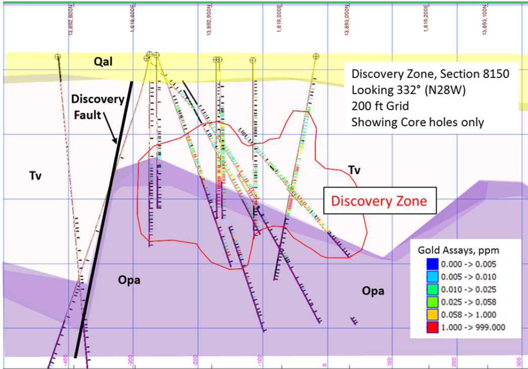
Figure 7-9: Cross Section through Discovery Zone (Section 8150 from Figure 7-4) (Podratz & LeLacheur, 2014)
