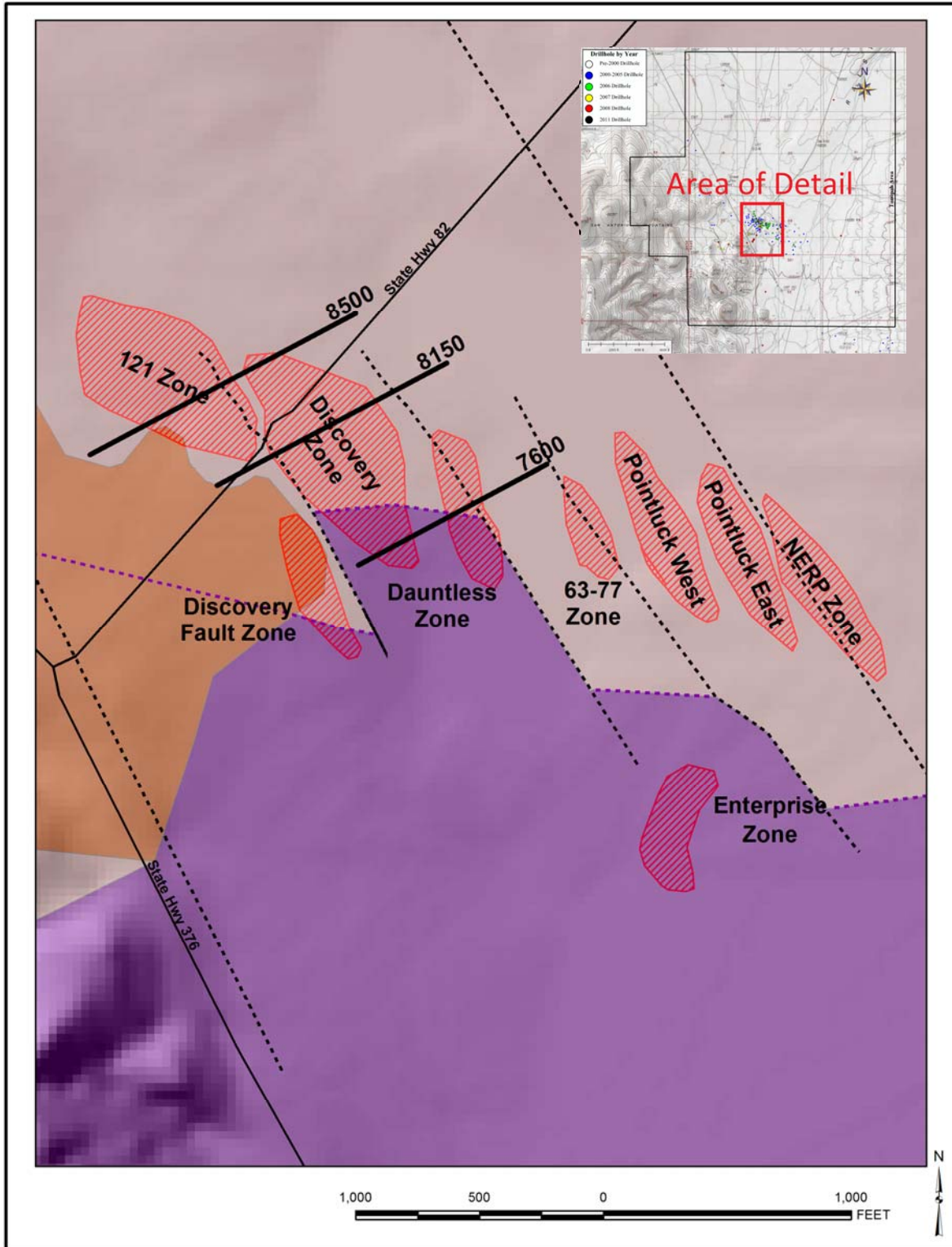
Figure 7-4 Mineralized Zones at the Tonopah project, and cross section traces for Section Lines. Section 8500 corresponds to Figure 7-10. Section 8150 corresponds to Figure 7-9. Section 7600 corresponds to Figure 7-11. (Podratz & LeLacheur, 2014)
