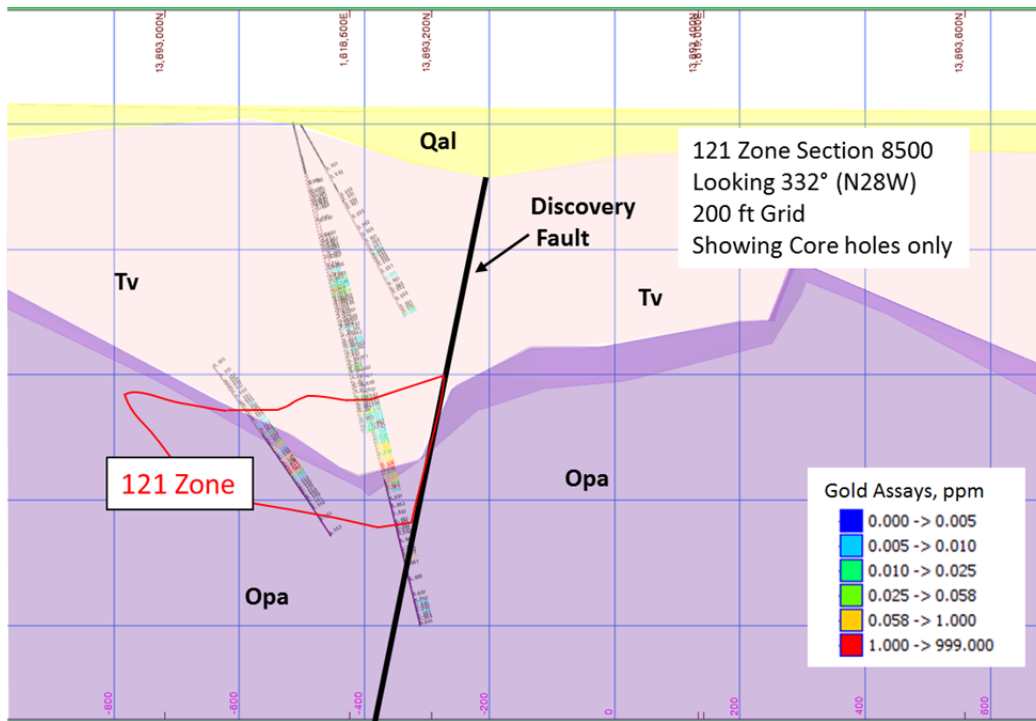
Figure 7-10: Cross Section through 121 zone Mineralization (Section 8500 from Figure 7-4) (Podratz & LeLacheur, 2014)
