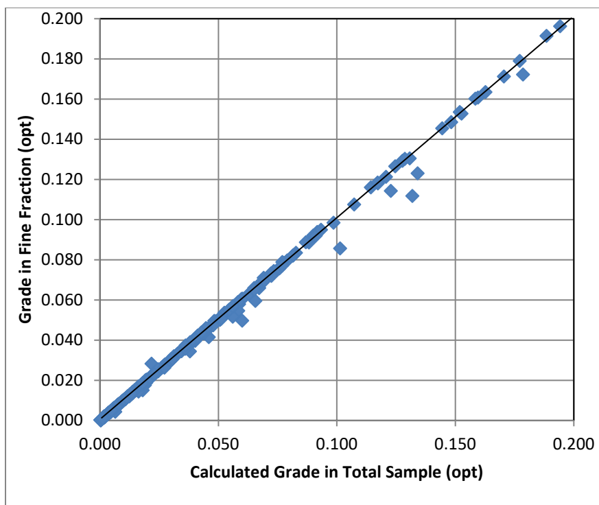
Figure 11-2: Comparison of Gold in Fine Fraction to Gold in total Sample
