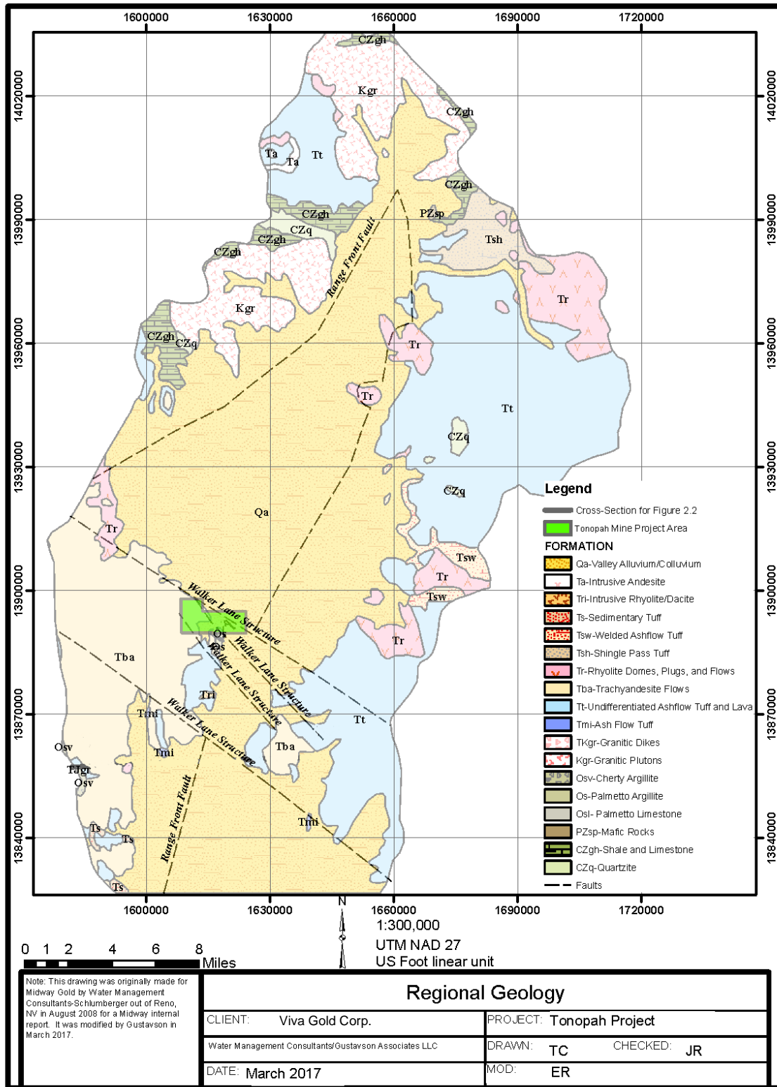
Figure 7-1: Regional Geology
