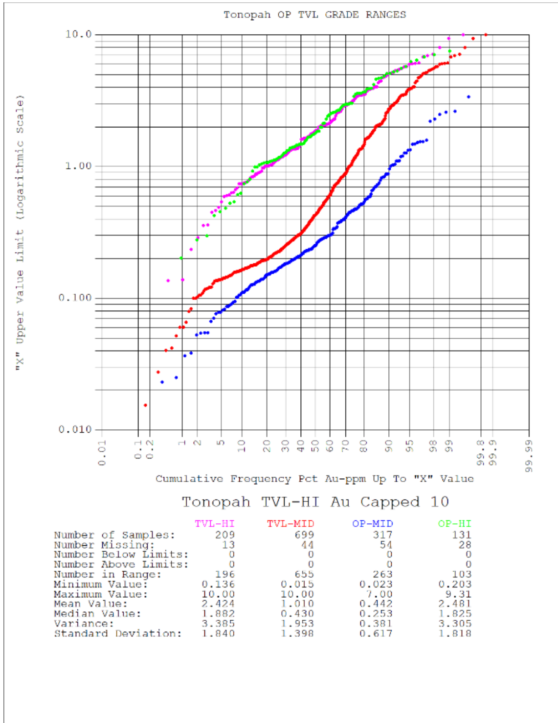
Figure 14-7: 0.15ppm and 0.8ppm domains for TVL and OP
