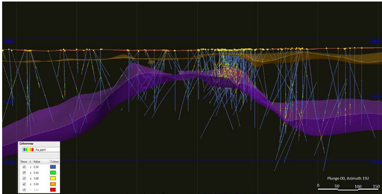
Figure 14-2: Long section view showing mineralization relative to Opa /Tv boundary surface. Az 192. Scale in meters.
