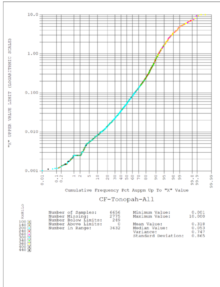
Figure 14-6: Global Cumulative Frequency Curve
