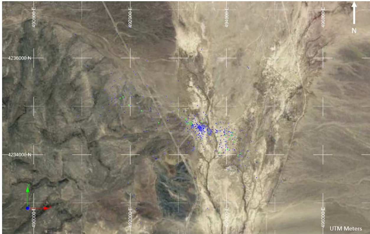
Figure 10-2: Plan view of drilling
