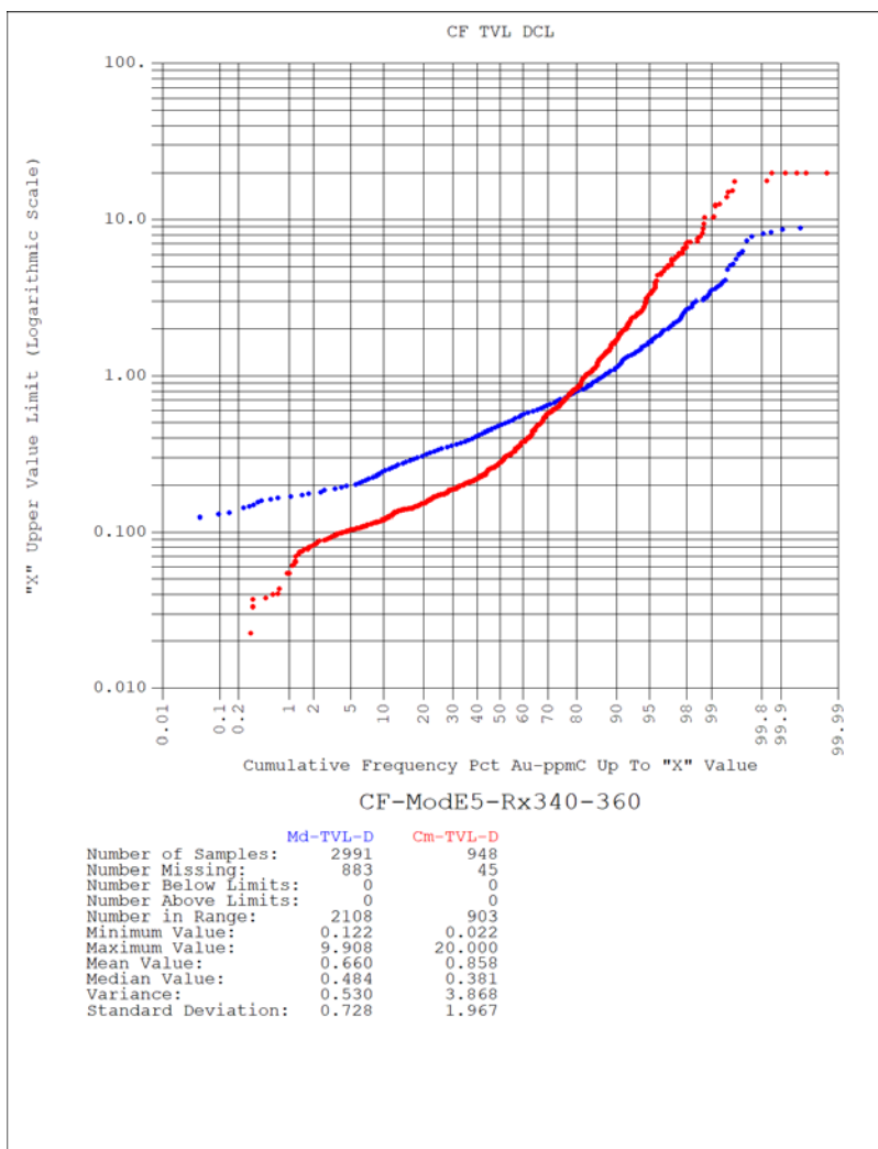
Figure 14-13: TVL Composites and Block grades, CFP Comparison.
