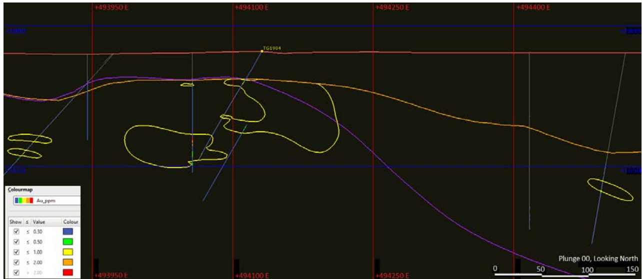
Figure 10-8: Cross Section showing Nautilus/Rye Patch Zone Mineralization with 2018-2019 drilling (Section E-E' from Figure 10-3)
