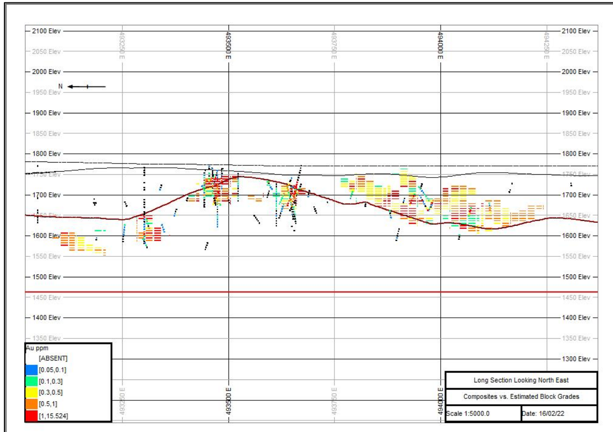
Figure 14-11: Example Cross Section (Looking NE) through Tonopah block model
