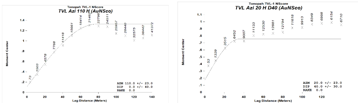
Figure 14-8: Normal Scores Variograms of TVL
