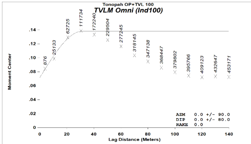
Figure 14-10: Variogram of 1.0ppm Indicator
