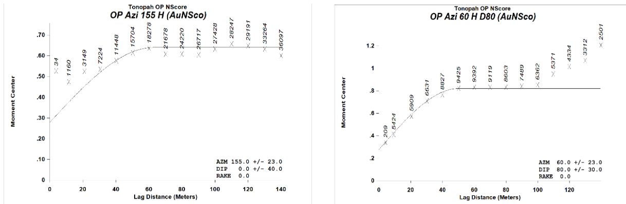
Figure 14-9: Normal Scores Variograms for OPA
