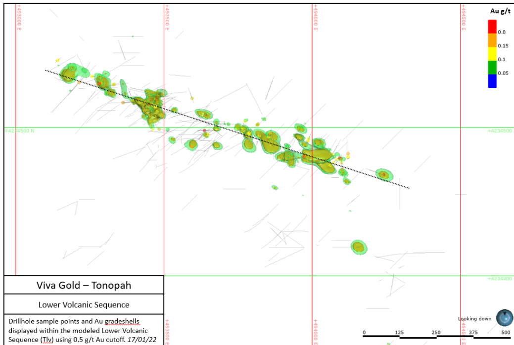
Figure 14-4: Lower Volcanic Composites >0.5ppm
