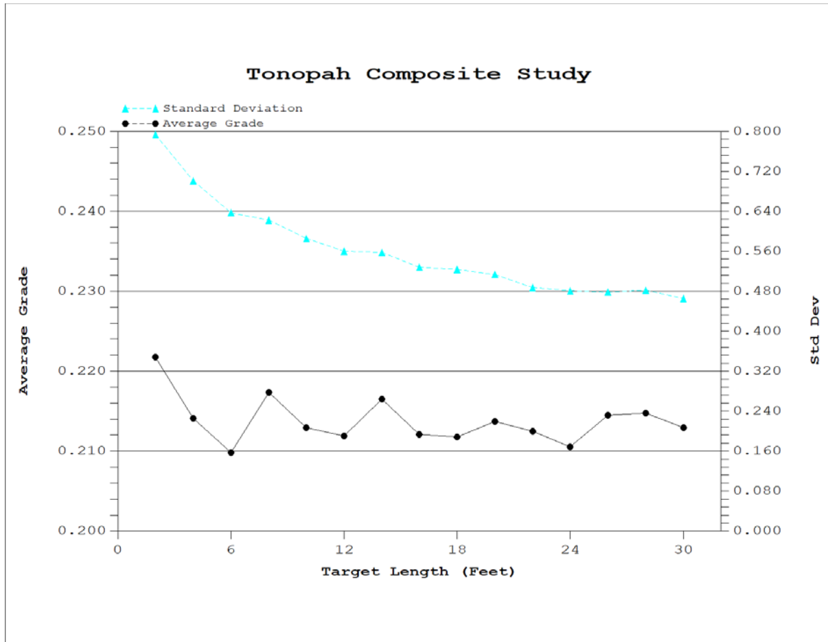
Figure 14-5: Drill Hole Composite Study
