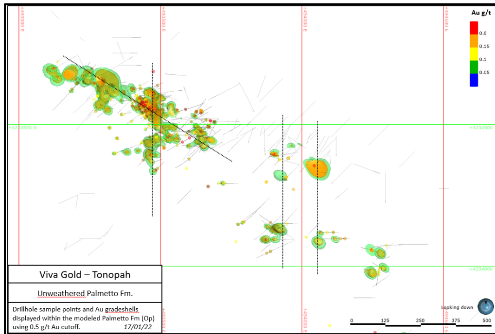
Figure 14-3: Palmetto Composites >0.5ppm
