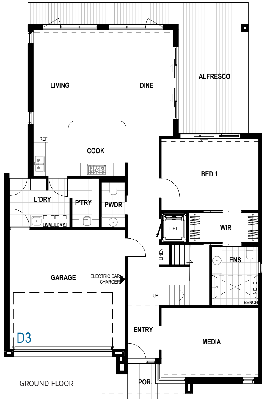
DWELLING 3 FLOOR PLAN
