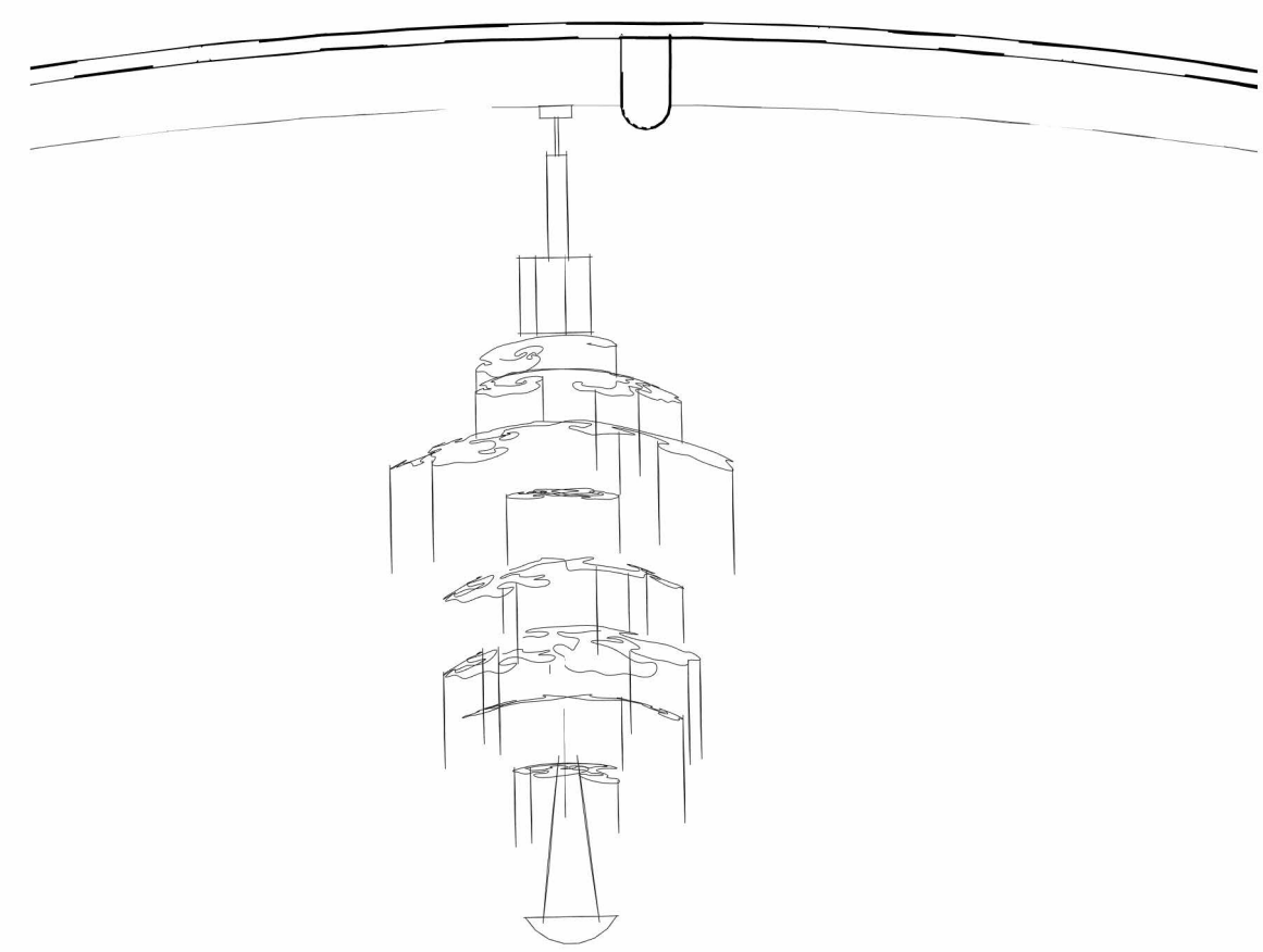
③ VIEW OF FARAWAY TREE 8-TIER CHANDELIER 1/2" = 1'-0"
