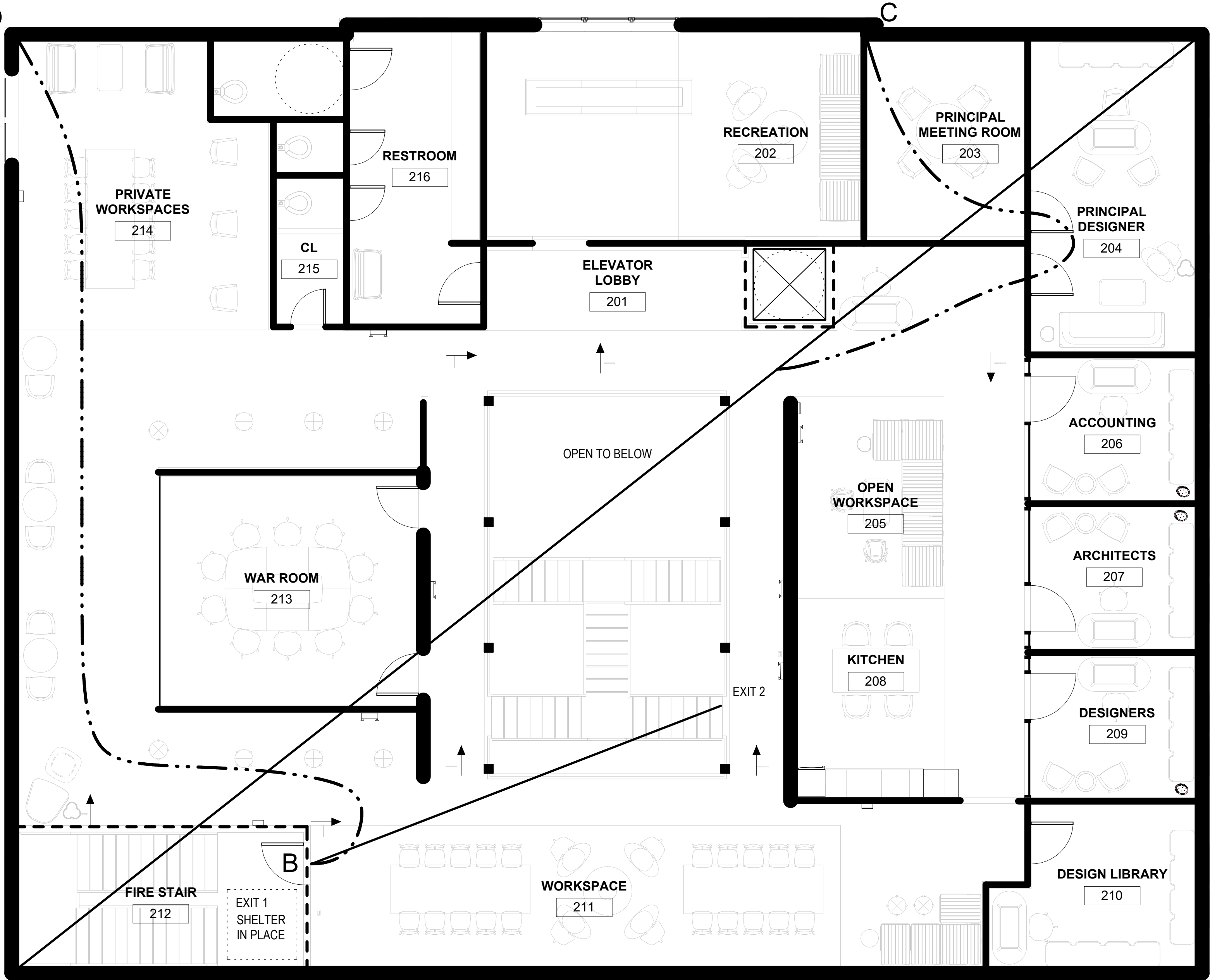
2 LIFE SAFETY PLAN - 2ND FLR. 3/16" = 1'-0"
