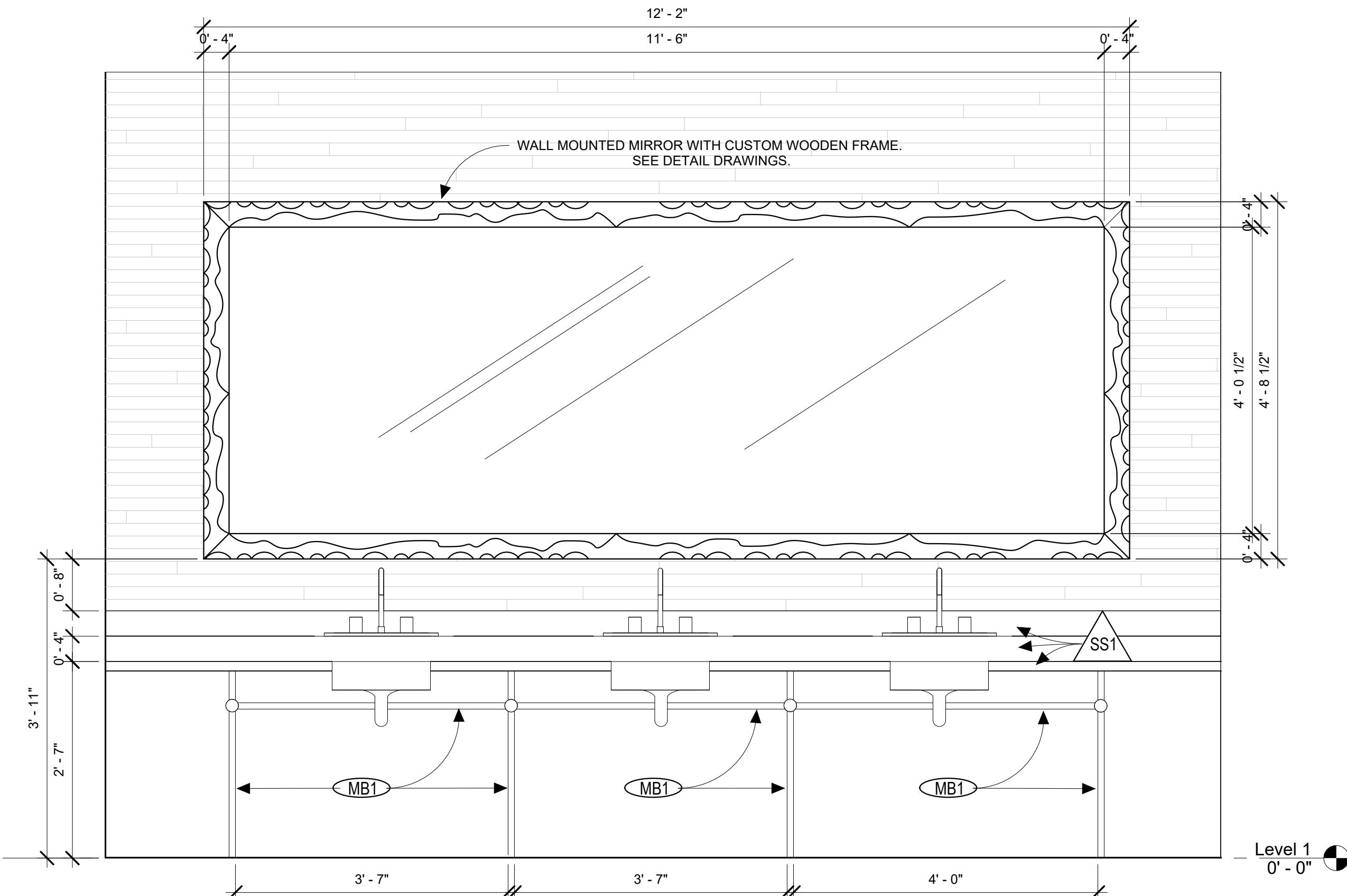
ELEVATION OF FIRST FLOOR RESTROOM VANITIES 3/4" = 1'-0"
