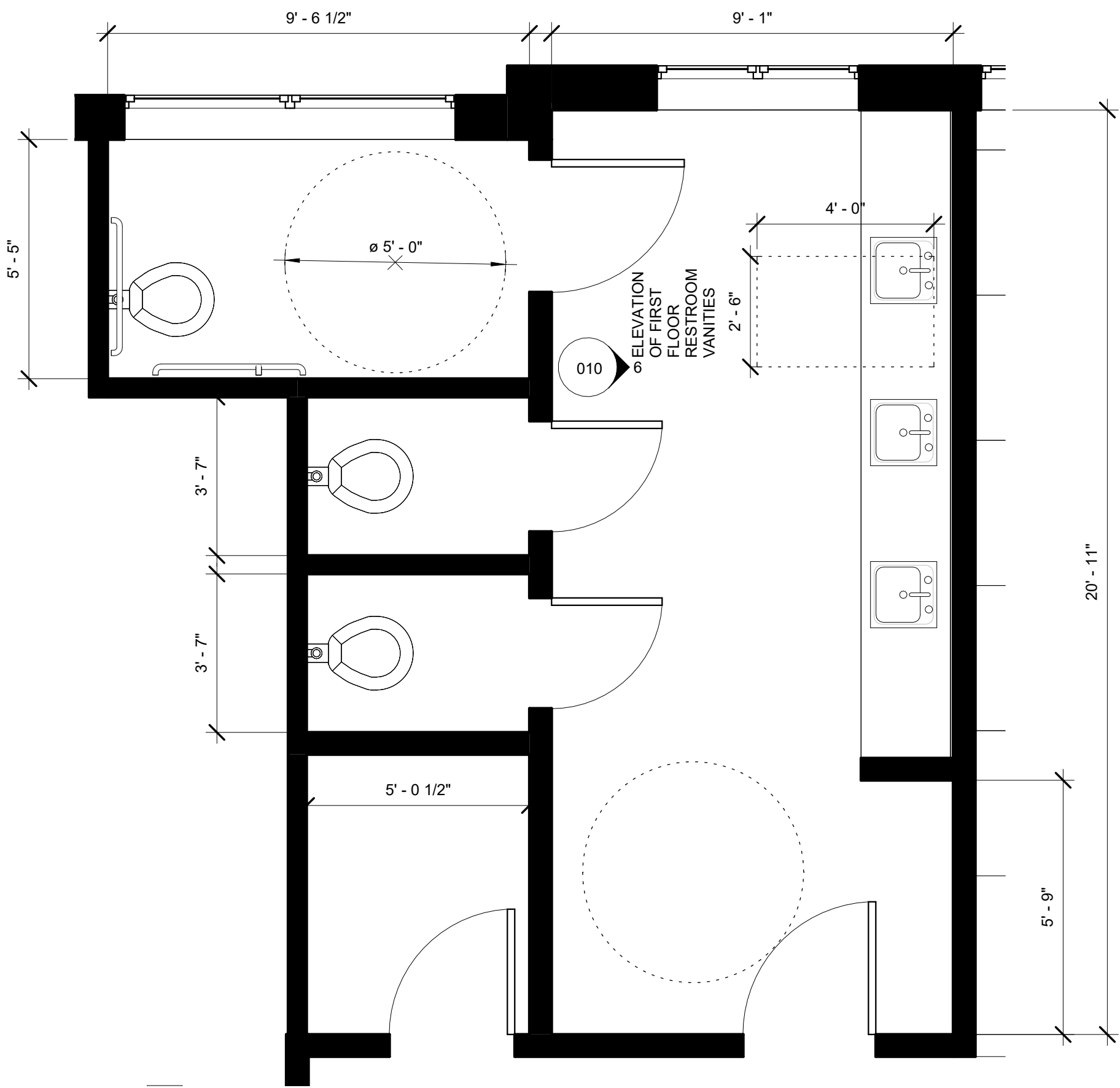
3 ADA COMPLIANT SHARED GENDER NEUTRAL RESTROOM 3/16" = 1'-0"
