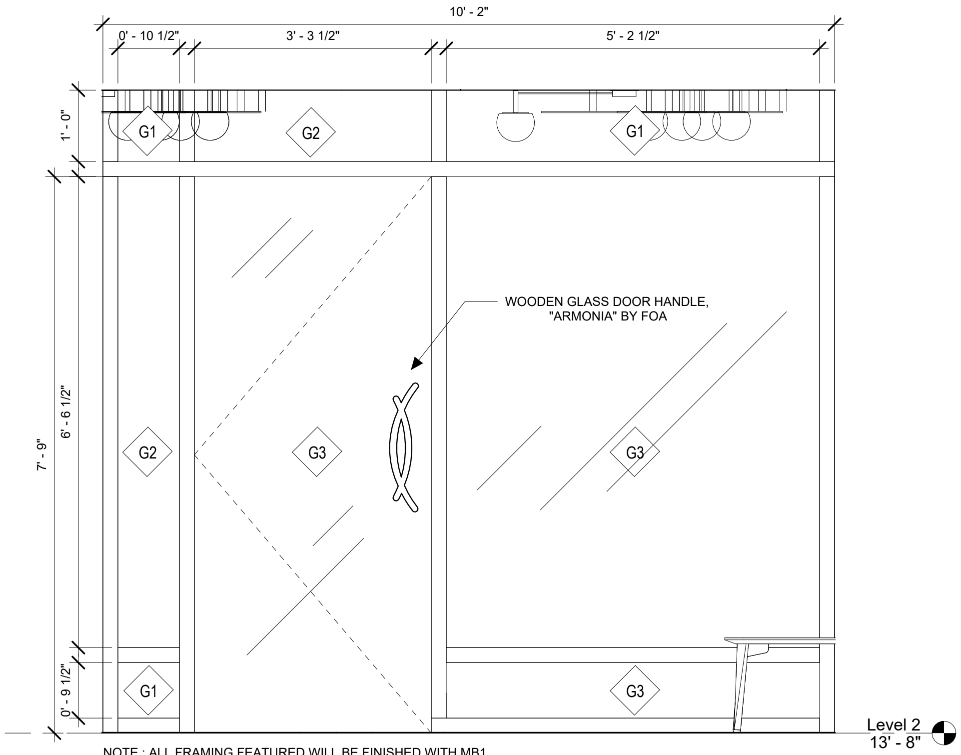
ELEVATION OF GLASS OFFICE PARTITION WALL 3/4" = 1'-0"
