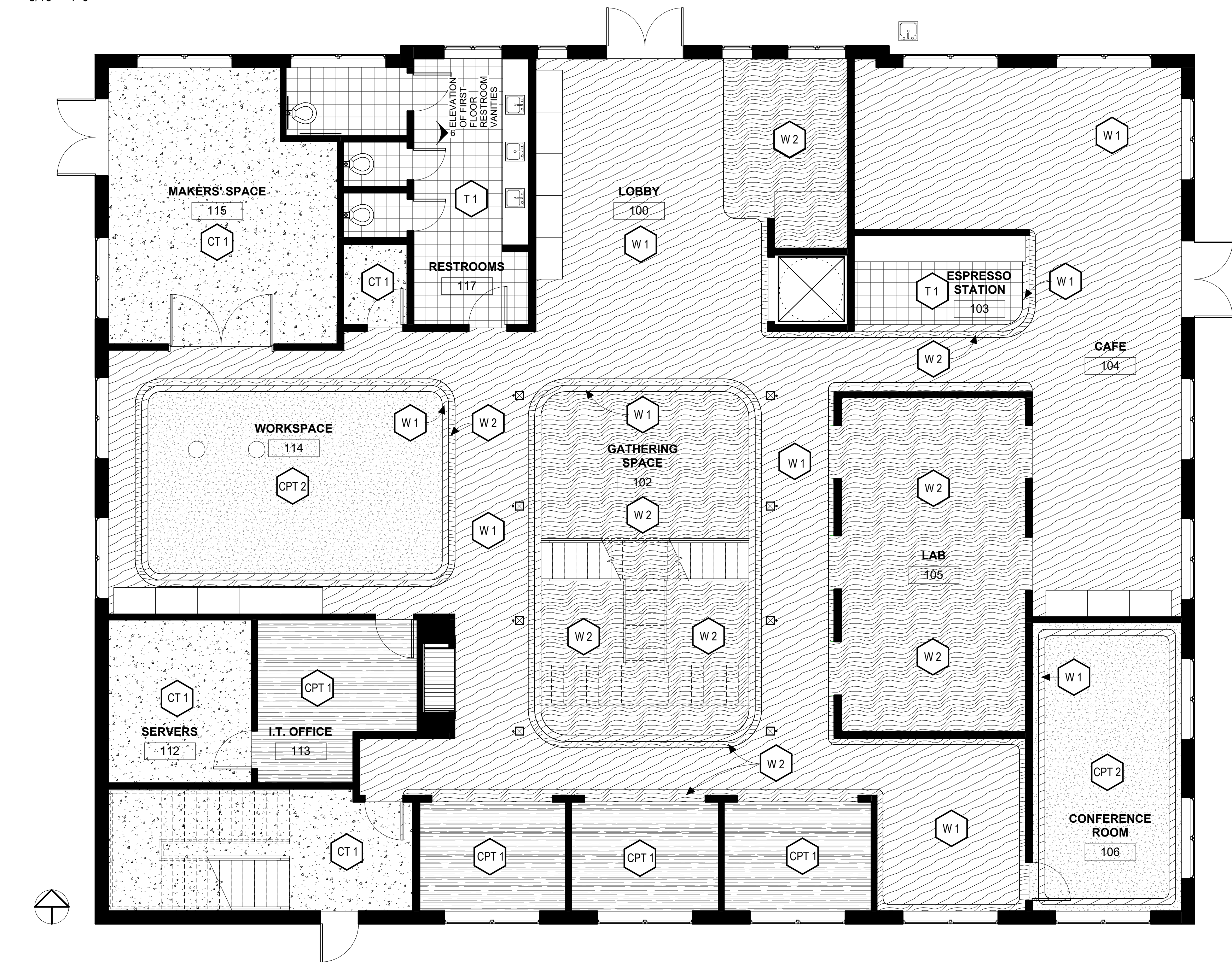
1 FINISH PLAN - 1ST FLR 3/16" = 1'-0"
