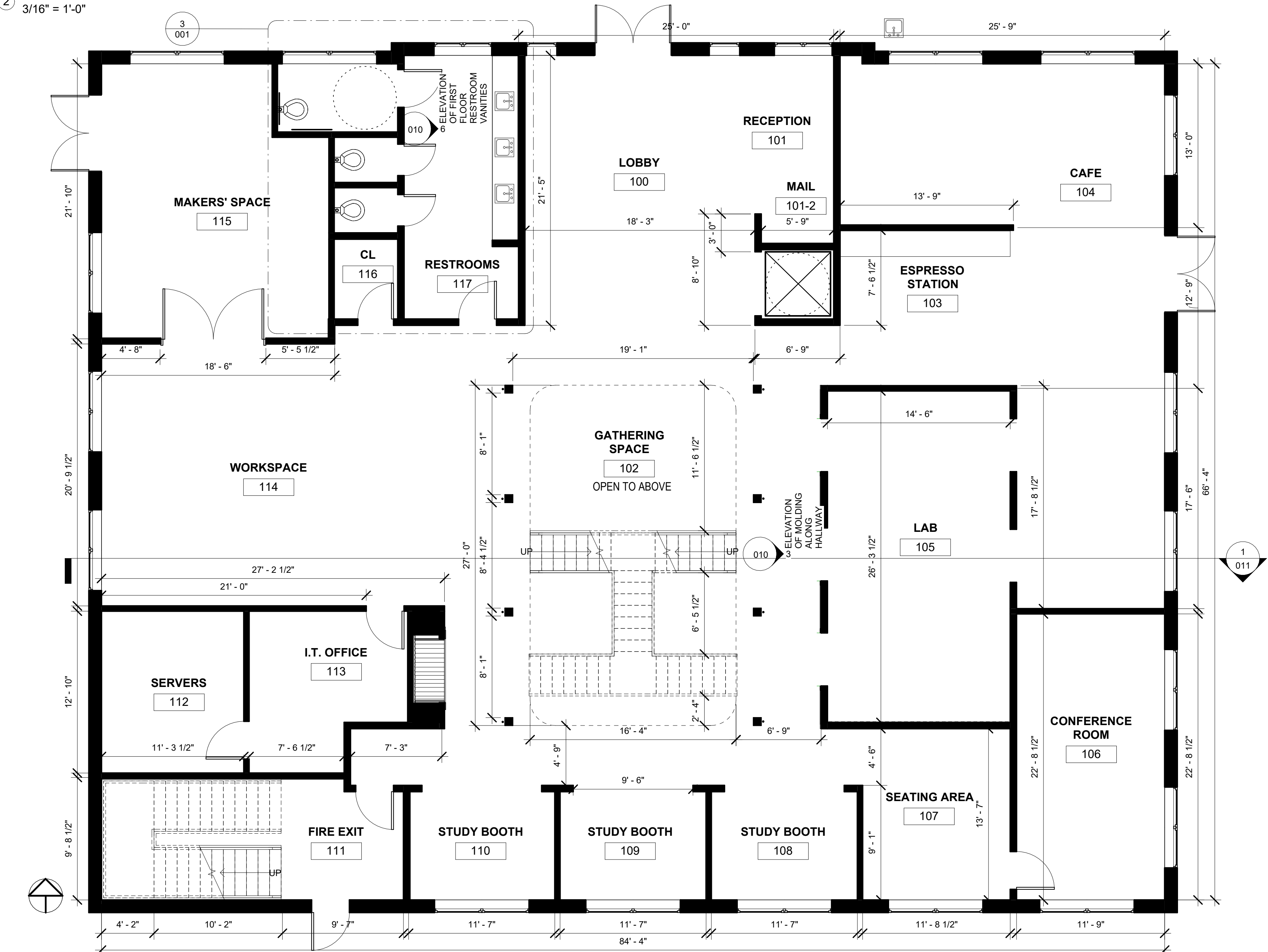
1 FLOOR PLAN - 1ST FLR 3/16" = 1'-0"
