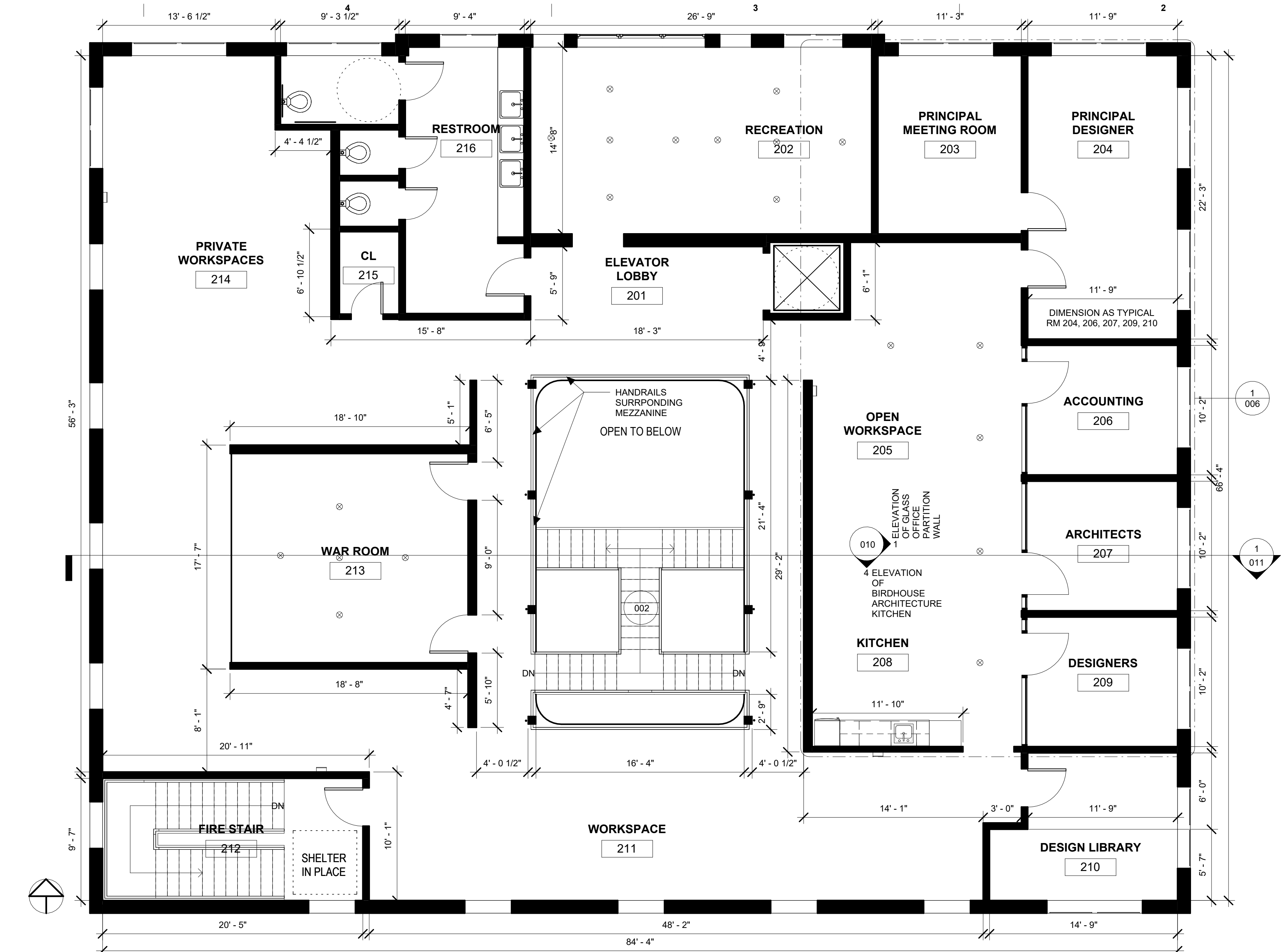
2 FLOOR PLAN - 2ND FLR 3/16" = 1'-0"
