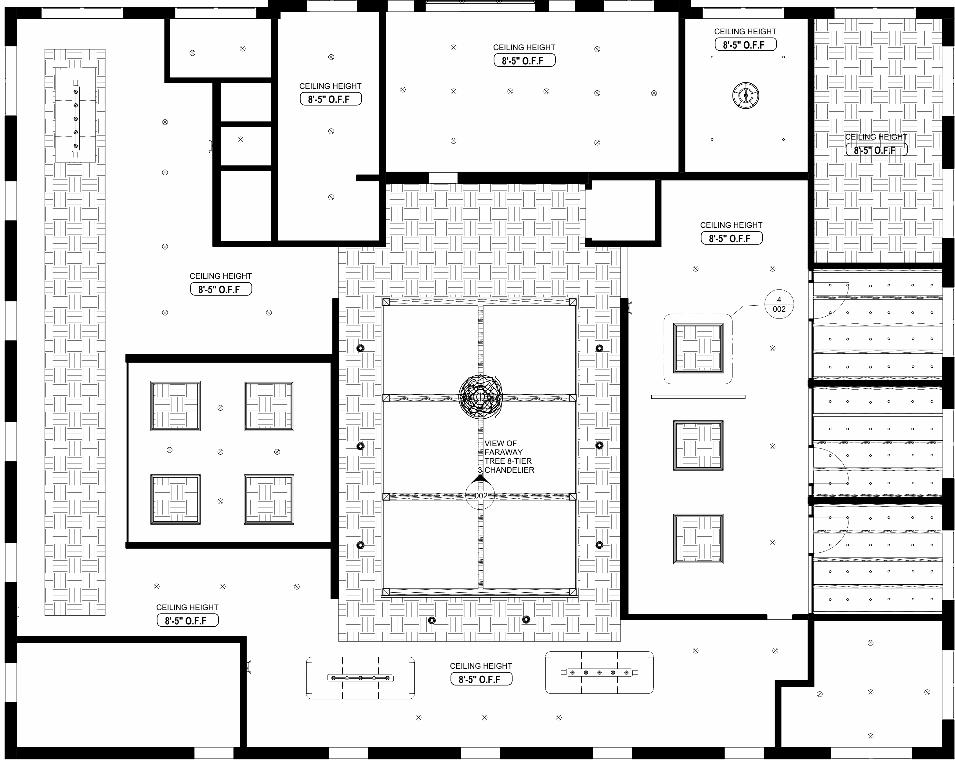
② RCP LEVEL 2 3/16" = 1'-0"
