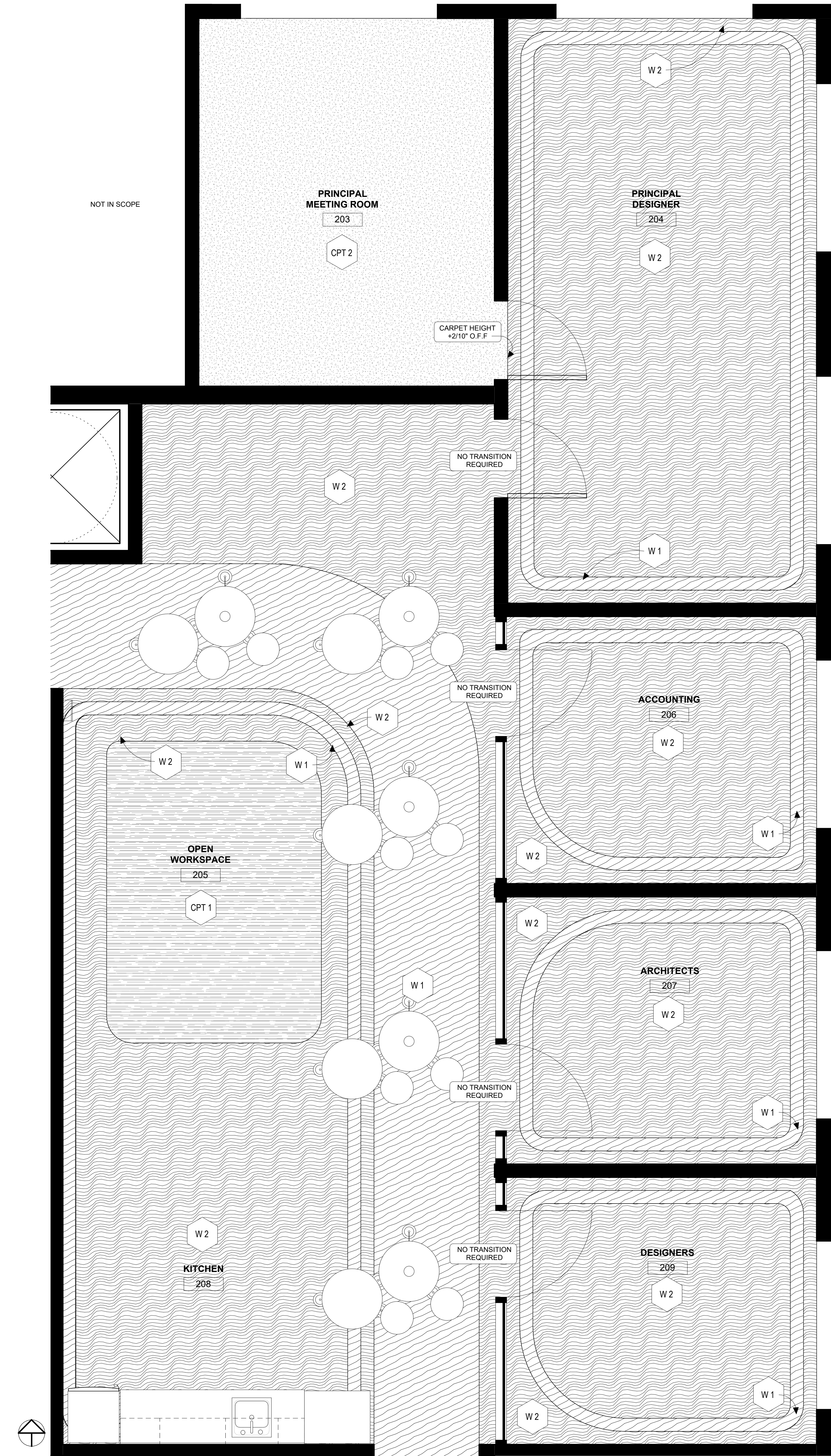
LEVEL 2 BIRDBHOUSE ARCHITECTURE FLOOR FINISH PLAN 1/2" = 1'-0"
