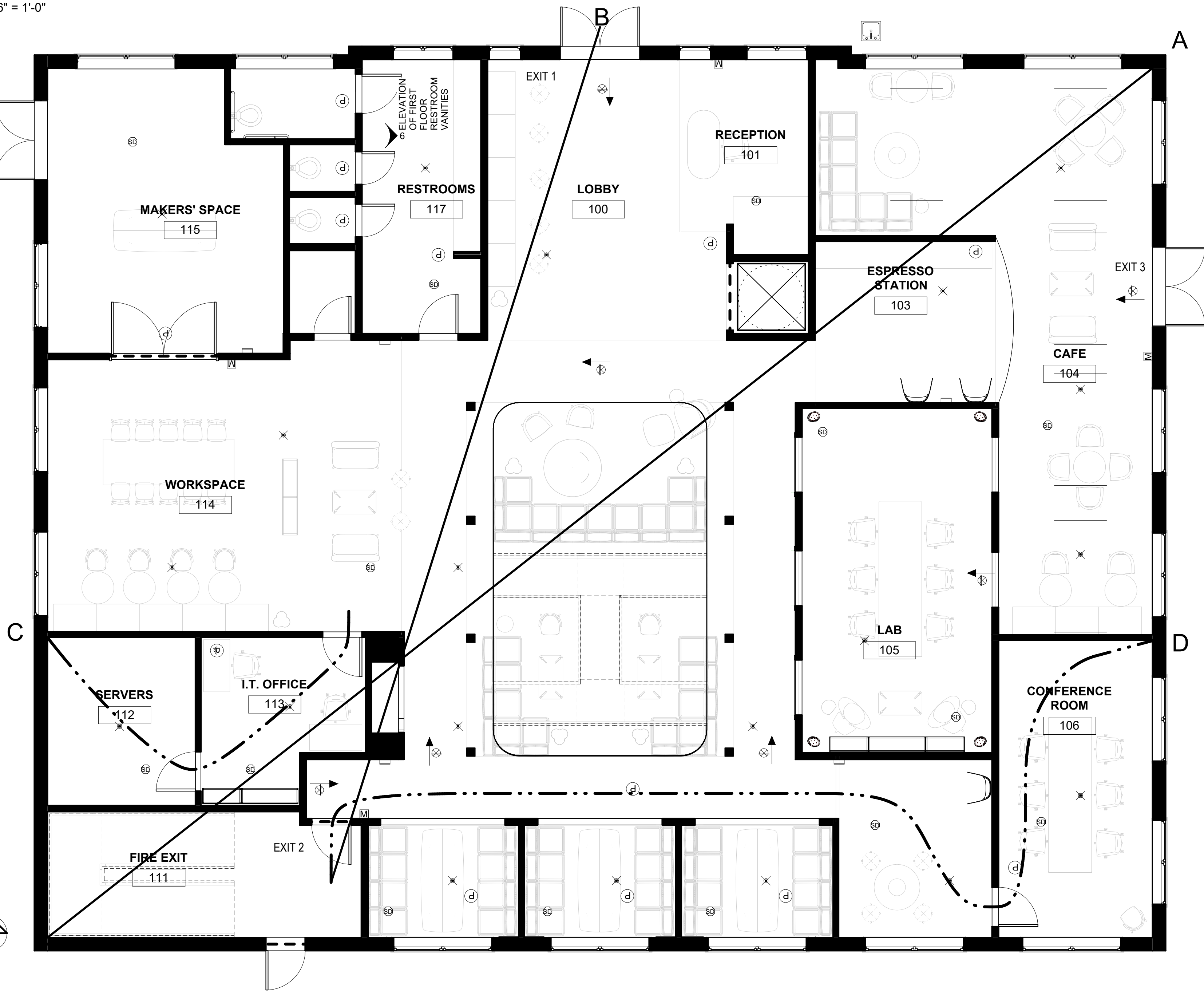
1 LIFE SAFETY PLAN - 1ST FLR. 3/16" = 1'-0"
