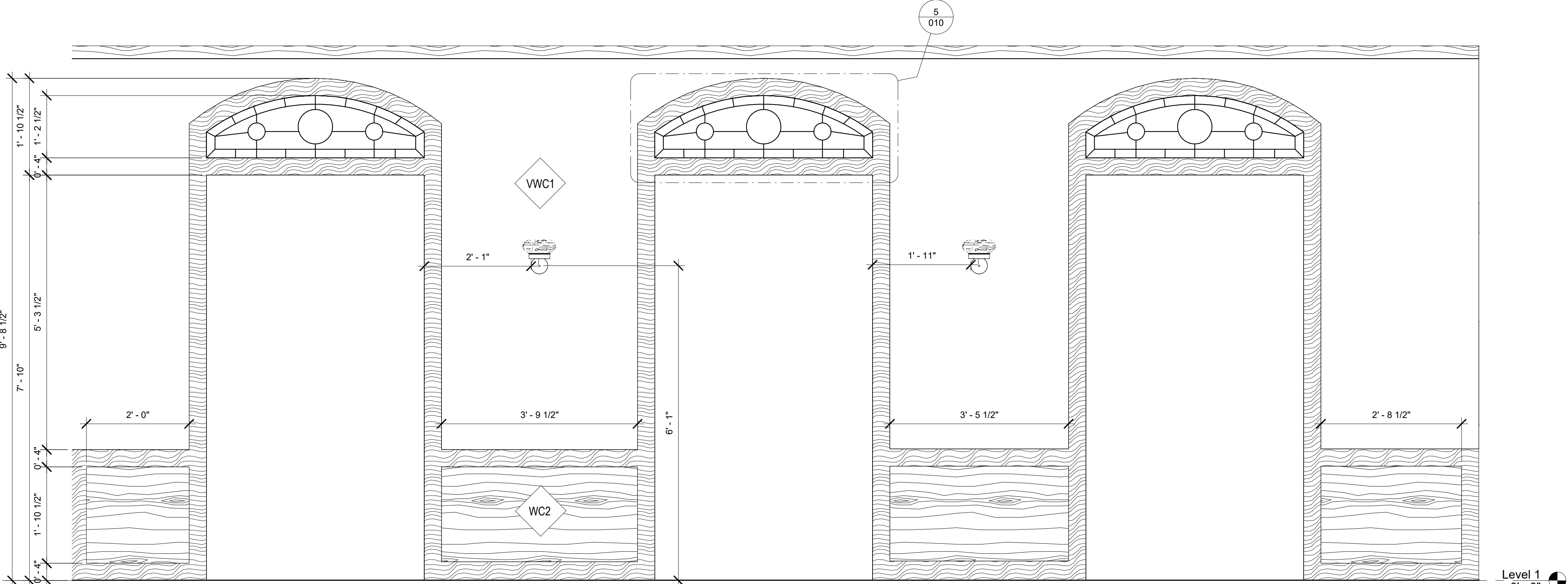
ELEVATION OF MOLDING ALONG HALLWAY 3/4" = 1'-0"
