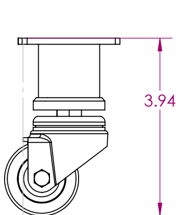
FULLY RETRACTED
