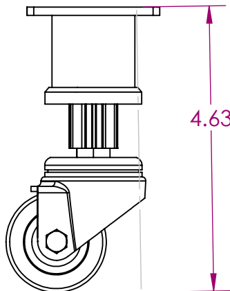
FULLY EXTENDED
