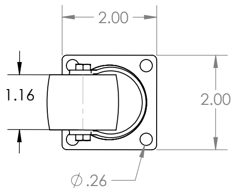
FULLY EXTENDED
