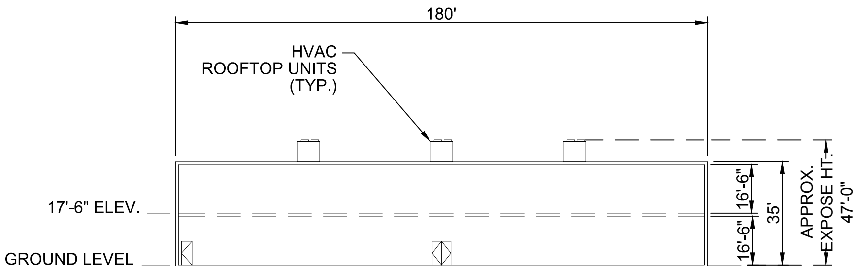
SECTION VIEW B-B (LOOKING NORTH) SCALE: 1/32" = 1'
