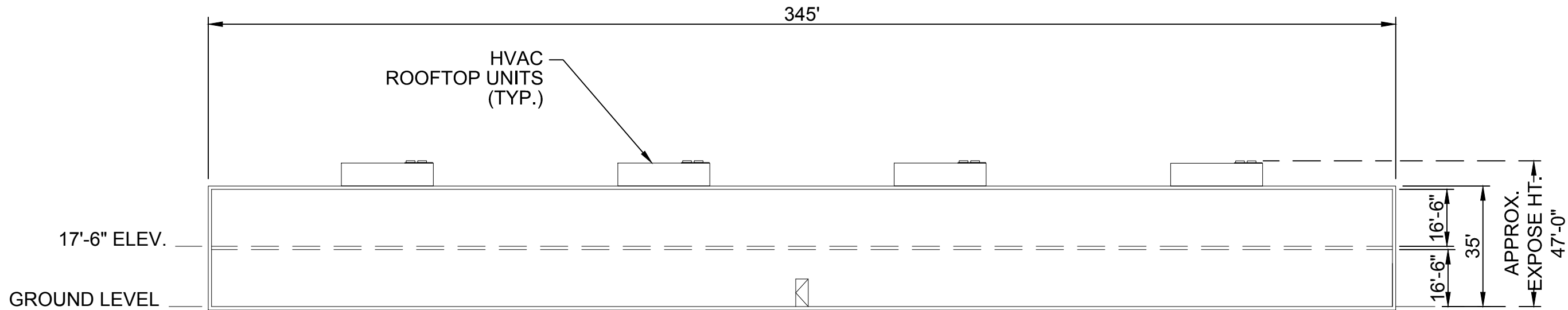
SECTION VIEW A-A & A'-A' (LOOKING WEST AND EAST) SCALE: 1/32" = 1'
