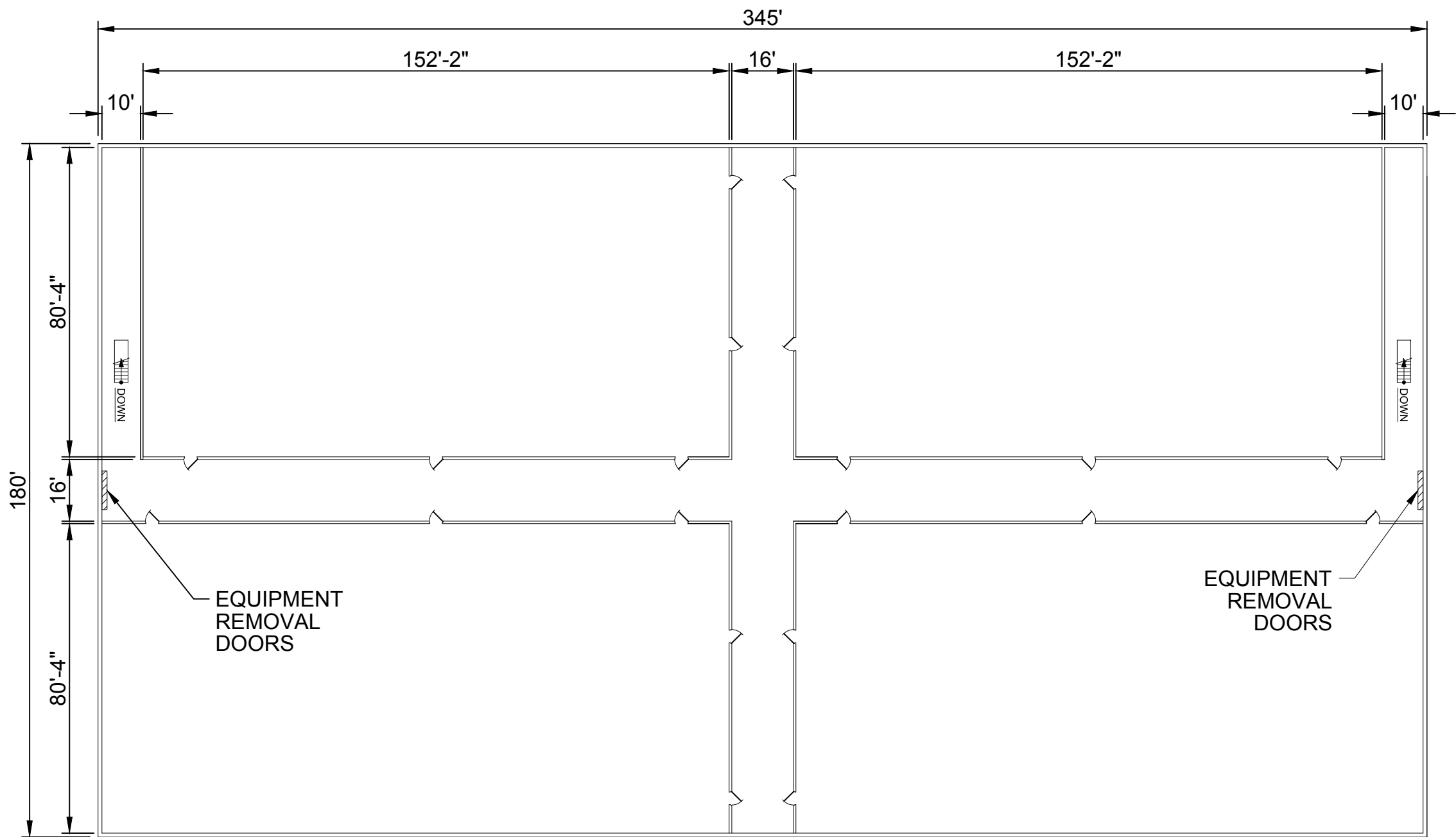
2ND FLOOR SCALE: 1/32" = 1'
