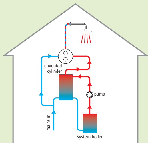
hot water cylinder installed in the airing cupboard
