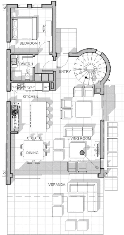
PRELIMINARY GROUND FLOOR
