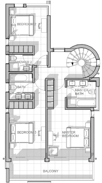
PRELIMINARY FIRST FLOOR
