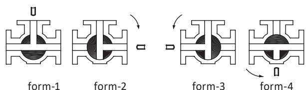
3-way T-Port
