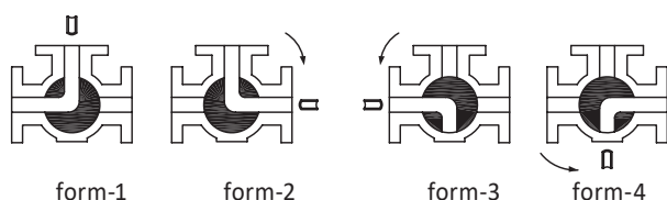
3-way L-Port
