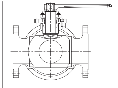
3-way T-Port
