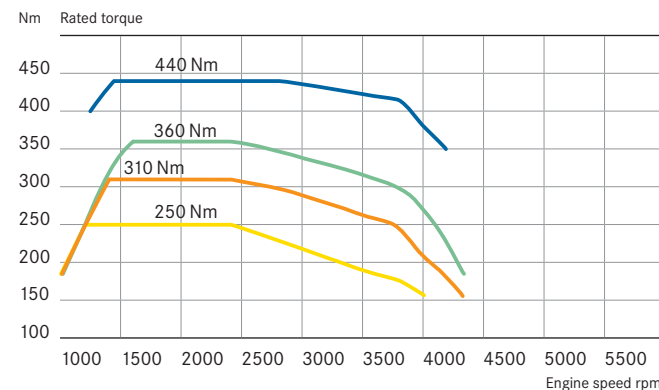
torque curves 1 :
