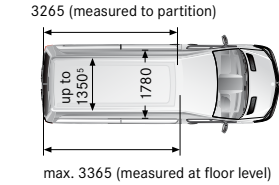
Medium with 3665 mm wheelbase, super-high roof
