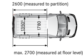
Short with 3250 mm wheelbase, high roof
