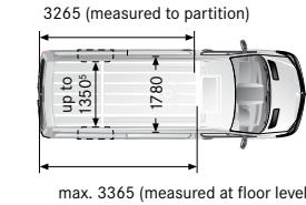
Medium with 3665 mm wheelbase, high roof
