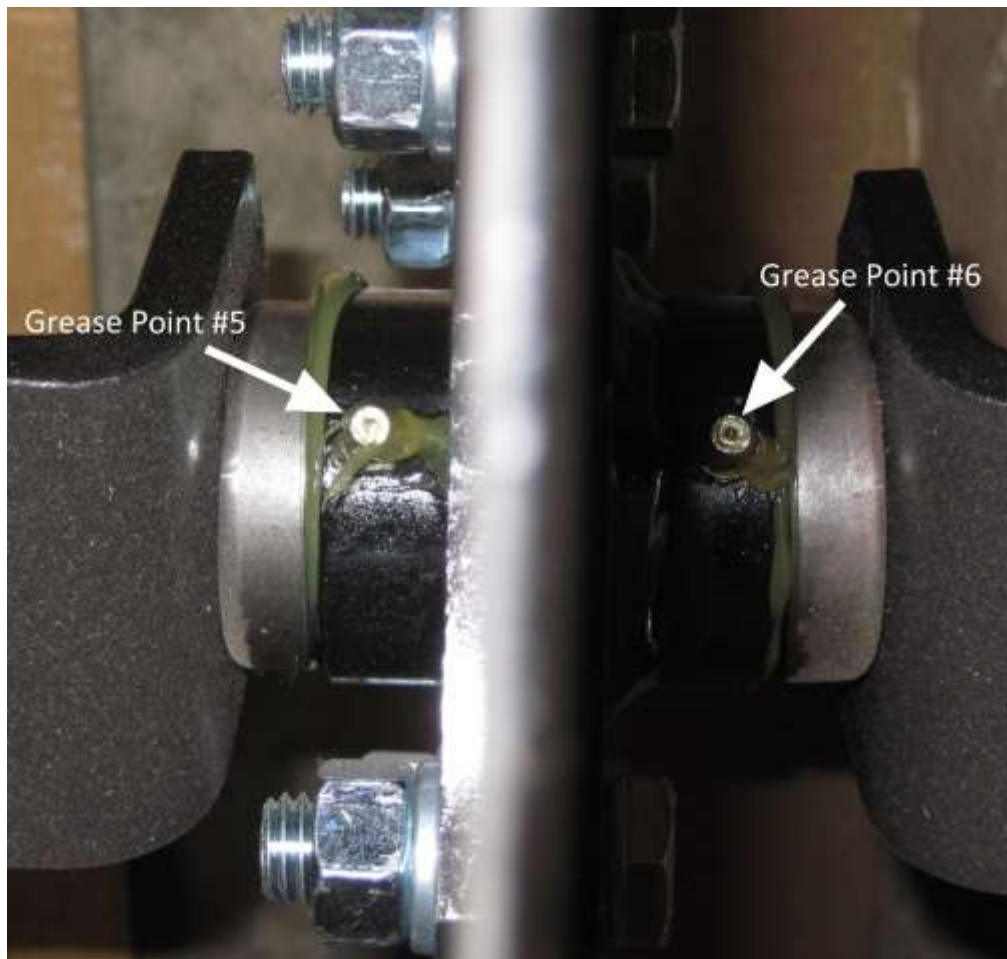
Figure 18: Coulter Hub Grease Points
