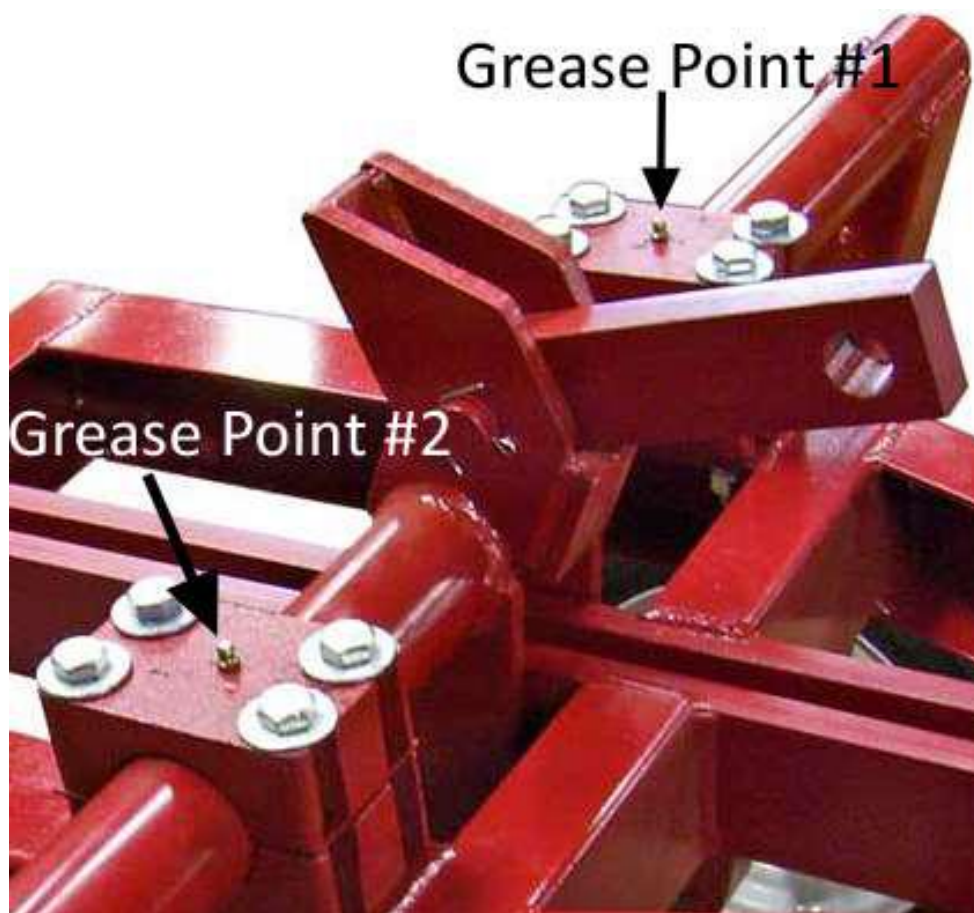
Figure 16: Packer Wheel Axle Grease Points
