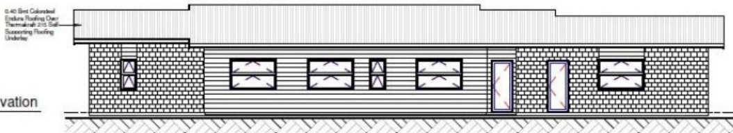
2 East Elevation 1:100
