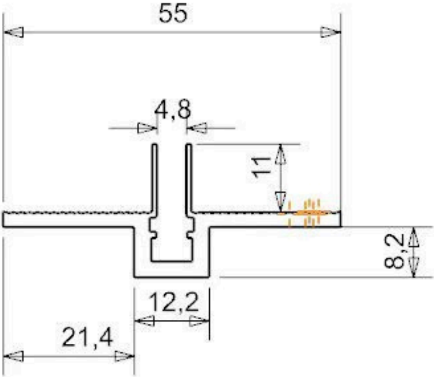
CONCEAL TRACK
