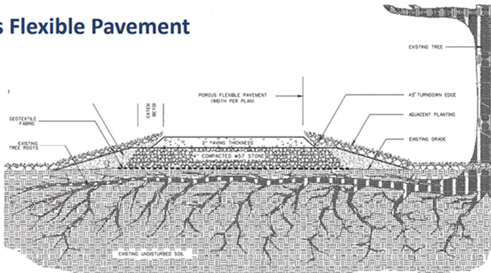
Cross section for Eastern Avenue NW: Metropolitan Branch Trail
