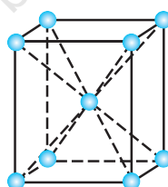
Body-centred
