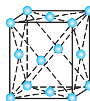
Face-centred
