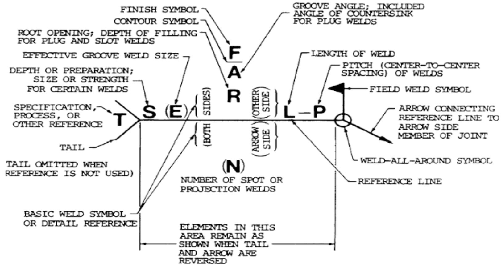
ELEMENTS OF WELDING SYMBOL
