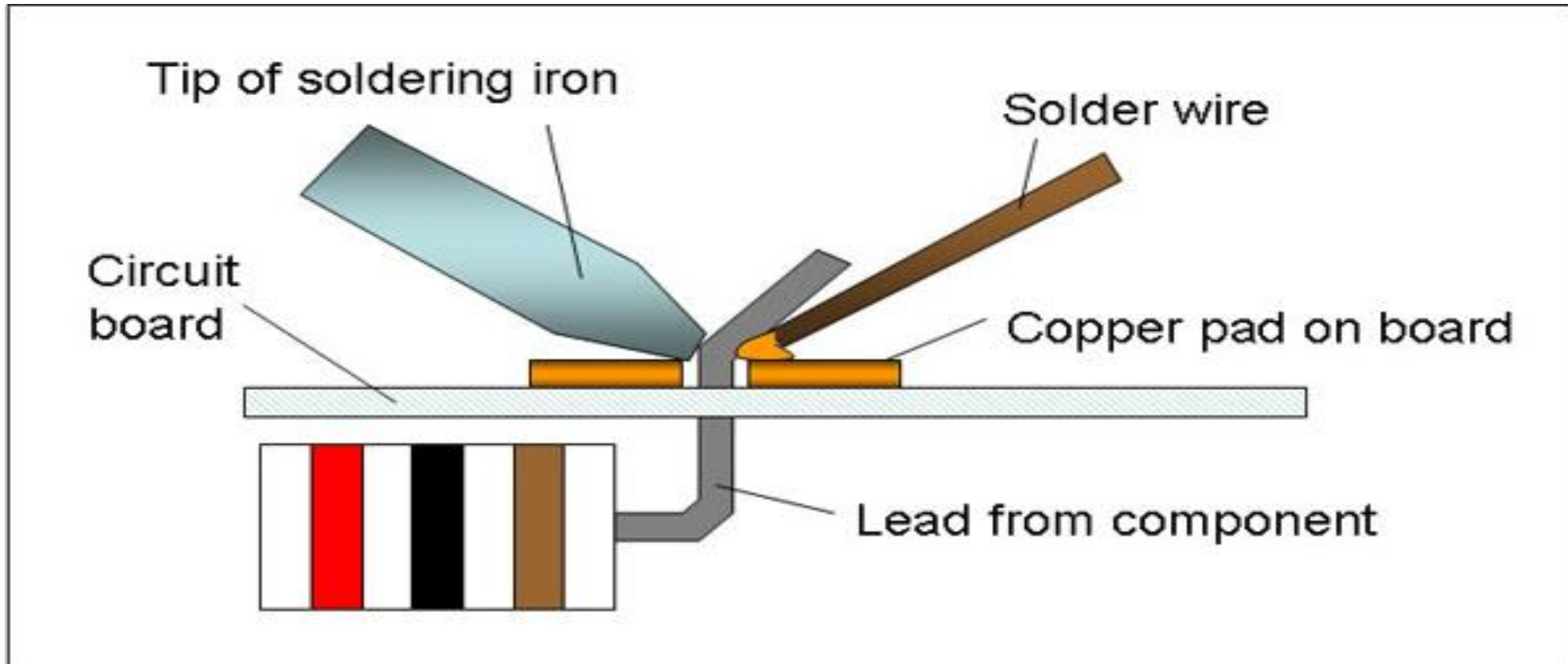
SOLDERING – SEMI PERMENANT METHOD
