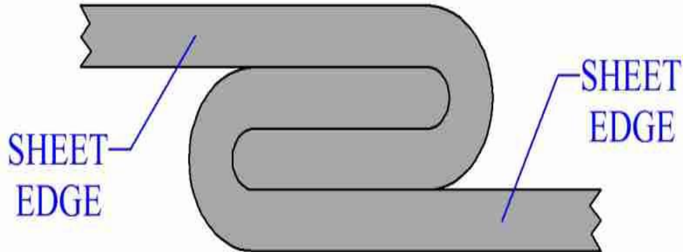
SEAMING – TEMPORARY METHOD
