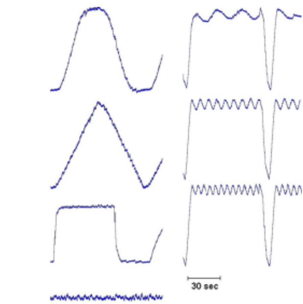
Figure 2: Various waveforms of distraction-forces applied via Accu-SPINA device (left panel). Low, medium and high frequency oscillations are presented in the right panel
