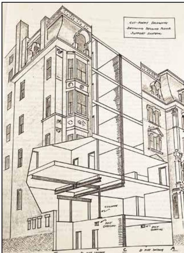
Cutaway Drawing of Second Floor Support System.
