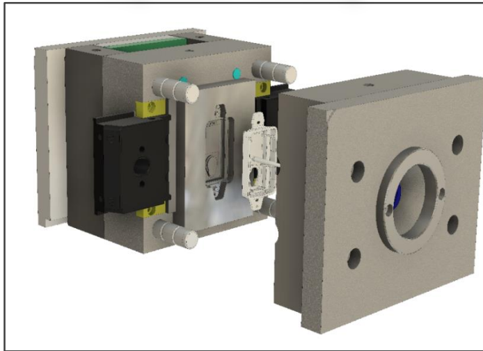
Injection Molding
