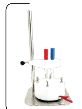
Bottom Mount Electro chemical Cell Setup
