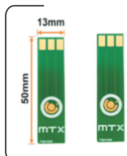
PCB Gold Electrode
