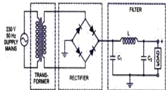
Block Diagram of an Unregulated Power Supply
