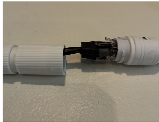
Make connection between the camera and CAT5
