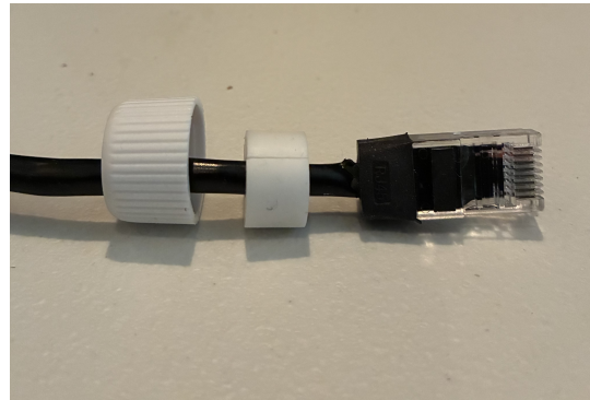
Add connector and split grommet on cable end
