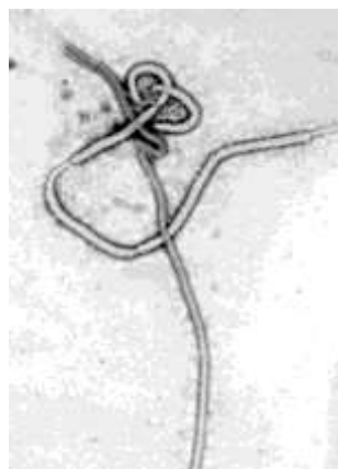
Ebola virus (source: Wikipedia)
